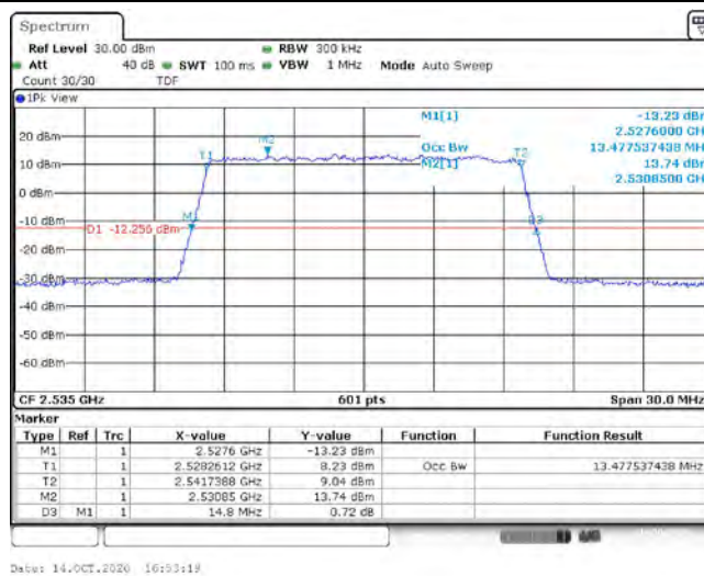
Band7-15MHz-16QAM-21375-75RB#0-13.478
