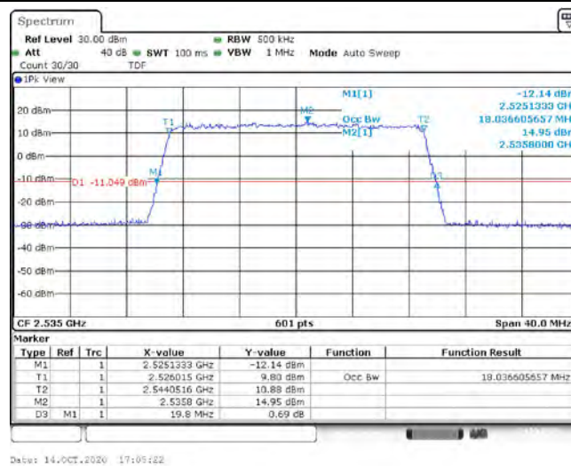
Band7-20MHz-16QAM-21350-100RB#0-17.97
