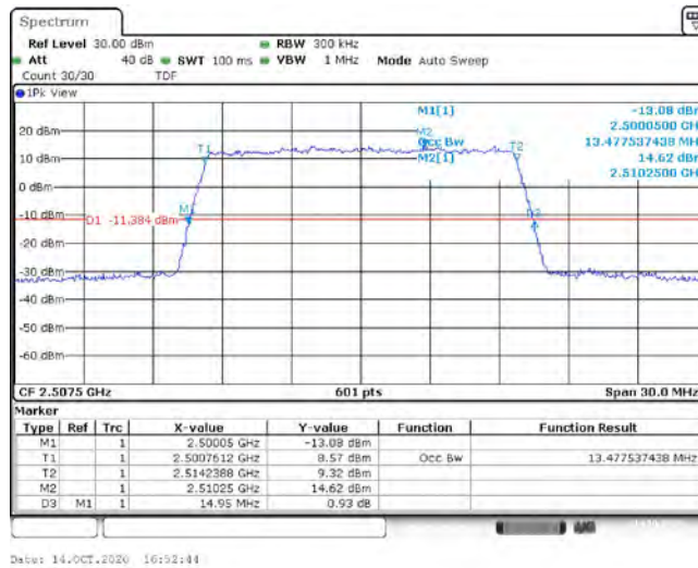
Band7-15MHz-QPSK-21100-75RB#0-13.478
