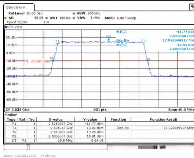
Band7-20MHz-QPSK-21350-100RB#0-17.97
