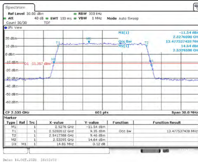
Band7-15MHz-QPSK-21375-75RB#0-13.478
