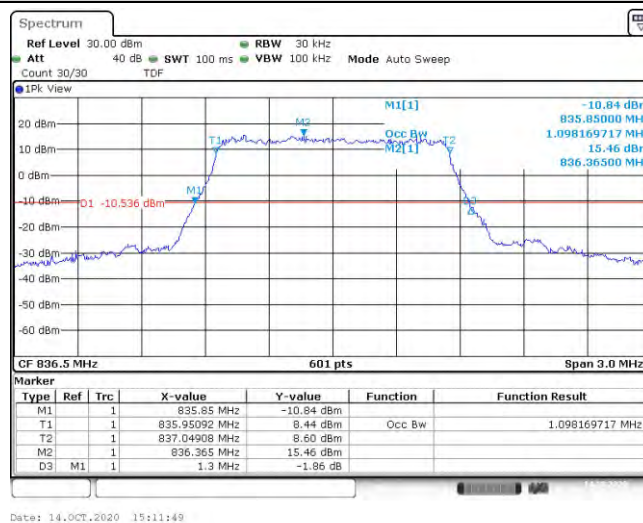
Band5-1.4MHz-16QAM-20643-6RB#0-1.103
