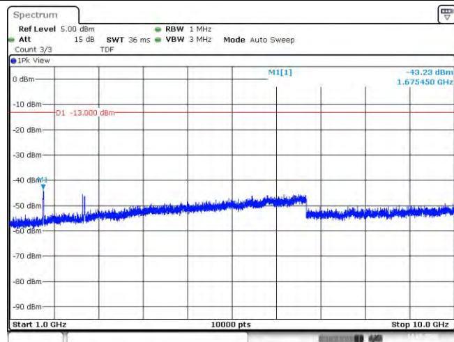
Band5-10MHz-16QAM-20525-50RB#0-Range2:1000~10000MHz
