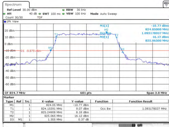
Band5-1.4MHz-QPSK-20407-6RB#0-1.093
