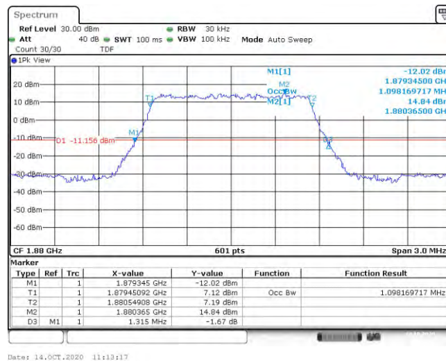
Band2-1.4MHz-QPSK-19193-6RB#0-1.093
