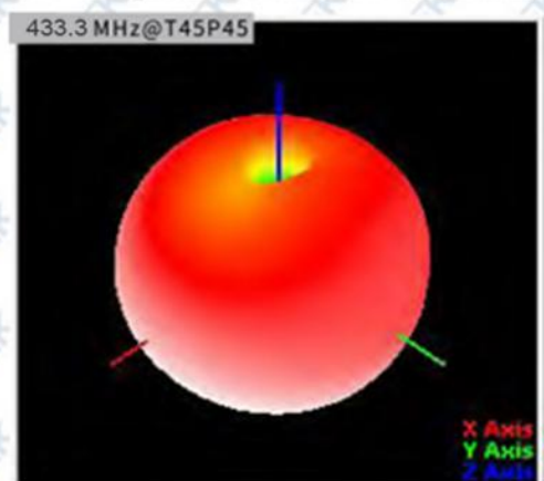
(4) Typical Free Space 3D Radiation Pattern at 433.3MHz:
