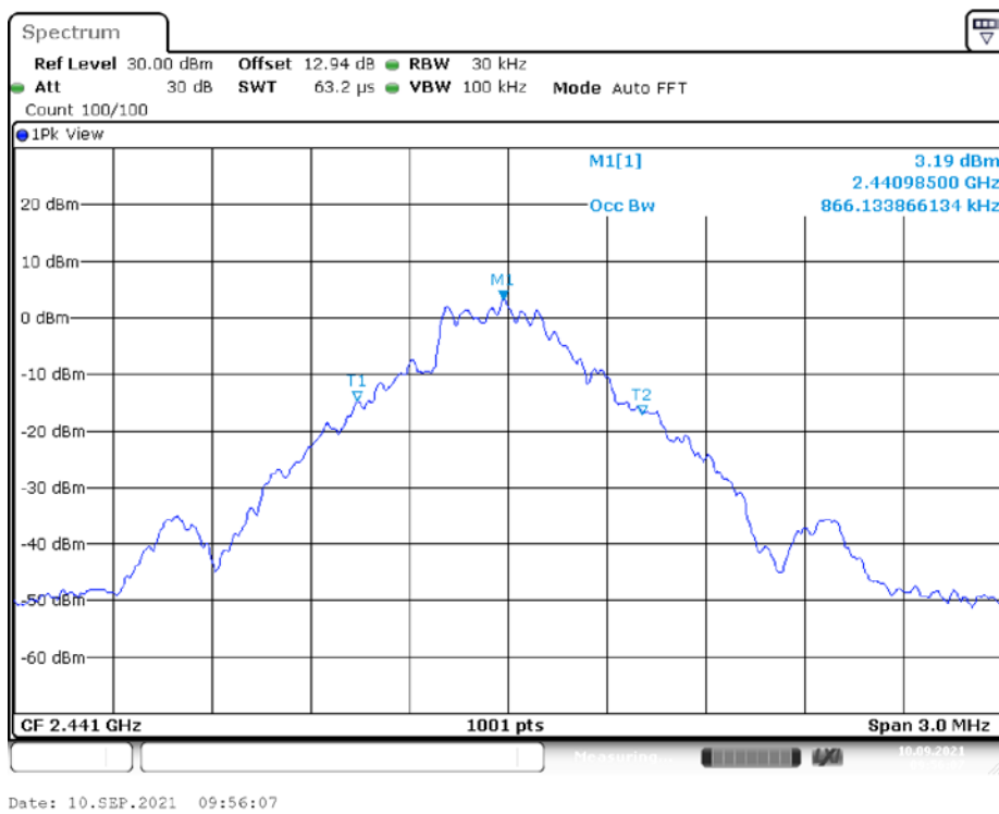
DH1_Ant1_2441MHz
