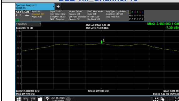
In-Band Reference Level BLE 1M_Channel 39
