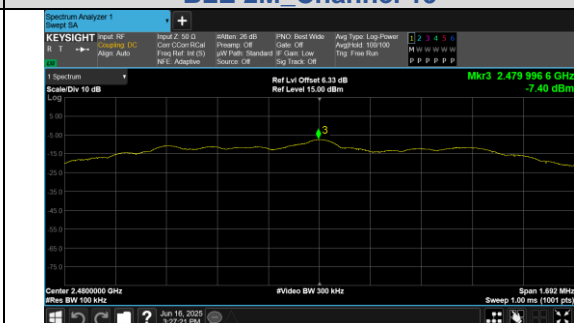
In-Band Reference Level BLE 2M_Channel 39
