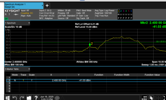
Out Of Band Emission BLE 2M_Channel 0
