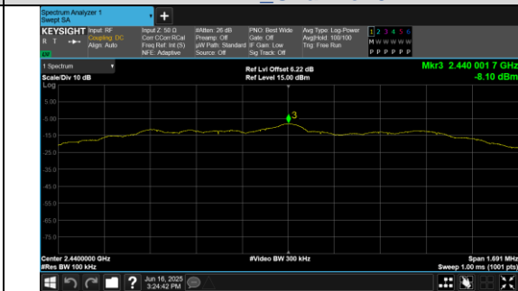
In-Band Reference Level BLE 2M_Channel 19
