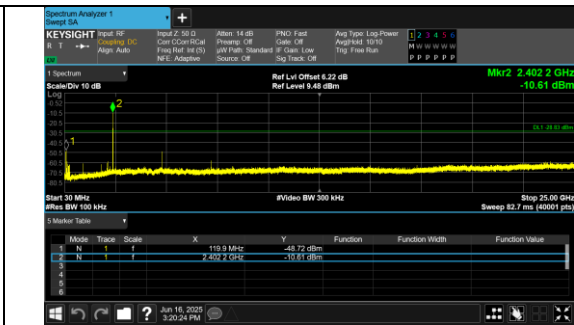
30.0 MHz - 25000.0 MHz BLE 2M_Channel 0
