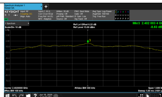
In-Band Reference Level BLE 2M_Channel 0
