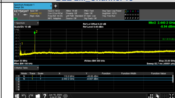
30.0 MHz - 25000.0 MHz BLE 2M_Channel 19
