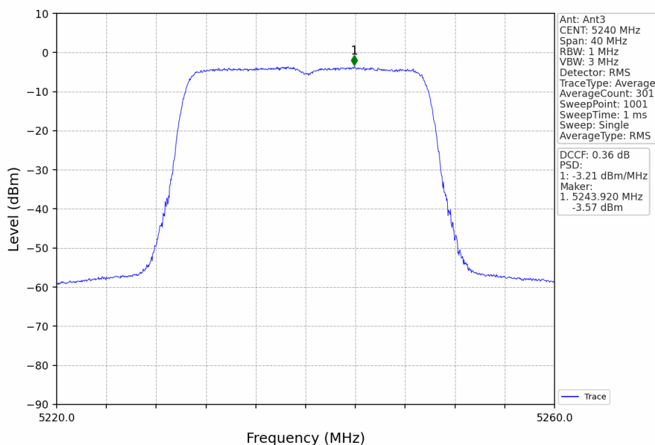
802.11ax(HEW20)_HCH_5240MHz_RU242_Left_Ant3_NTNV
