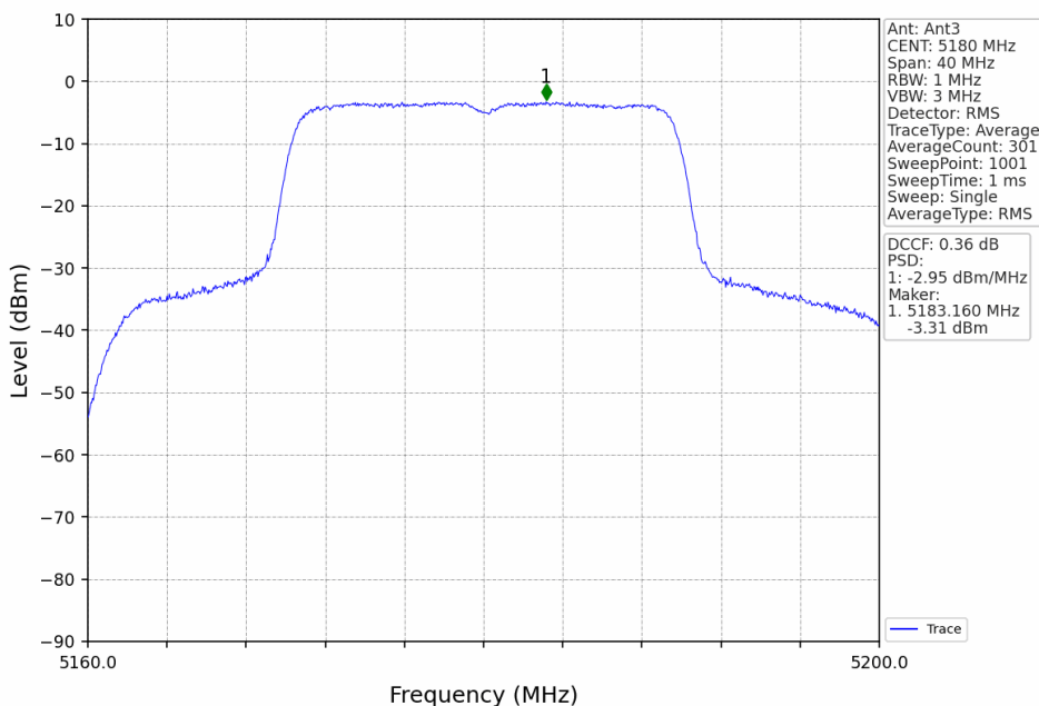
802.11ax(HEW20)_LCH_5180MHz_RU242_Left_Ant3_NTNV
