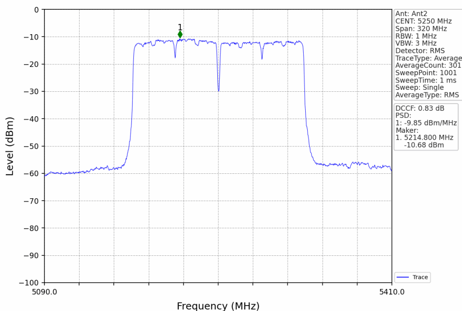
802.11ac(VHT160)_MCH_5250MHz_Ant2_NTNV
