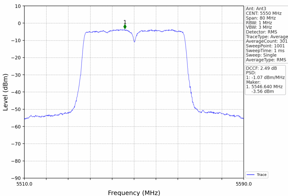
802.11n(HT40)_MCH_5550MHz_Ant3_NTNV
