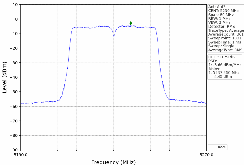
802.11ac(VHT40)_HCH_5230MHz_Ant3_NTNV
