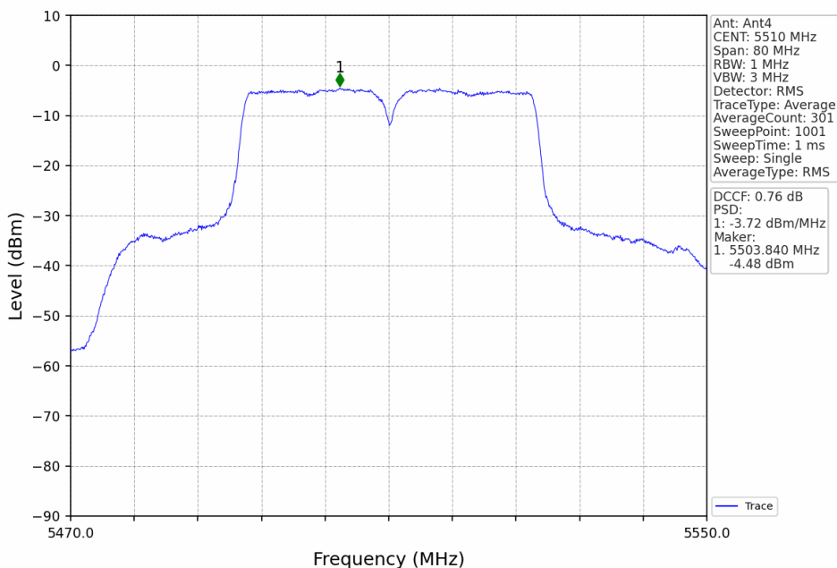
802.11ac(VHT40)_LCH_5510MHz_Ant4_NTNV
