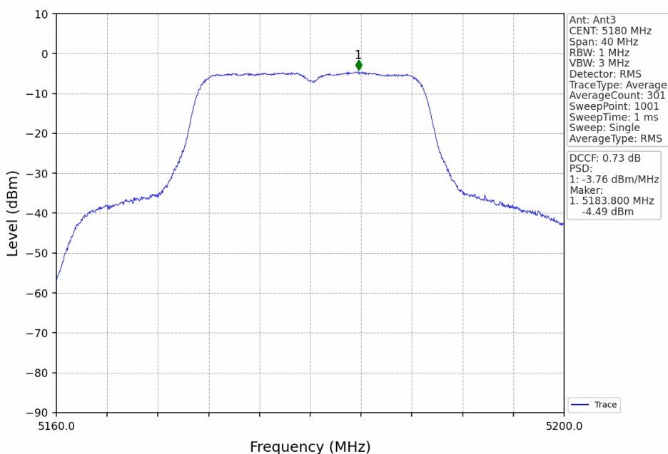
802.11ac(VHT20)_LCH_5180MHz_Ant3_NTNV
