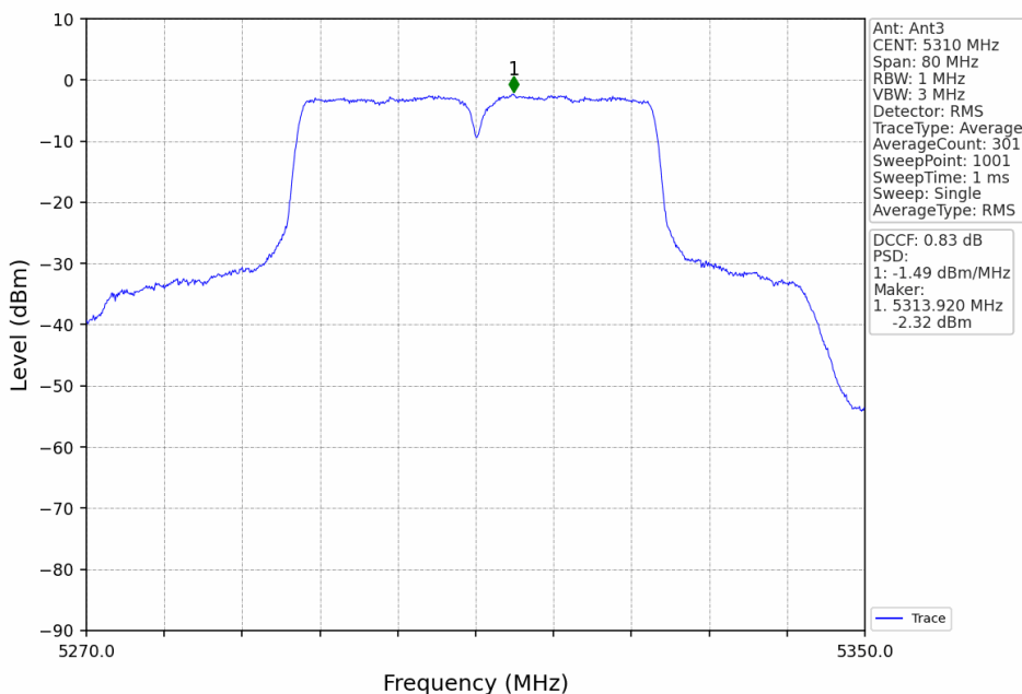
802.11ac(VHT40)_HCH_5310MHz_Ant3_NTNV
