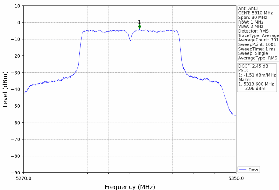
802.11n(HT40)_HCH_5310MHz_Ant3_NTNV
