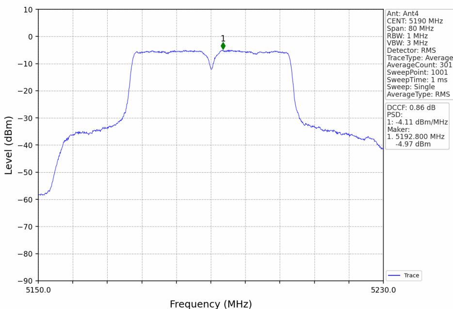
802.11ac(VHT40)_LCH_5190MHz_Ant4_NTNV
