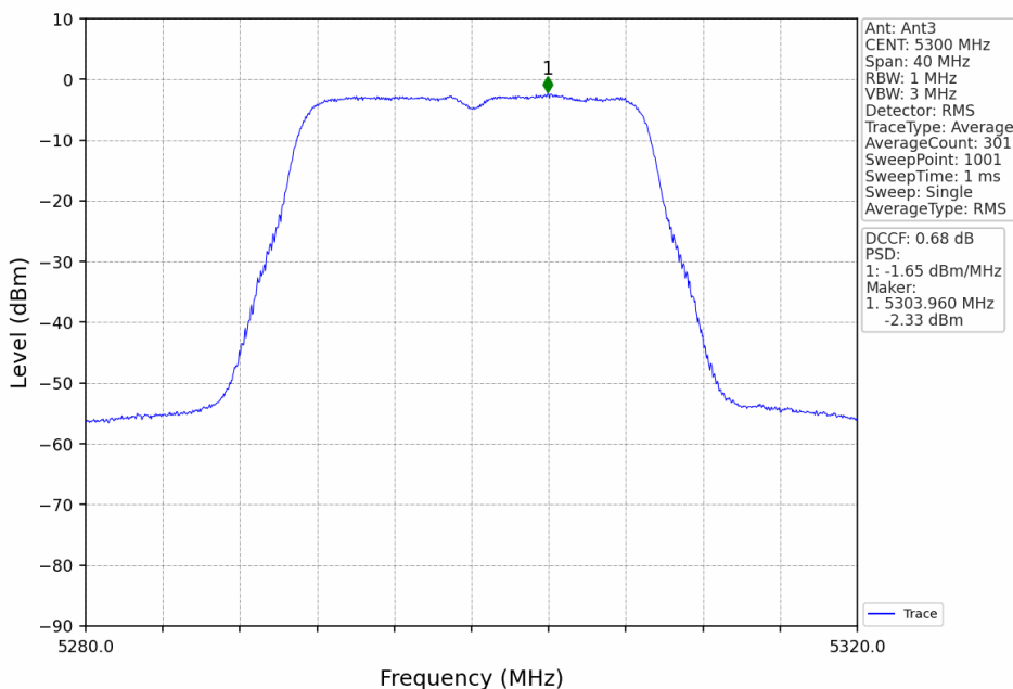
802.11ac(VHT20)_MCH_5300MHz_Ant3_NTNV
