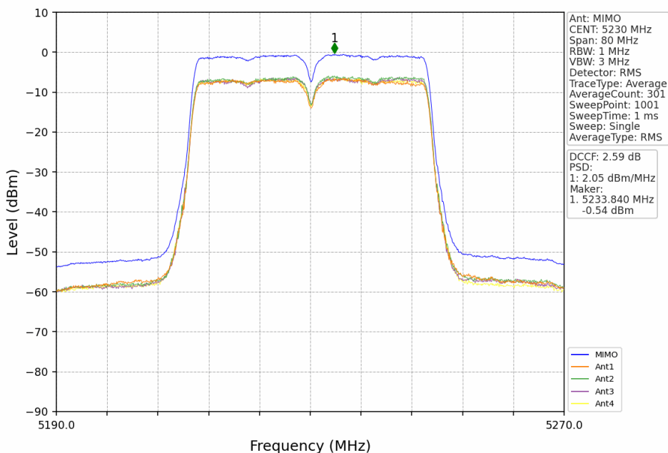
802.11n(HT40)_HCH_5230MHz_MIMO_NTNV
