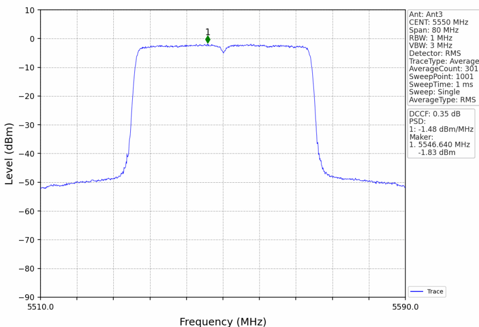
802.11ax(HEW40)_MCH_5550MHz_RU484_Left_Ant3_NTNV
