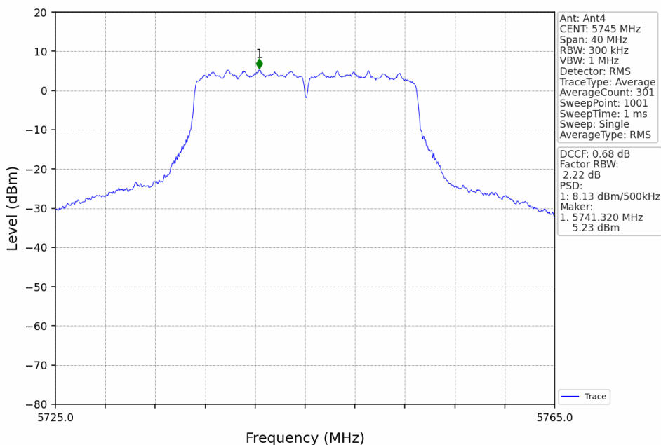
802.11ac(VHT20)_LCH_5745MHz_Ant4_NTNV
