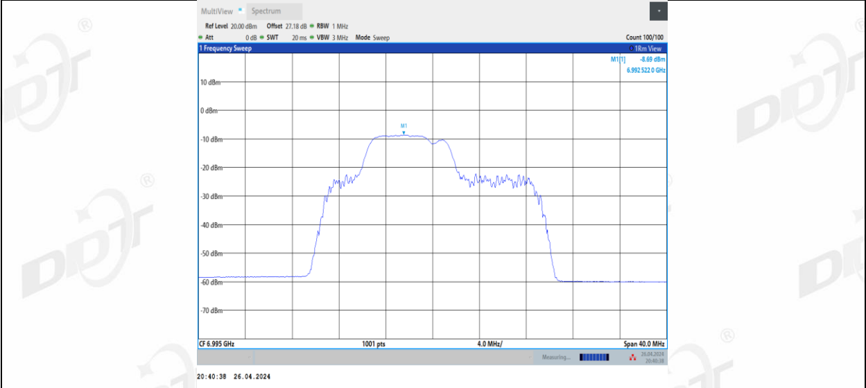
11BE20MIMO Ant1_6995_52+26_3
