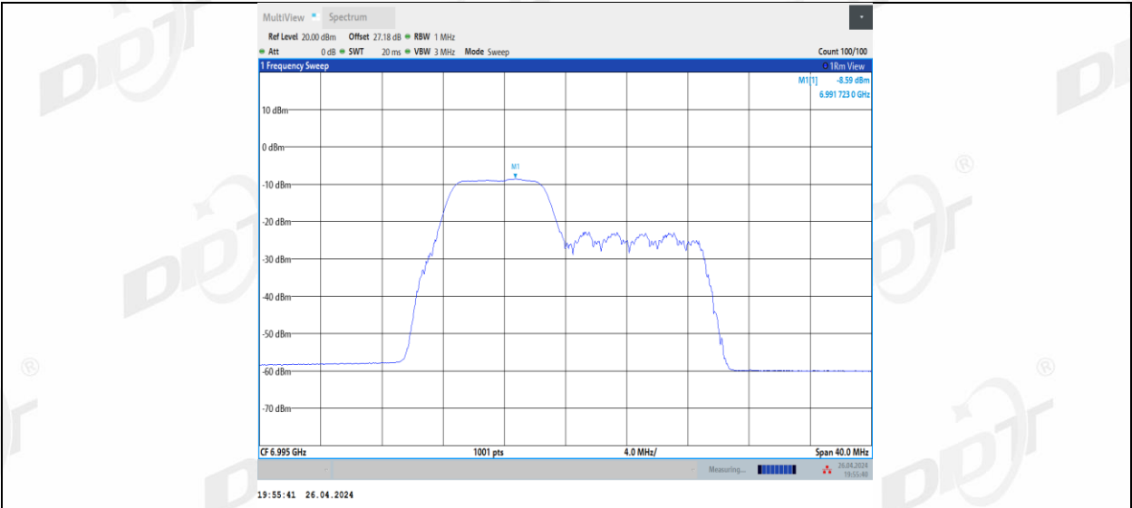
11BE20MIMO Ant1_6995_52+26_2
