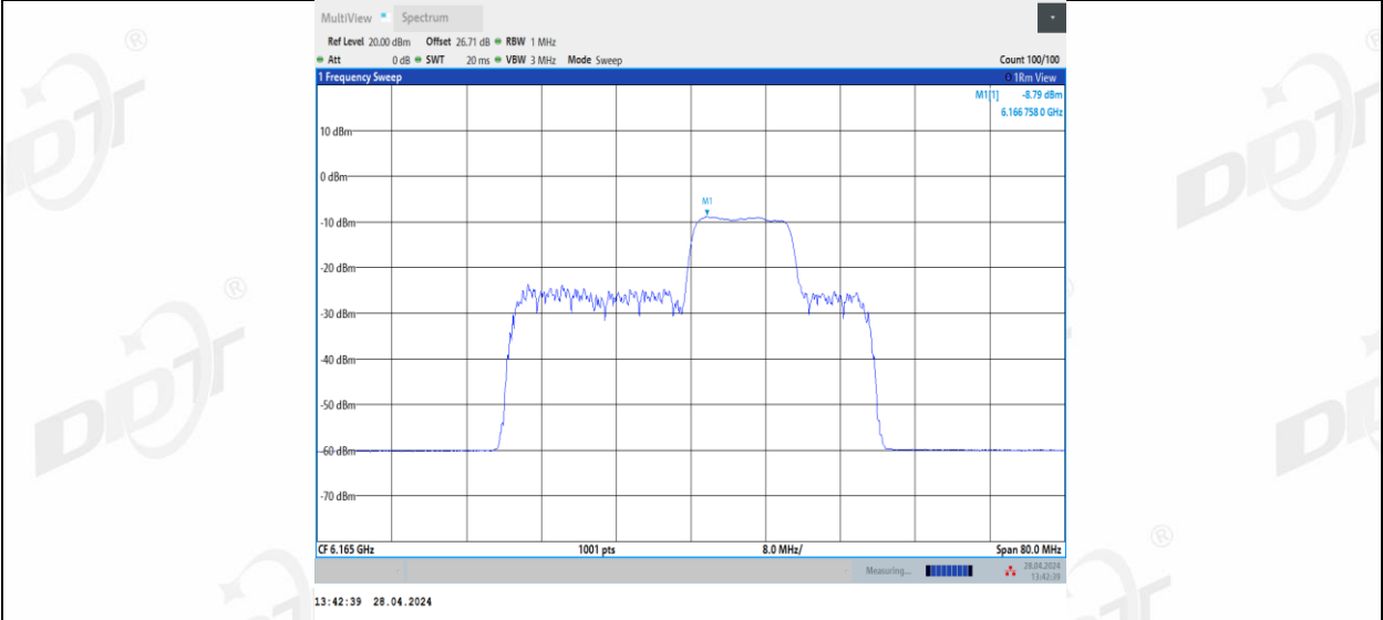
11BE40MIMO_Ant3_6165_106+26_4
