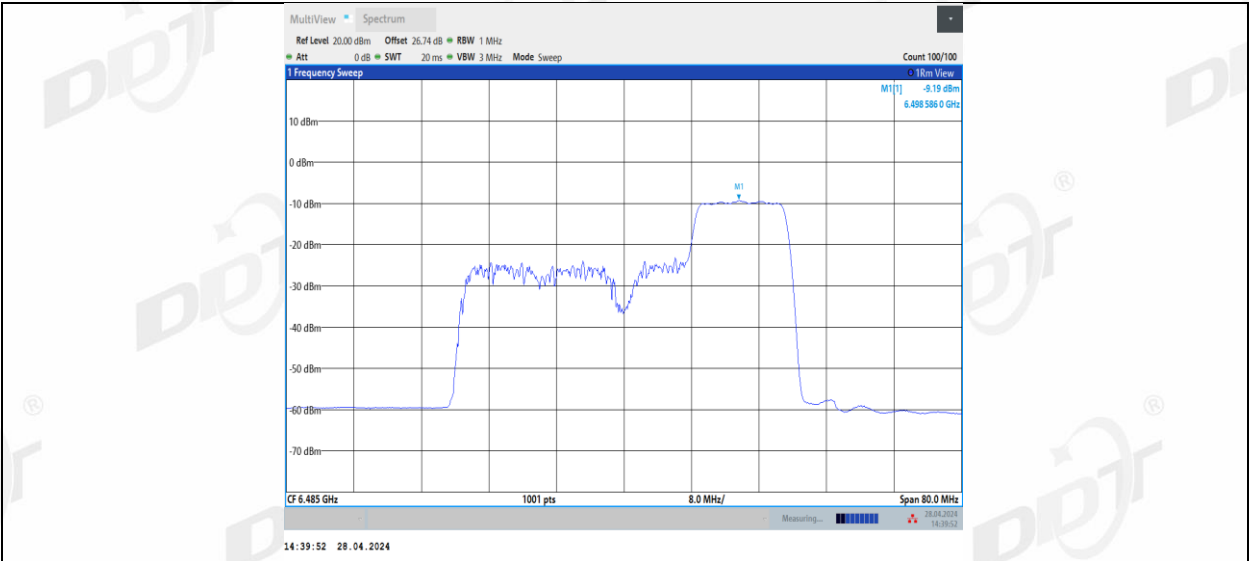
11BE40MIMO_Ant3_6485_106+26_3
