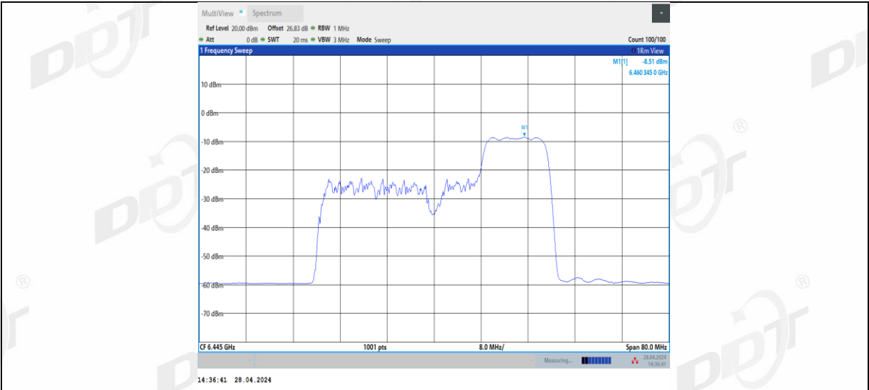
11BE40MIMO_Ant3_6445_106+26_3
