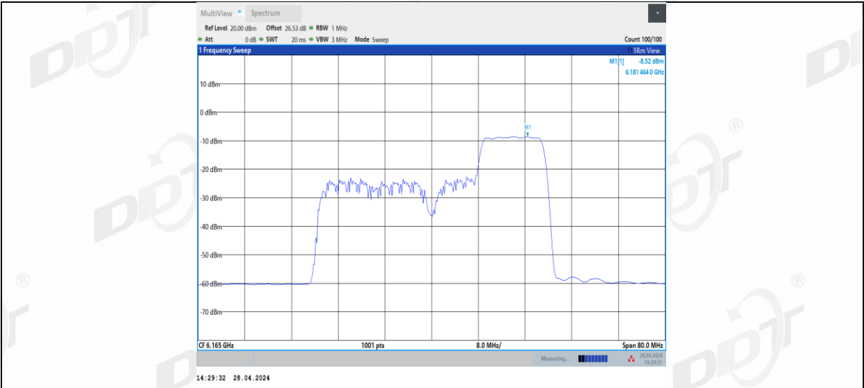
11BE40MIMO_Ant3_6165_106+26_3
