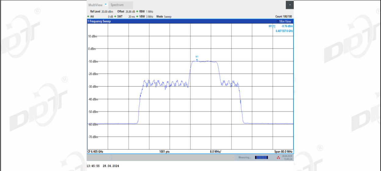
11BE40MIMO_Ant3_6405_106+26_4
