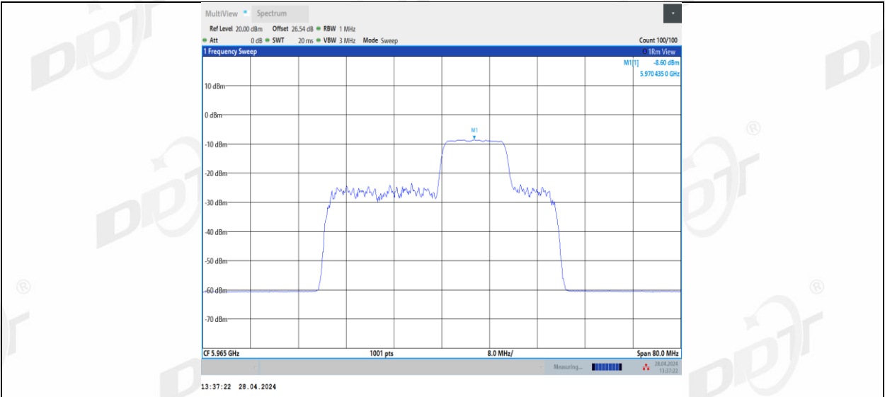
11BE40MIMO_Ant1_5965_106+26_4
