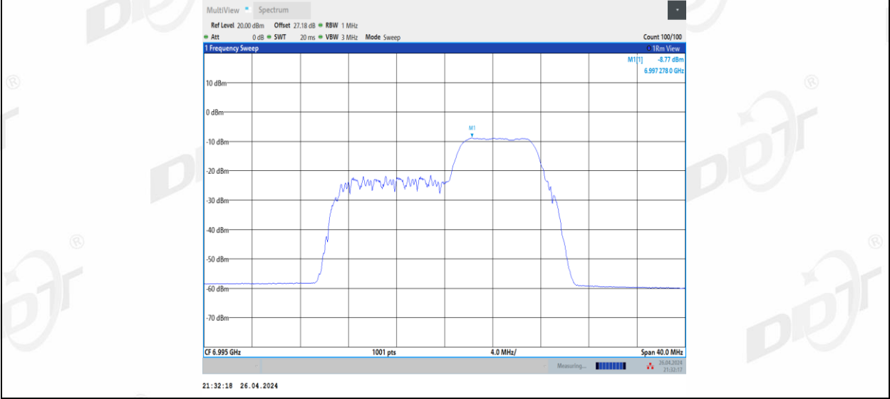
11BE20MIMO Ant1_6995_106+26_1
