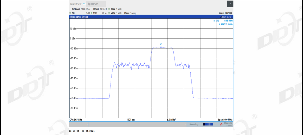
11BE40MIMO_Ant3_6565_106+26_4
