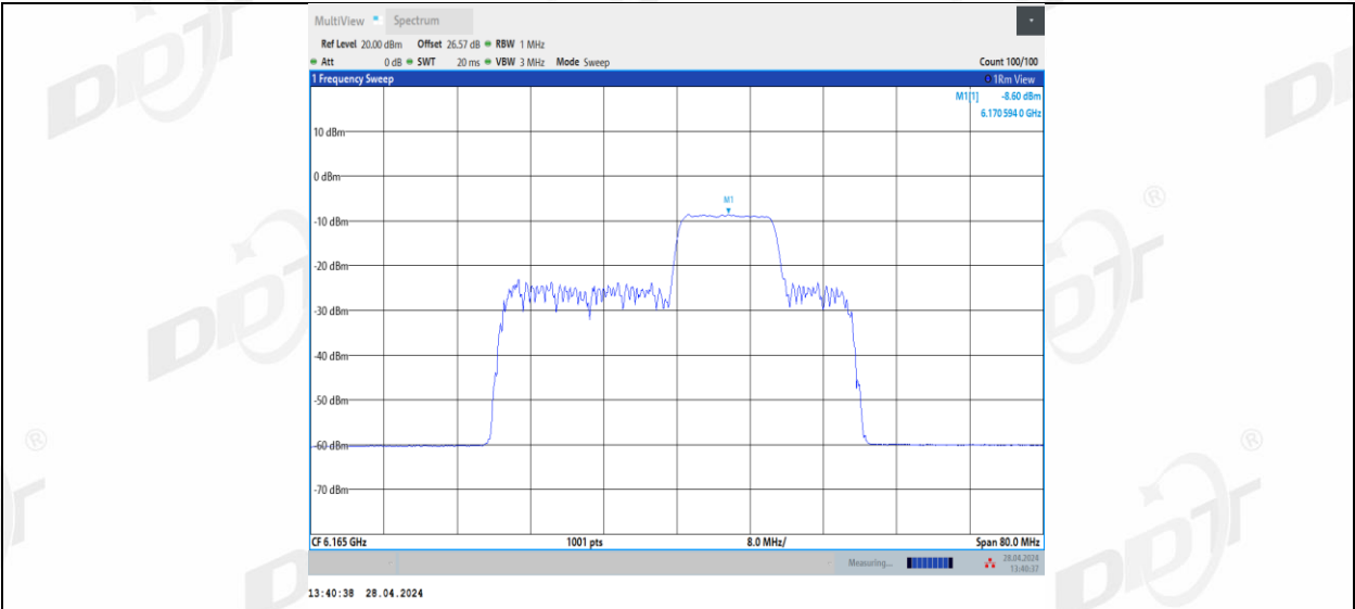
11BE40MIMO_Ant1_6165_106+26_4
