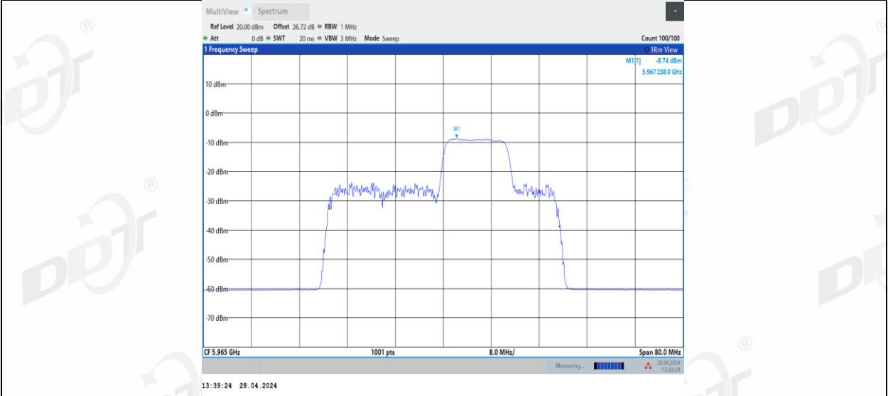
11BE40MIMO_Ant3_5965_106+26_4
