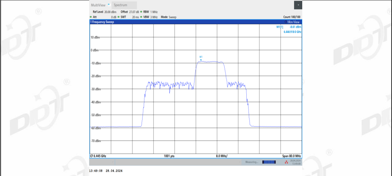
11BE40MIMO_Ant3_6445_106+26_4
