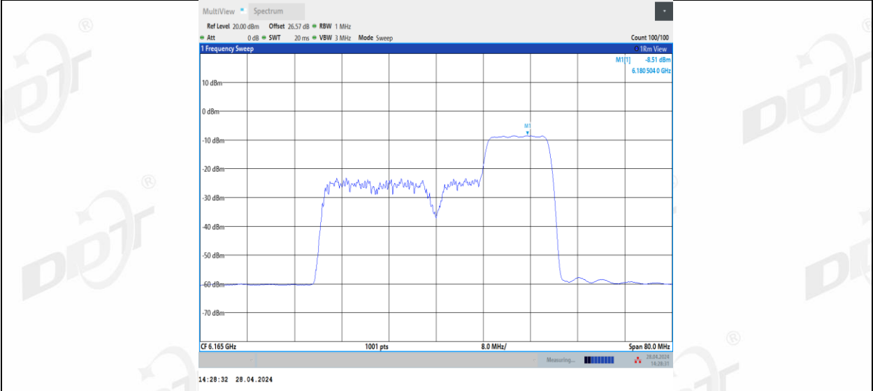
11BE40MIMO_Ant2_6165_106+26_3
