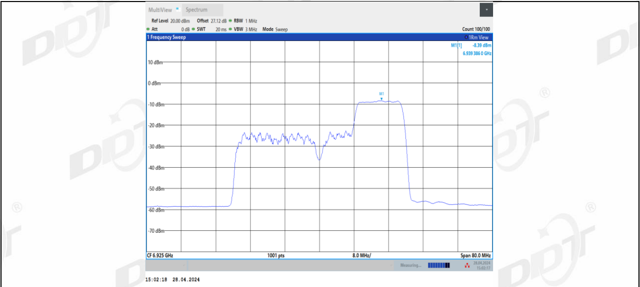
11BE40MIMO_Ant3_6925_106+26_3
