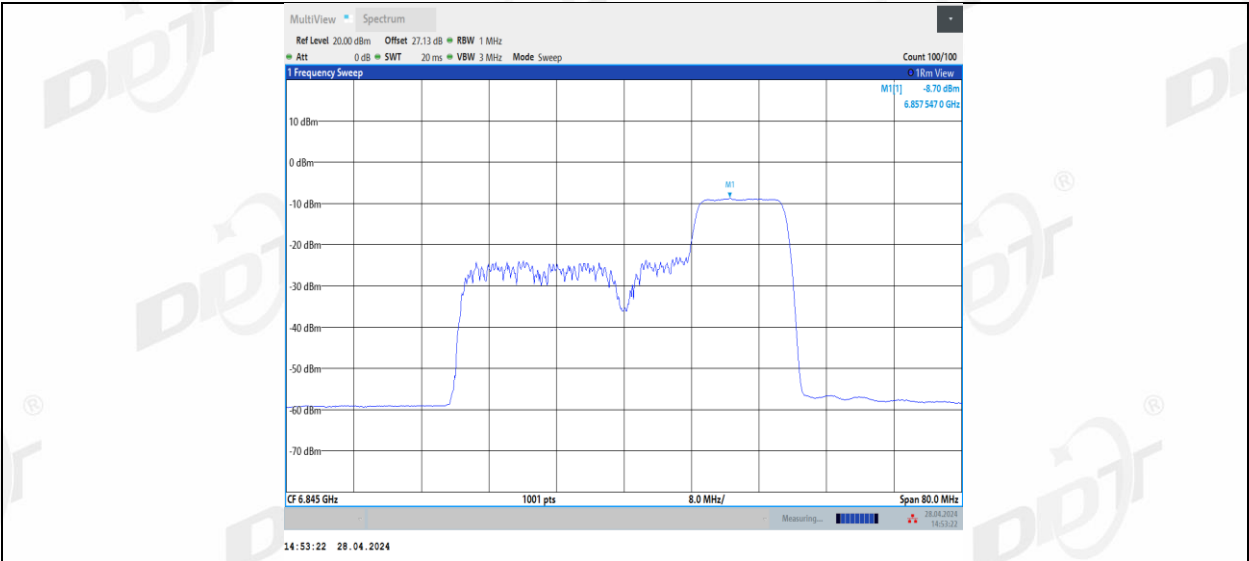
11BE40MIMO_Ant3_6845_106+26_3
