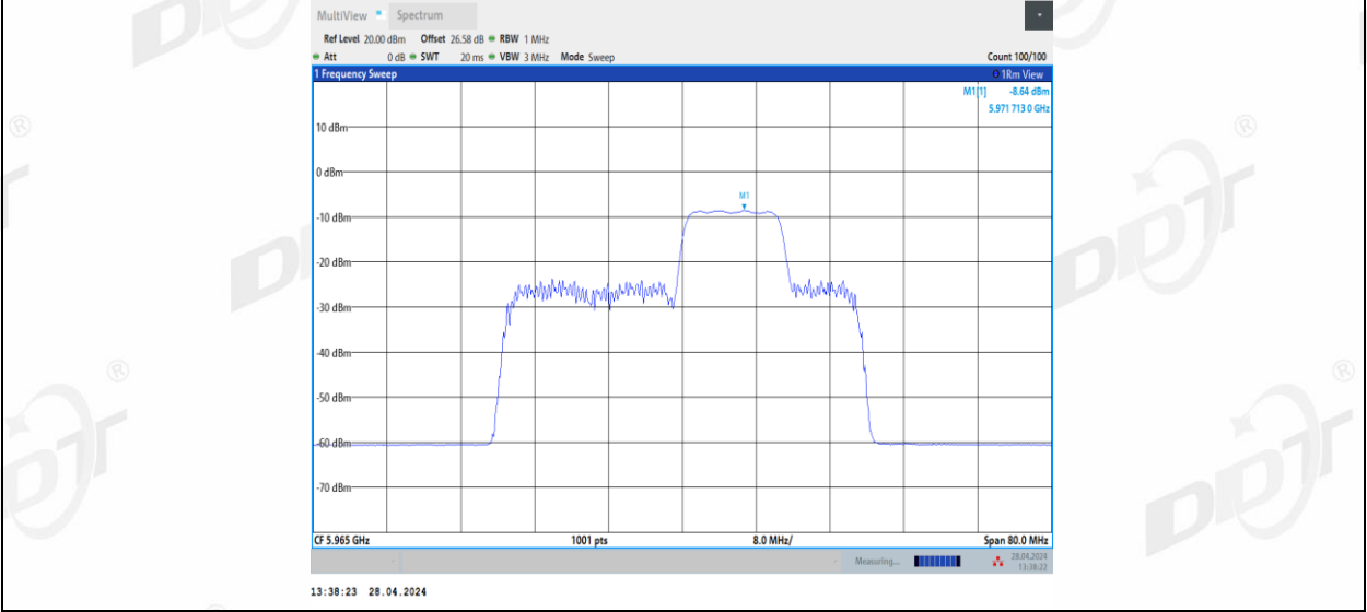
11BE40MIMO_Ant2_5965_106+26_4
