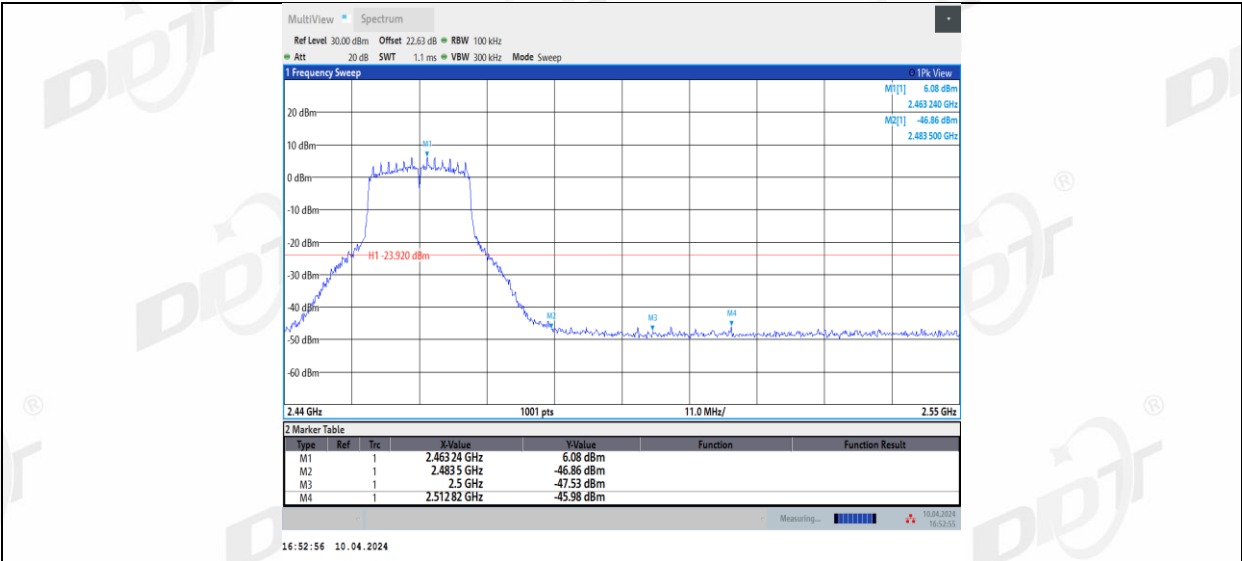
11G-CDD_Ant2_High_2462
