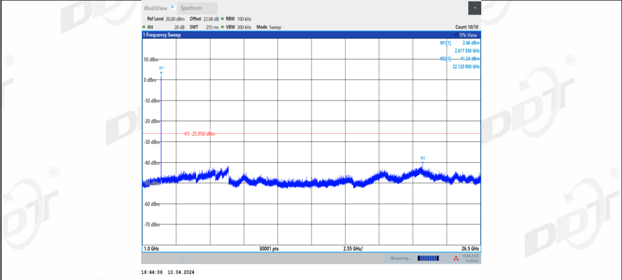
11G-CDD_Ant2_2412_0~Reference
