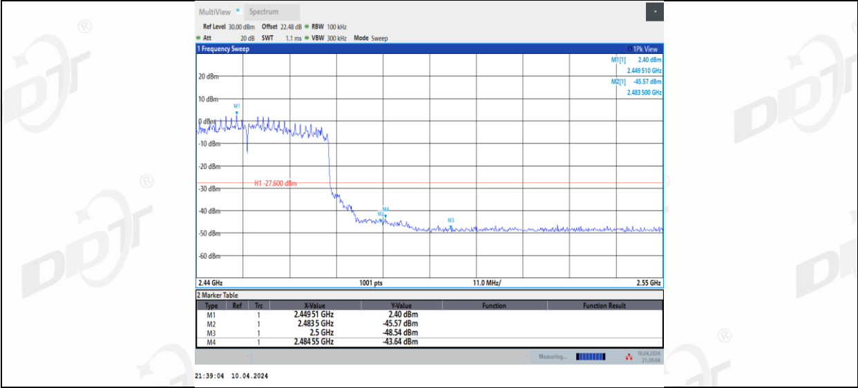
11BE40MIMO_Ant2_High_2452
