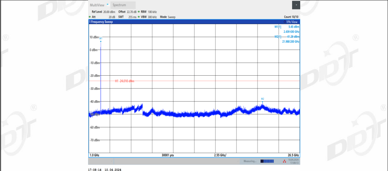
11G-CDD_Ant1_2462_0~Reference
