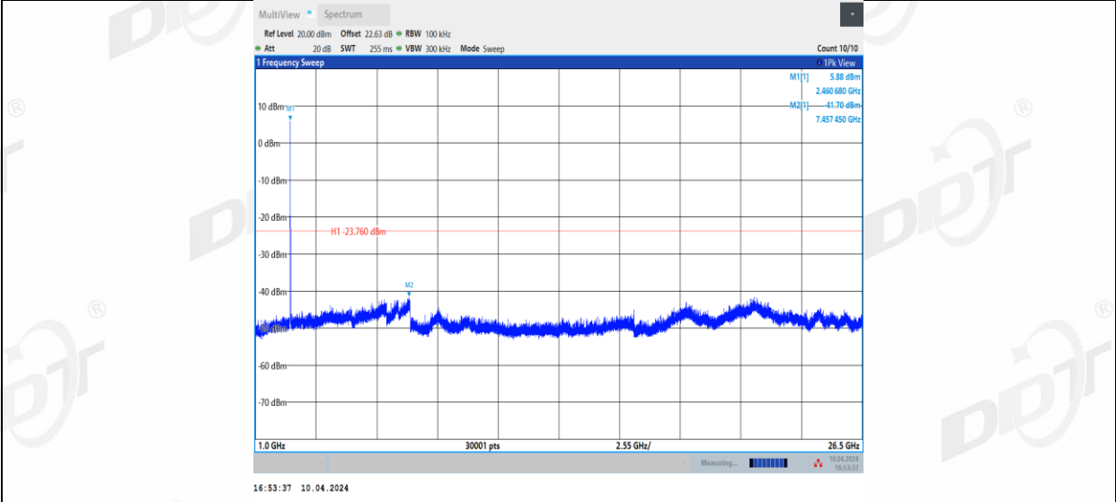
11G-CDD_Ant2_2462_0~Reference
