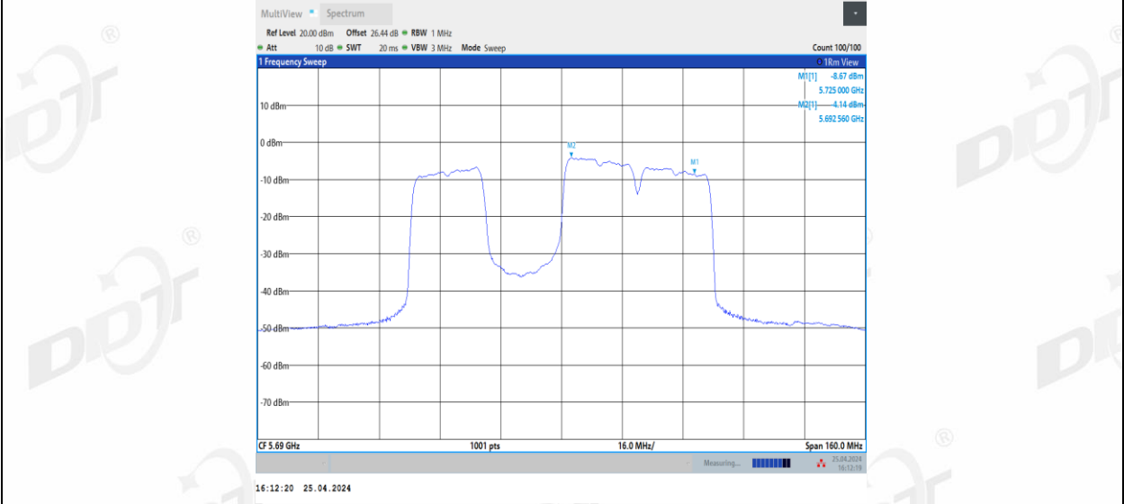
11BE80MIMO Ant1 5690 UNII-2C 484+242 Non-OFDMA 3
