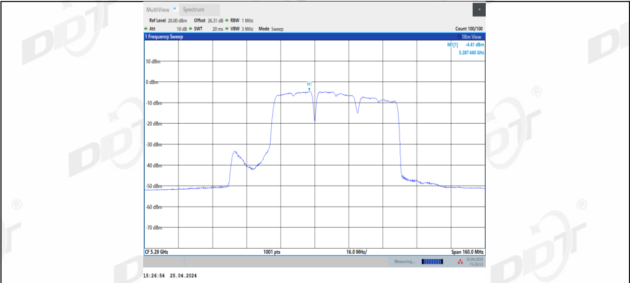
11BE80MIMO Ant1 5290 484+242 Non-OFDMA 2
