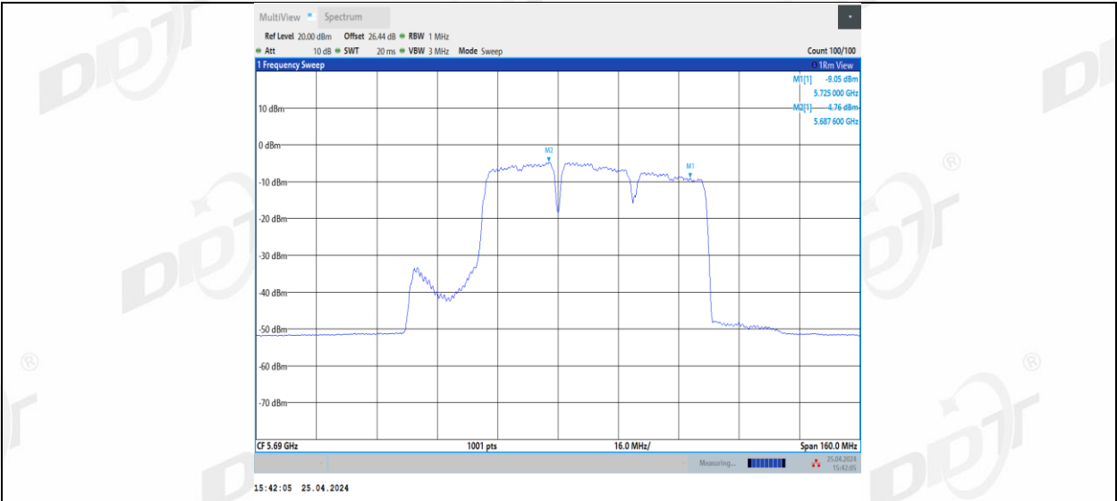
11BE80MIMO Ant1 5690 UNII-2C 484+242 Non-OFDMA 2
