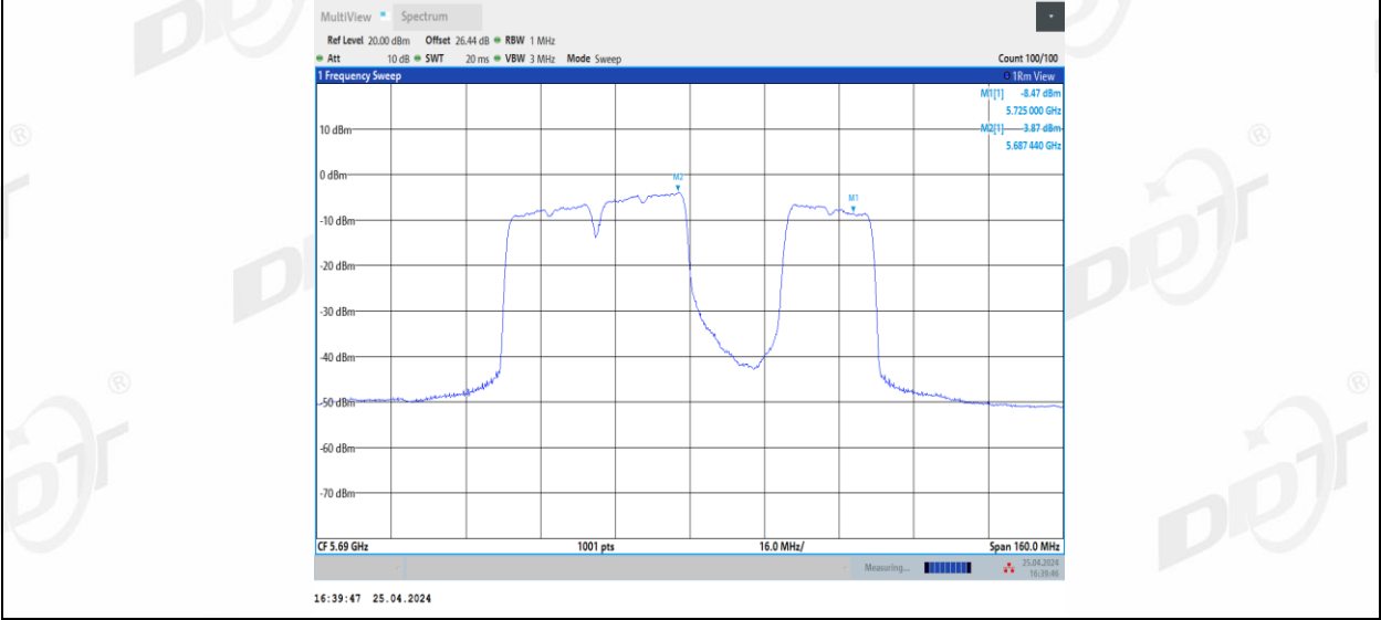
11BE80MIMO Ant1 5690 UNII-2C 484+242 Non-OFDMA 4
