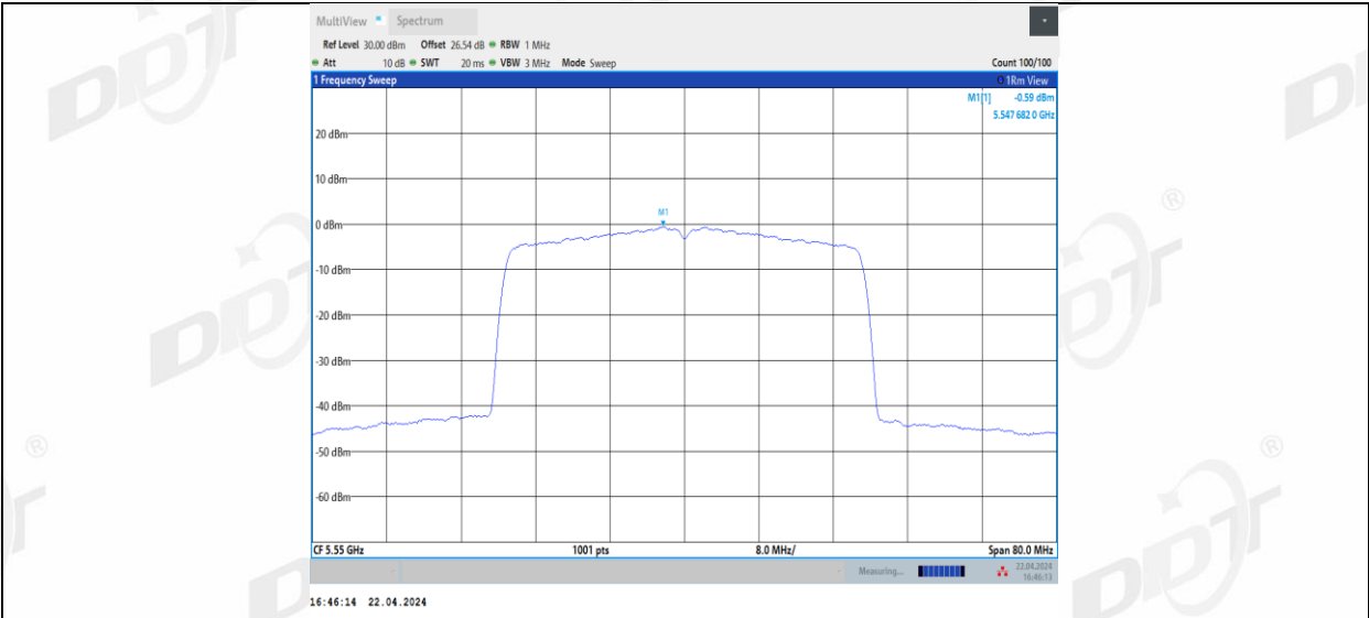
11BE40MIMO Ant2_5550
