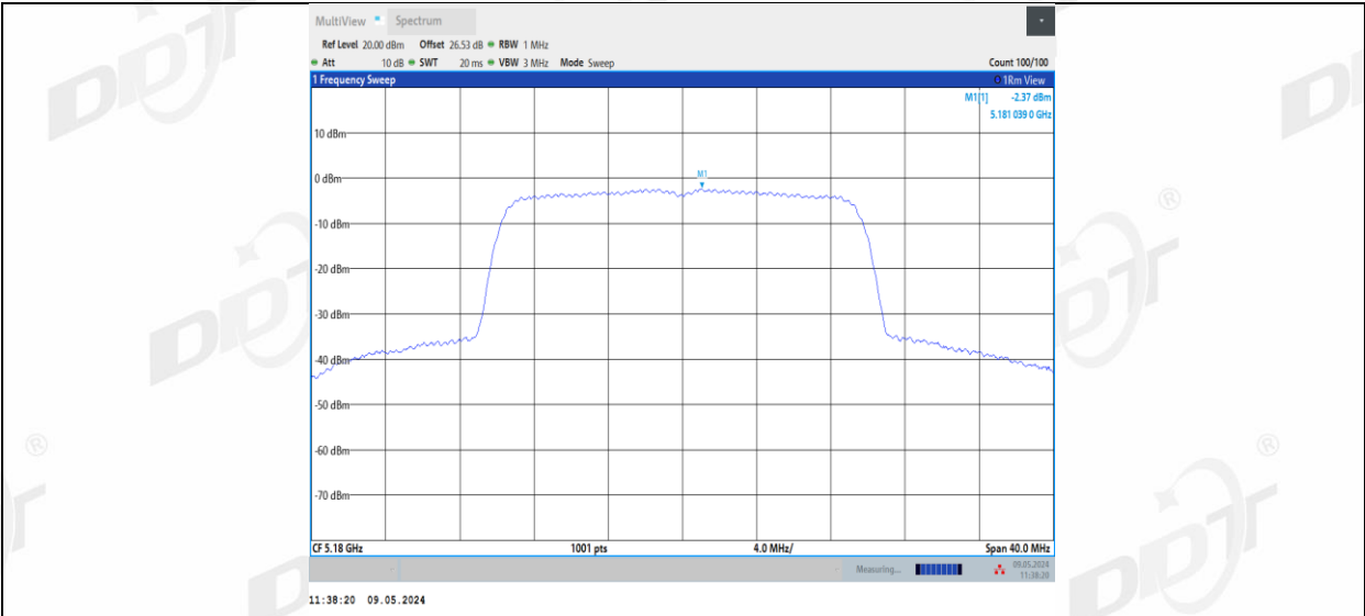
11BE20MIMO Ant2_5180
