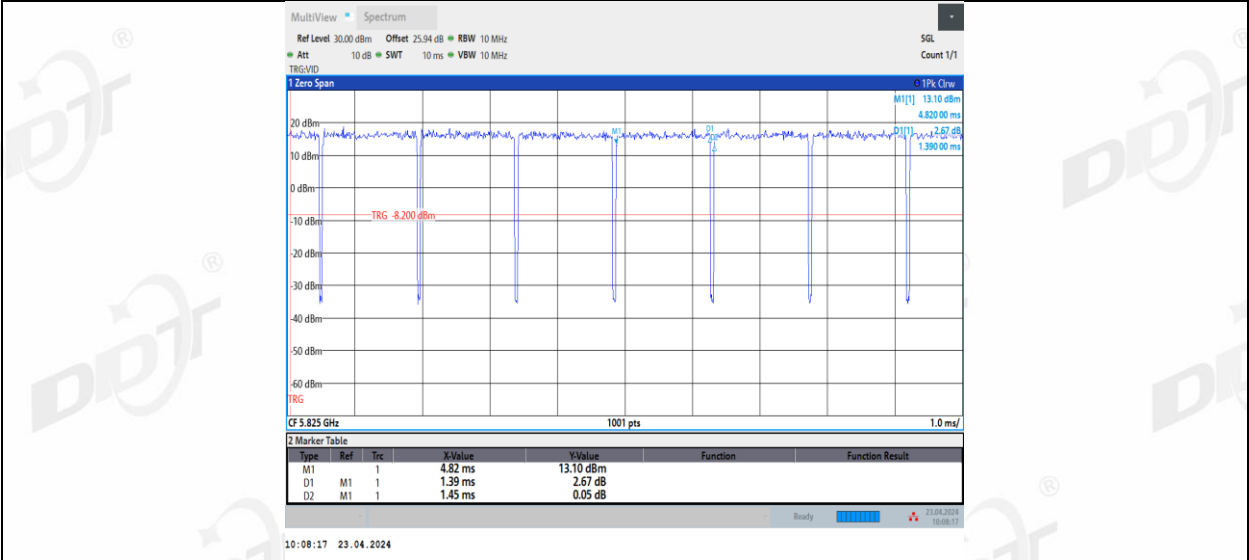
11A-CDD_Ant3_5825
