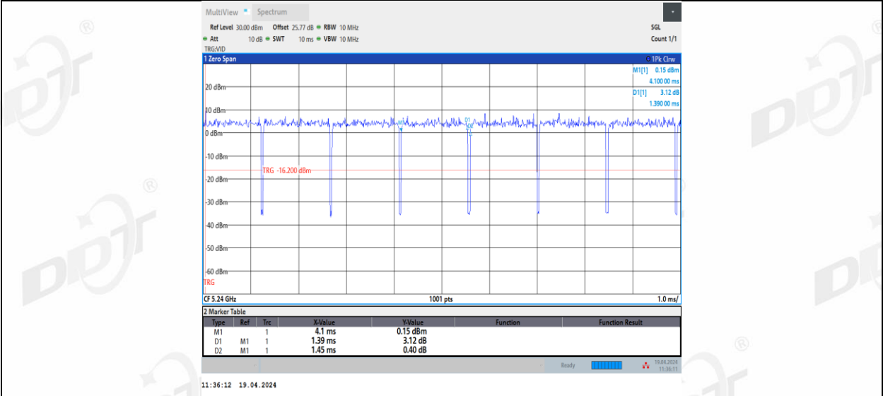
11A-CDD_Ant3_5240
