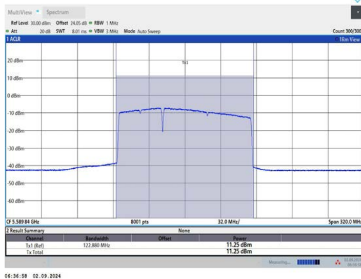
11BE160MIMO Ant2 5570 996+484 OFDMA_2
