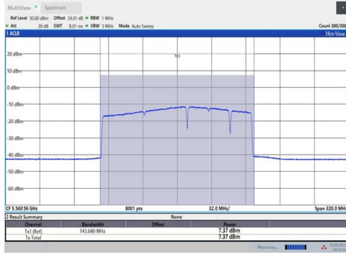
11BE160MIMO_Ant2_5570_996+484+242_OFDMA_8
