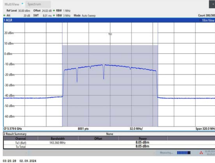
11BE160MIMO Ant3 5570 996+484+242 OFDMA 1
