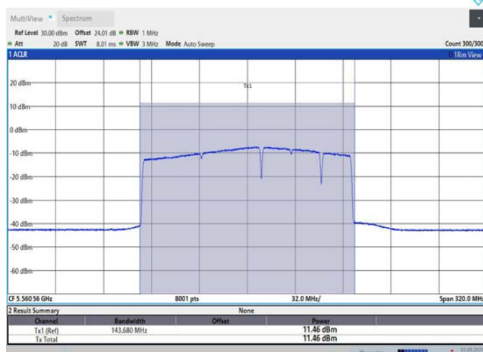
11BE160MIMO_Ant3_5570_996+484_OFDMA_1
