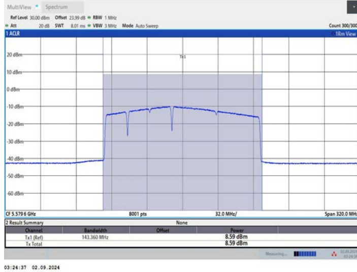
11BE160MIMO Ant1 5570 996+484+242 OFDMA 1
