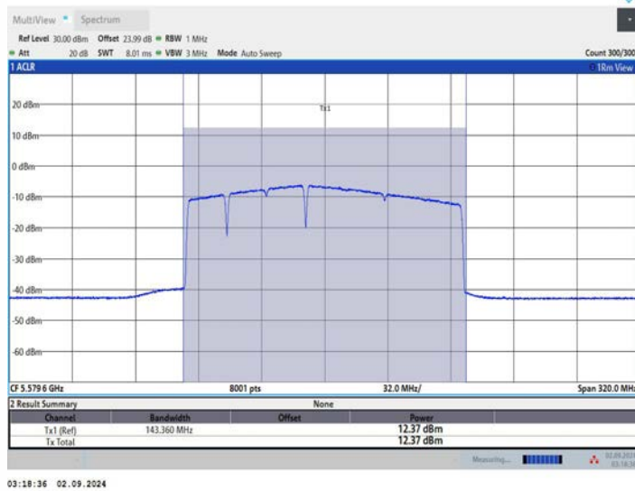
11BE160MIMO Ant1 5570 996+484+242 OFDMA 2
