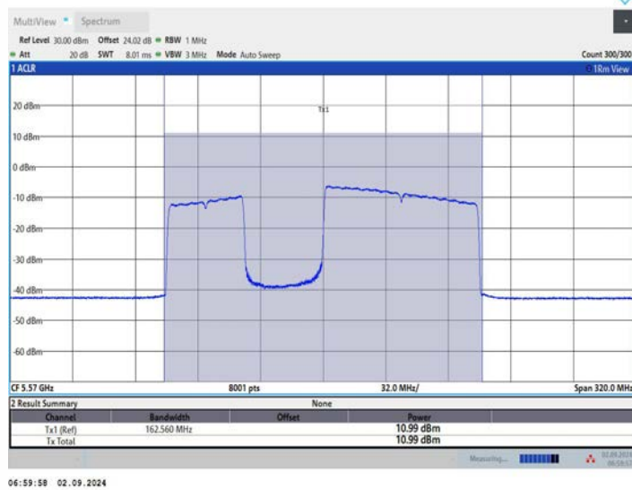
11BE160MIMO Ant3 5570 996+484 OFDMA 3
