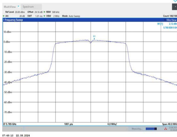
11A_Ant3_5785
