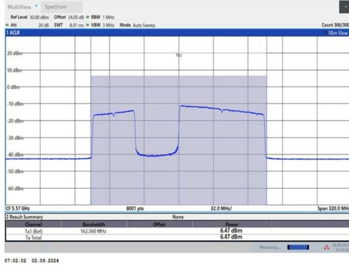
11BE160MIMO Ant2 5570 996+484 OFDMA 2
