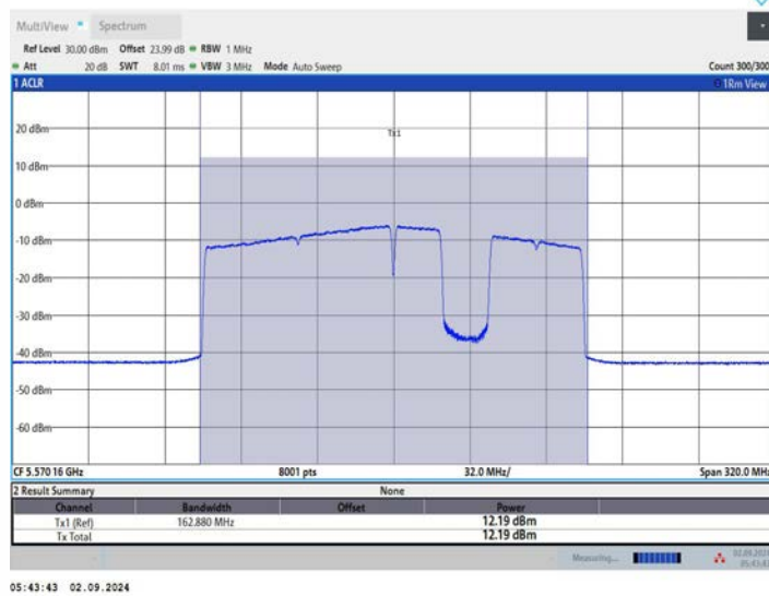
11BE160MIMO_Ant1_5570_996+484+242_OFDMA_7
