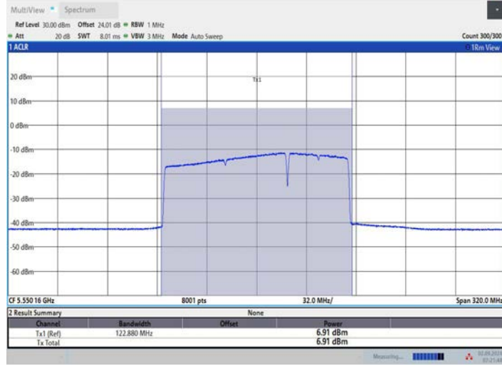
11BE160MIMO Ant2 5570 996+484 OFDMA 4
