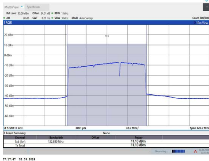
11BE160MIMO Ant2 5570 996+484+242 OFDMA 1
