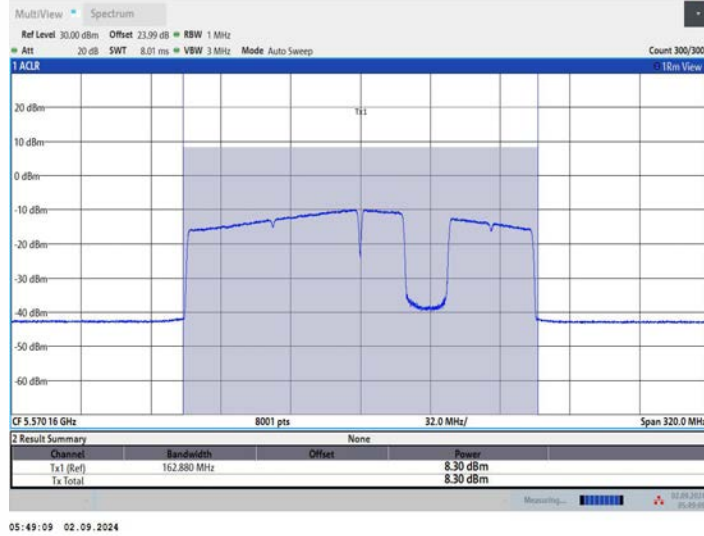
11BE160MIMO_Ant1_5570_996+484+242_OFDMA_6
