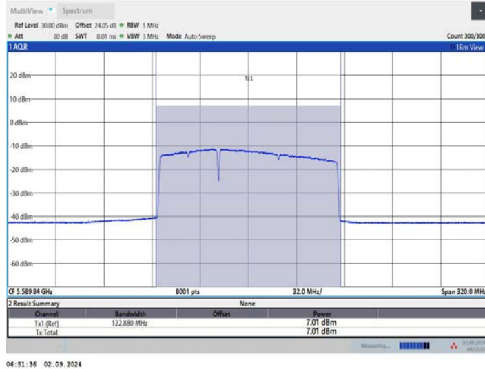
11BE160MIMO Ant2 5570 996+484 OFDMA_1
