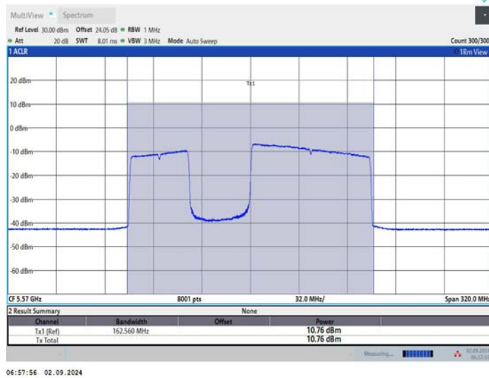
11BE160MIMO Ant2 5570 996+484 OFDMA 3
