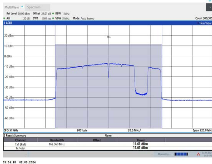
11BE160MIMO_Ant2_5570_996+484+242_OFDMA_8
