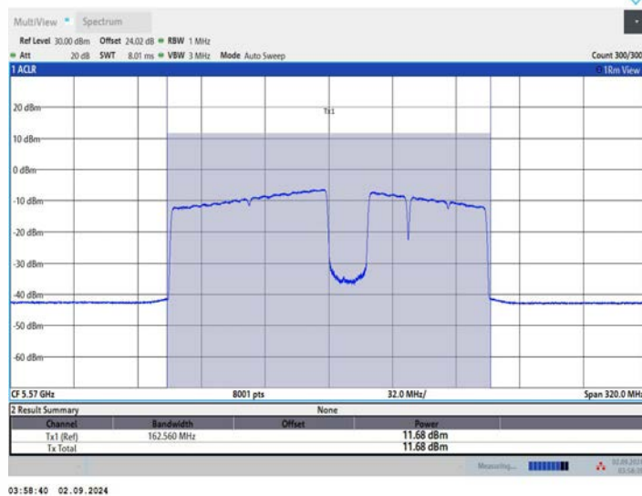
11BE160MIMO_Ant3_5570_996+484+242_OFDMA_6
