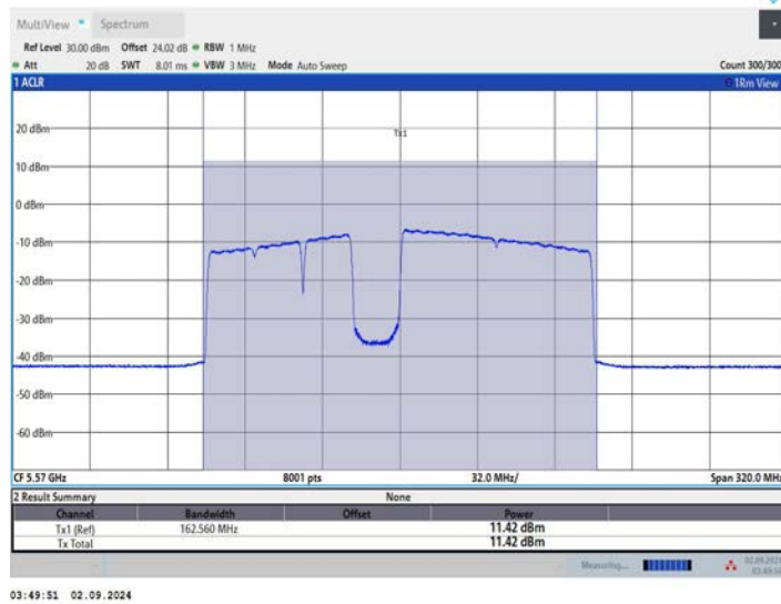
11BE160MIMO_Ant3_5570_996+484+242_OFDMA_5
