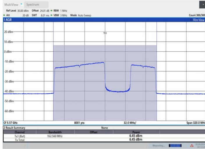
11BE160MIMO Ant2 5570 996+484 OFDMA 3
