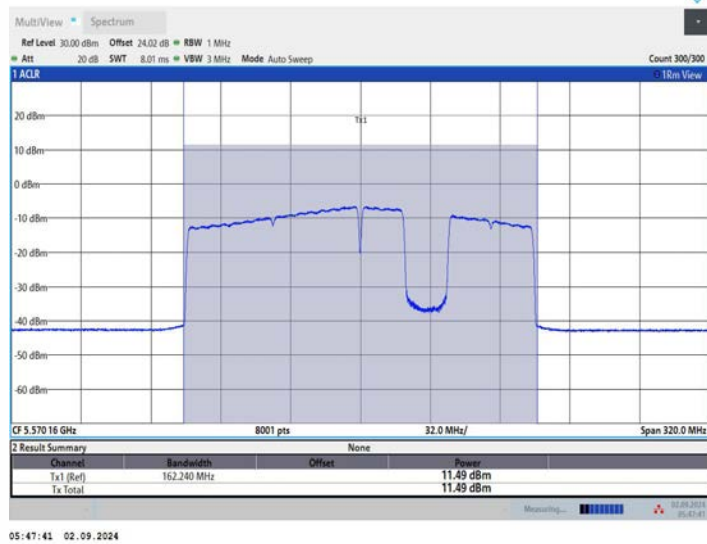
11BE160MIMO_Ant3_5570_996+484+242_OFDMA_7
