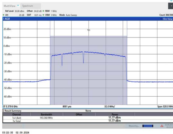
11BE160MIMO Ant3 5570 996+484+242 OFDMA 2
