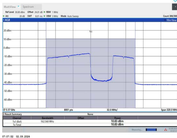
11BE160MIMO Ant2 5570 996+484 OFDMA 4
