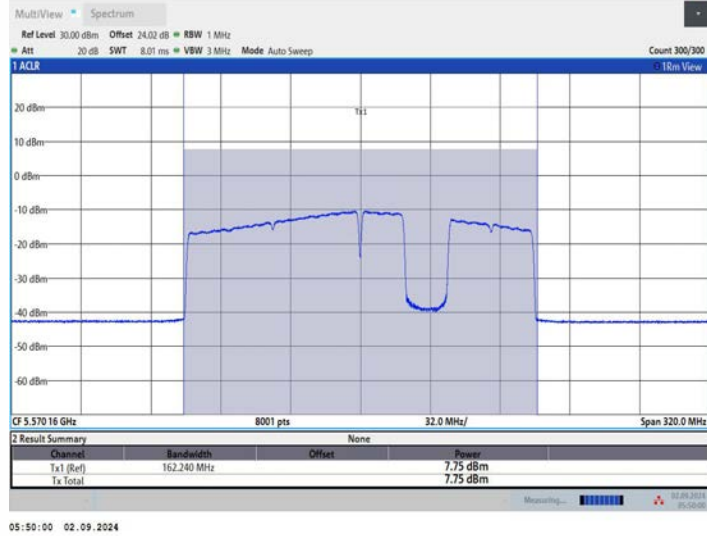
11BE160MIMO_Ant3_5570_996+484+242_OFDMA_6
