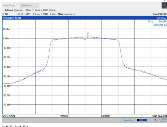
11A_Ant3_5745
