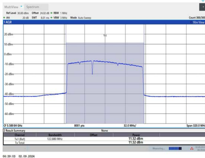
11BE160MIMO Ant3 5570 996+484 OFDMA 2
