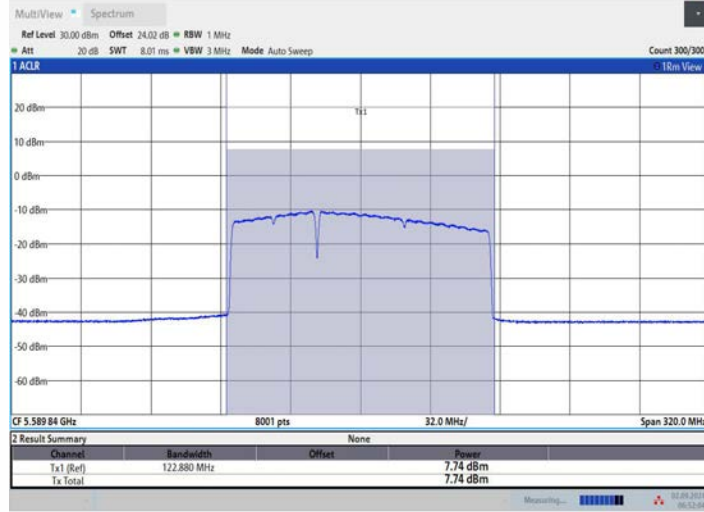
11BE160MIMO Ant3 5570 996+484 OFDMA 1
