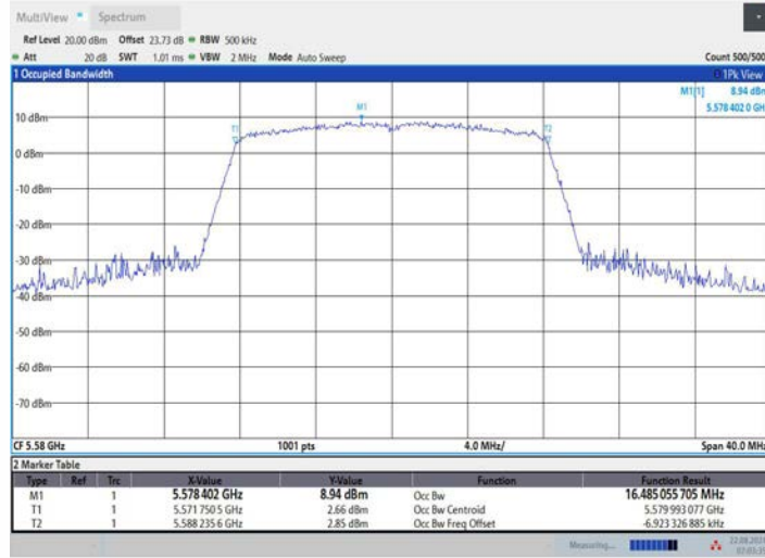
11A_Ant3_5580
