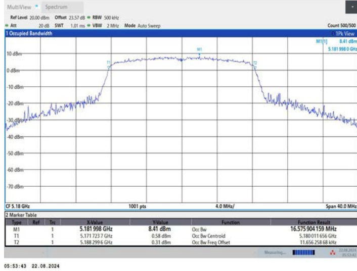
11A_Ant2_5180
