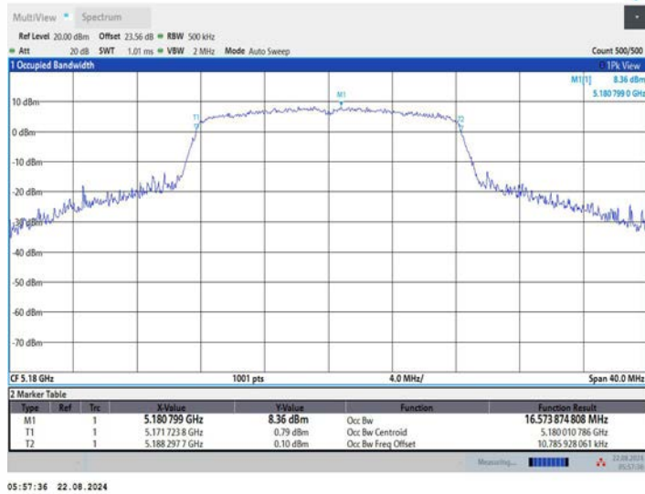
11A_Ant3_5180
