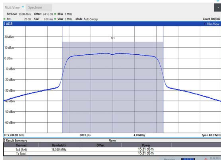
11A_Ant3_5785
