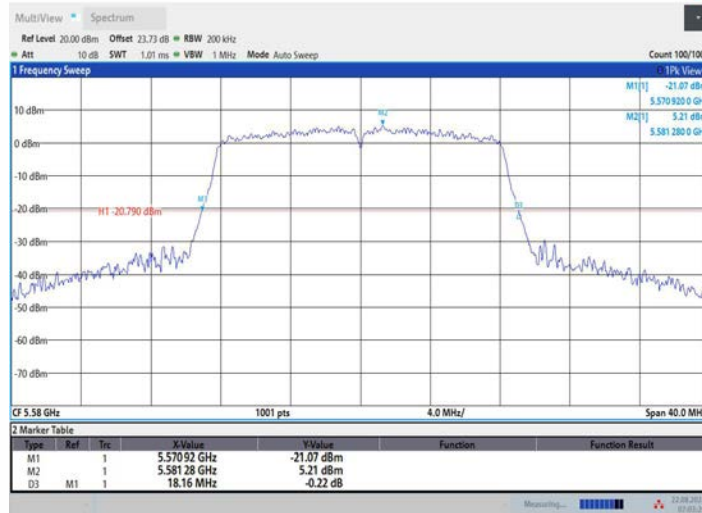
11A_Ant3_5580
