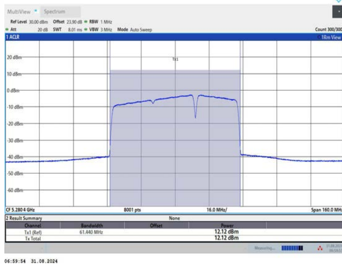
11BE80MIMO_Ant2_5290_484+242_OFDMA_1
