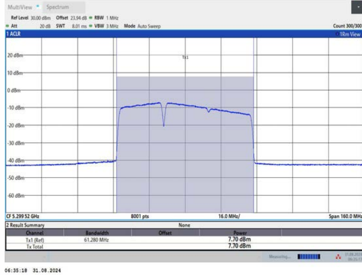
11BE80MIMO_Ant1_5290_484+242_OFDMA_1
