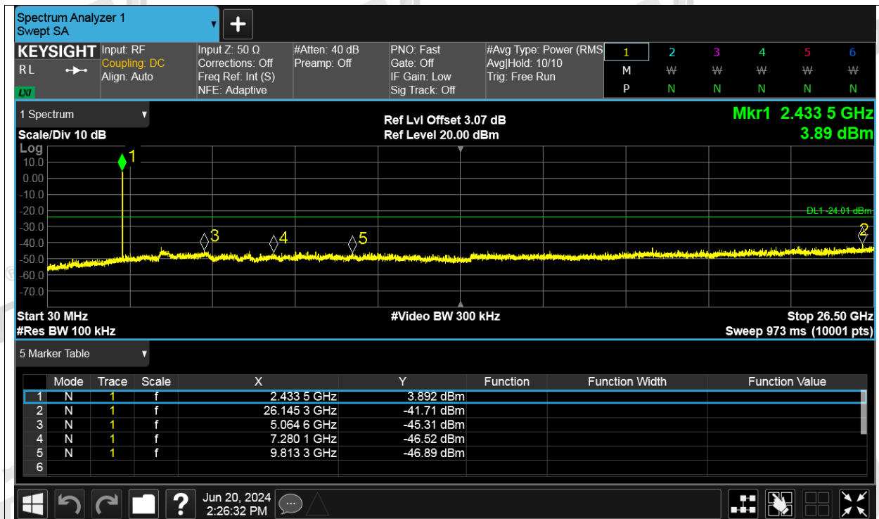
Tx. Spurious NVNT ax20 52RU Index 38 2437MHz Ant2 Ref
