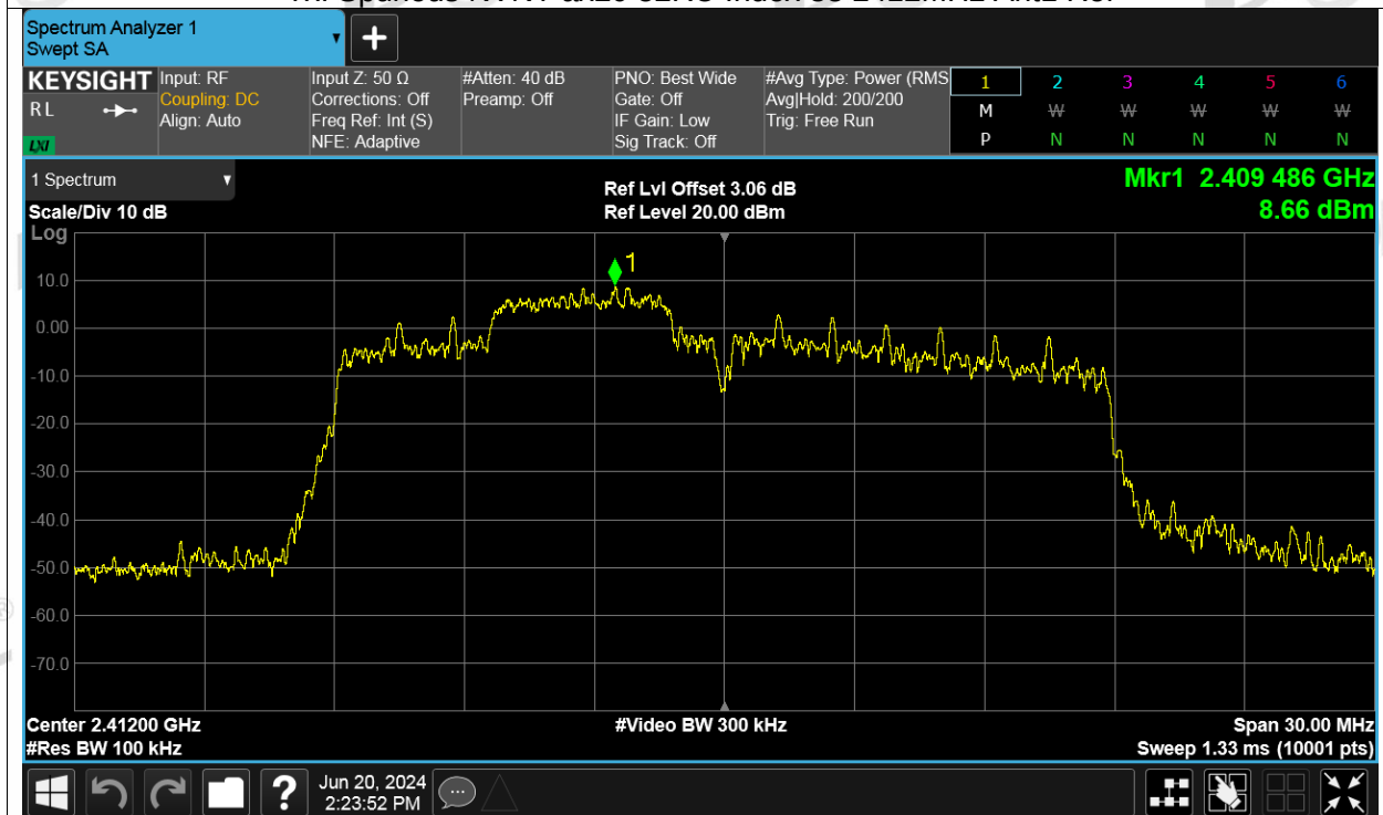
Tx. Spurious NVNT ax20 52RU Index 38 2412MHz Ant1 Emission
