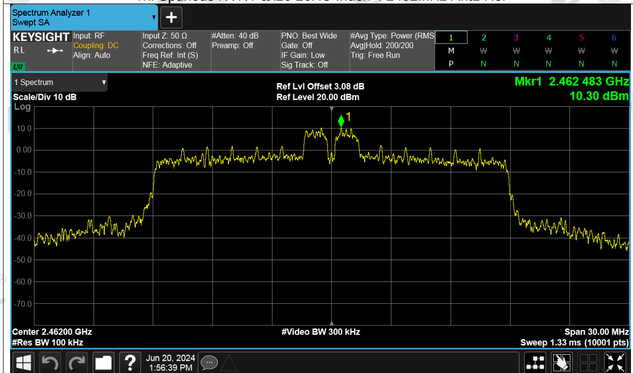
Tx. Spurious NVNT ax20 26RU Index 4 2462MHz Ant1 Emission
