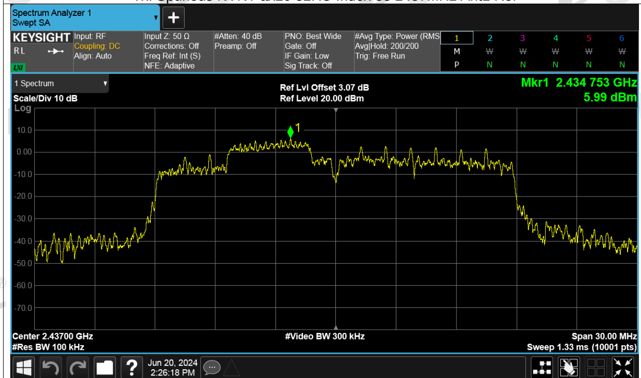
Tx. Spurious NVNT ax20 52RU Index 38 2437MHz Ant1 Emission
