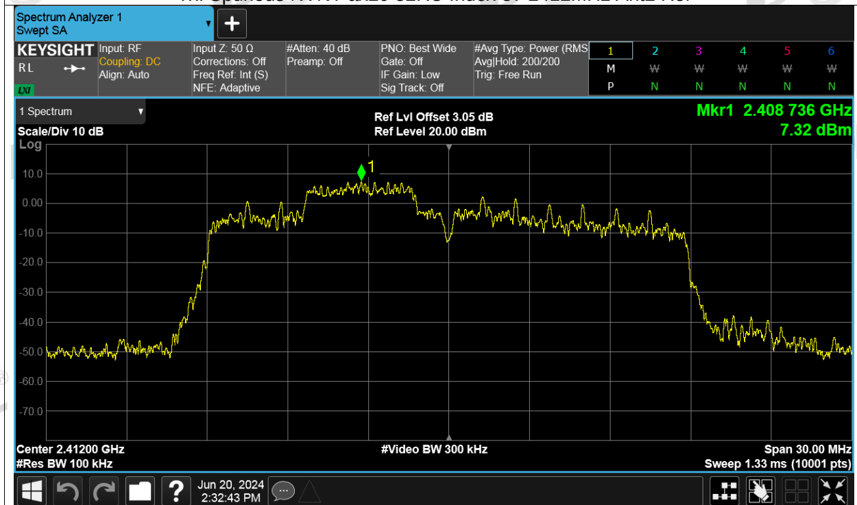
Tx. Spurious NVNT ax20 52RU Index 37 2412MHz Ant2 Emission
