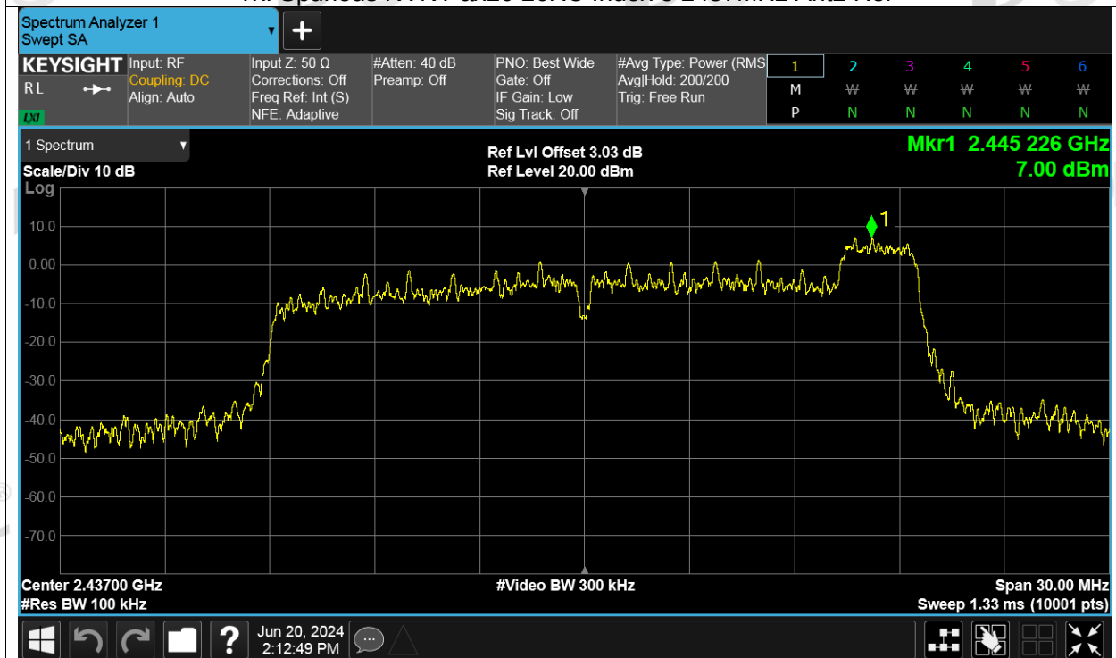
Tx. Spurious NVNT ax20 26RU Index 8 2437MHz Ant2 Emission
