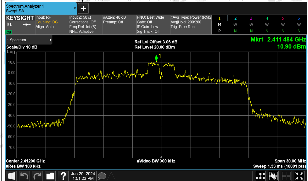
Tx. Spurious NVNT ax20 26RU Index 4 2412MHz Ant1 Emission
