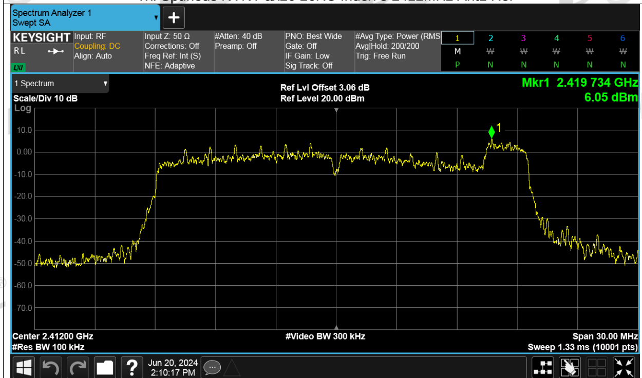
Tx. Spurious NVNT ax20 26RU Index 8 2412MHz Ant1 Emission
