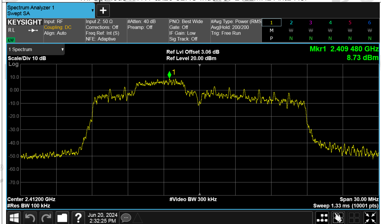
Tx. Spurious NVNT ax20 52RU Index 37 2412MHz Ant1 Emission
