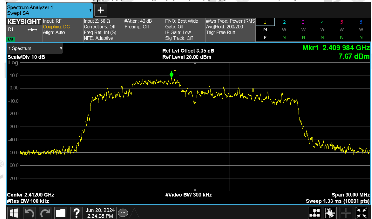
Tx. Spurious NVNT ax20 52RU Index 38 2412MHz Ant2 Emission
