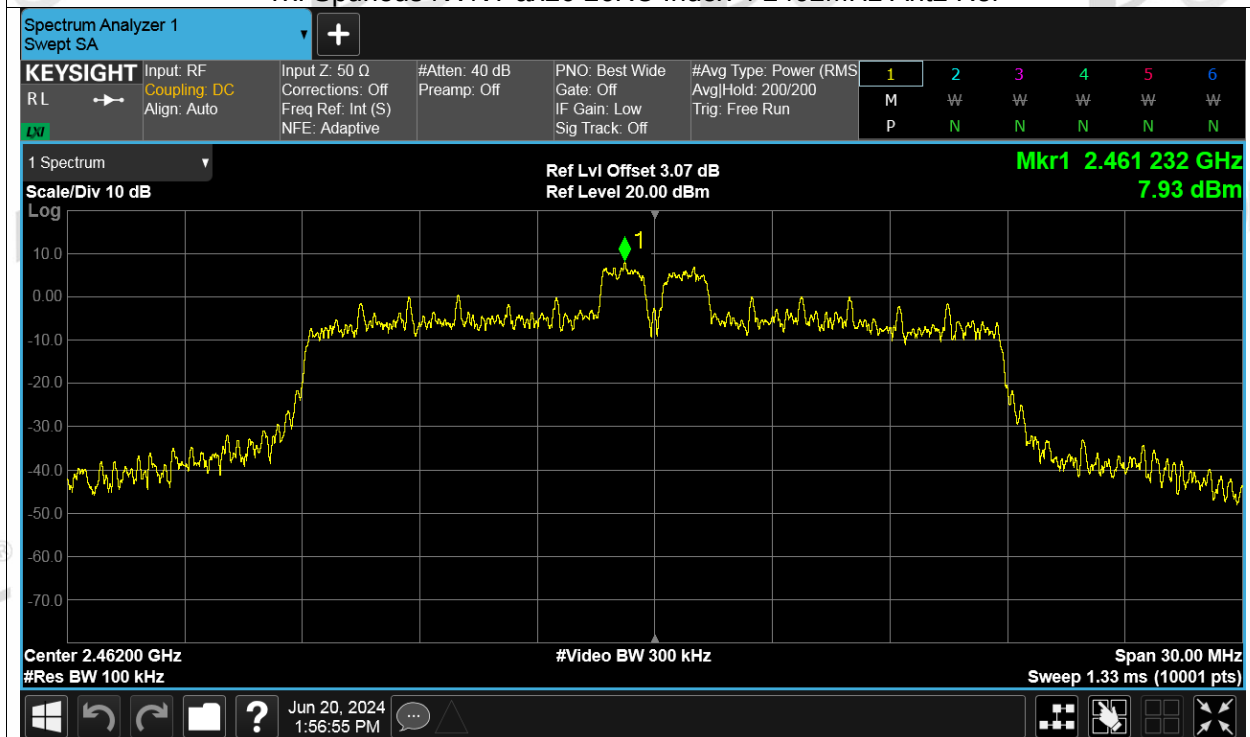
Tx. Spurious NVNT ax20 26RU Index 4 2462MHz Ant2 Emission
