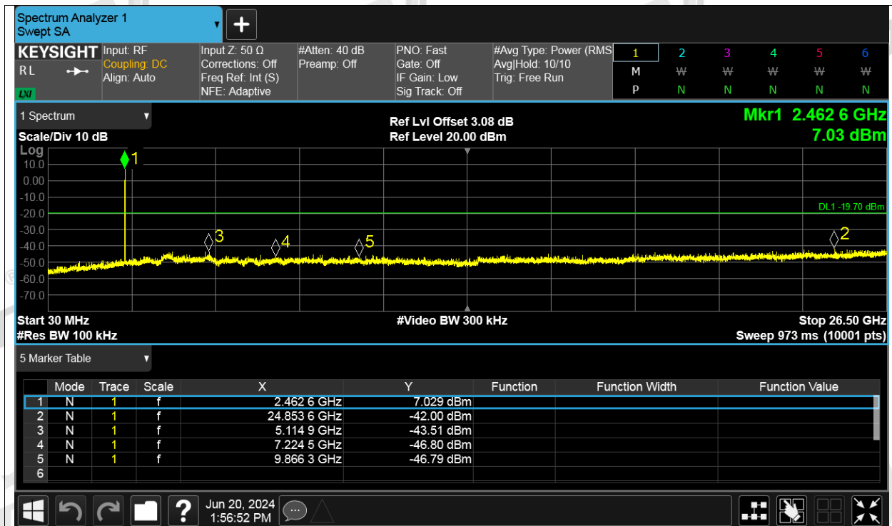
Tx. Spurious NVNT ax20 26RU Index 4 2462MHz Ant2 Ref
