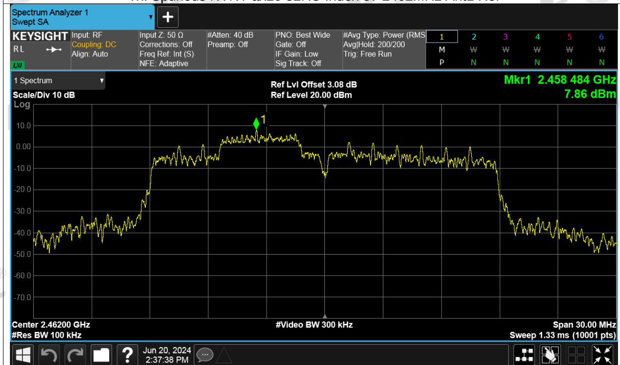
Tx. Spurious NVNT ax20 52RU Index 37 2462MHz Ant1 Emission
