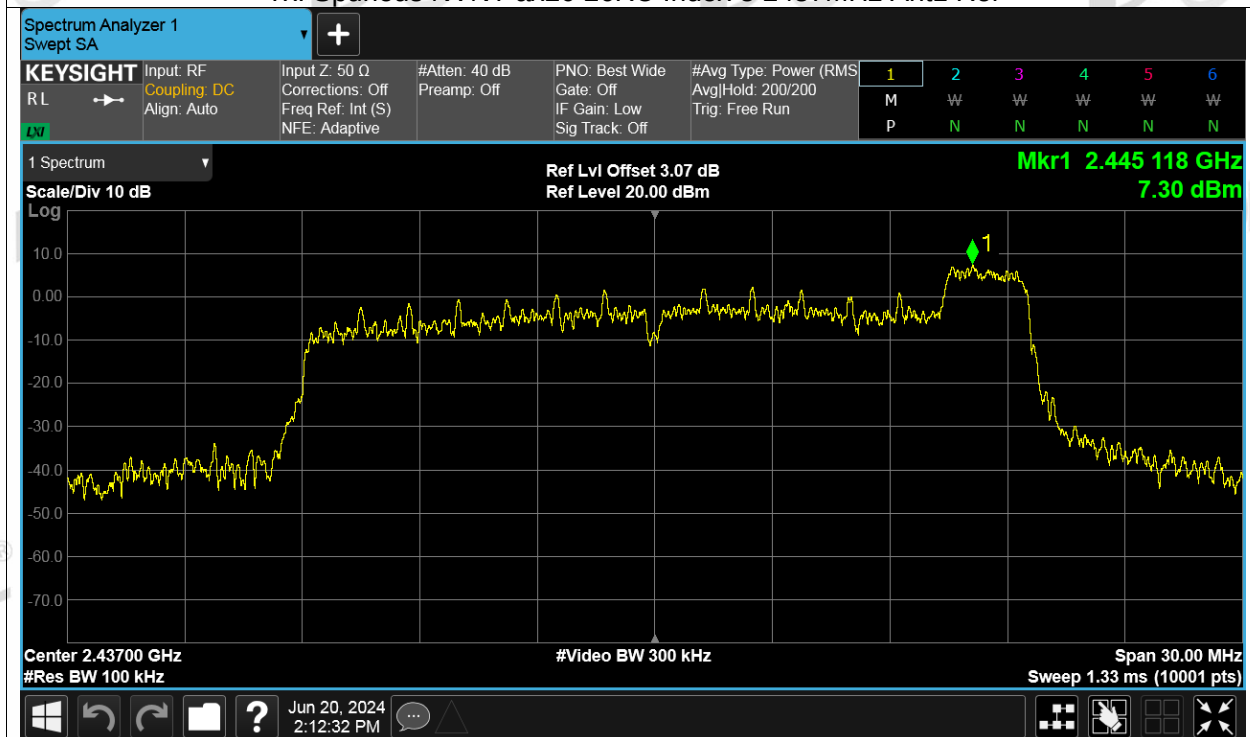
Tx. Spurious NVNT ax20 26RU Index 8 2437MHz Ant1 Emission
