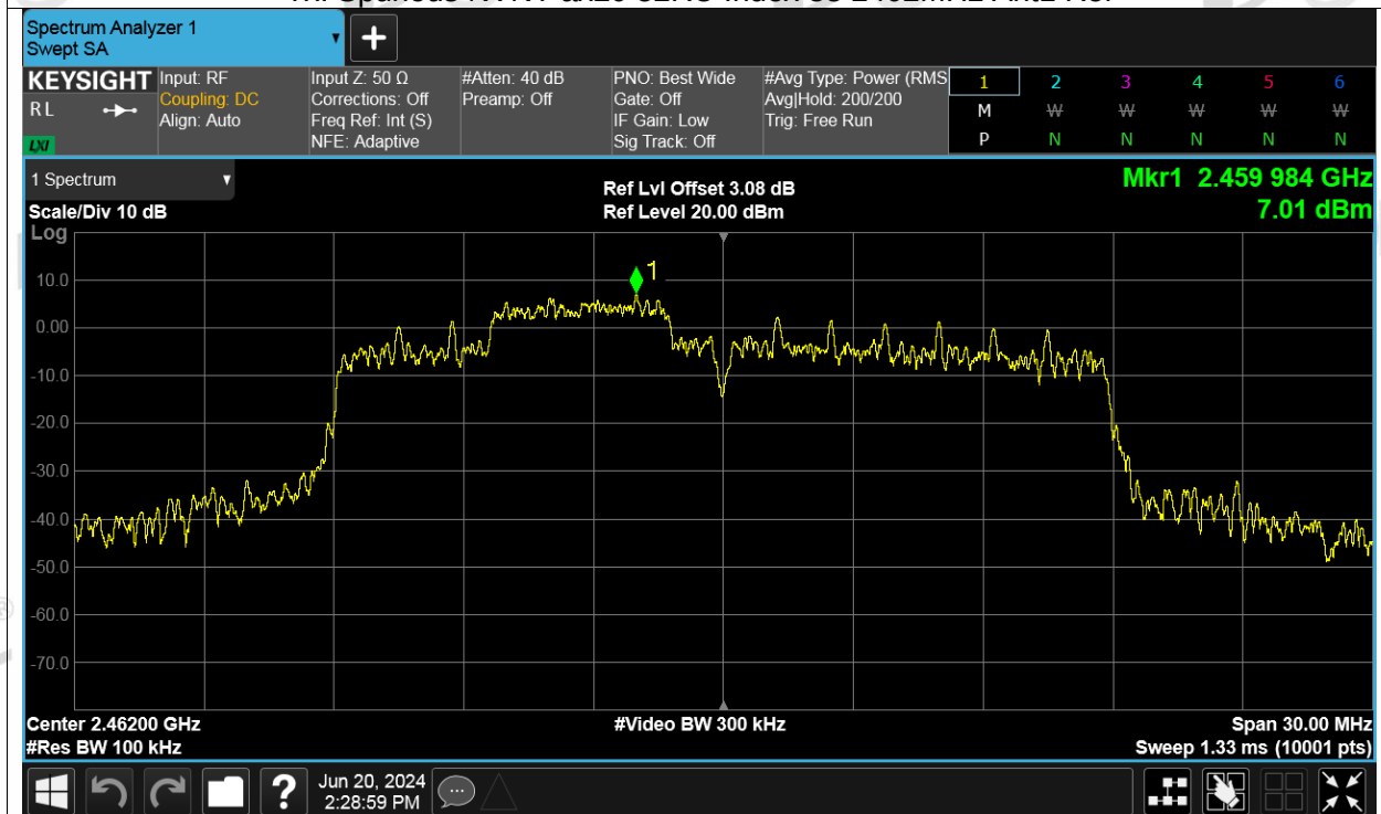
Tx. Spurious NVNT ax20 52RU Index 38 2462MHz Ant1 Emission
