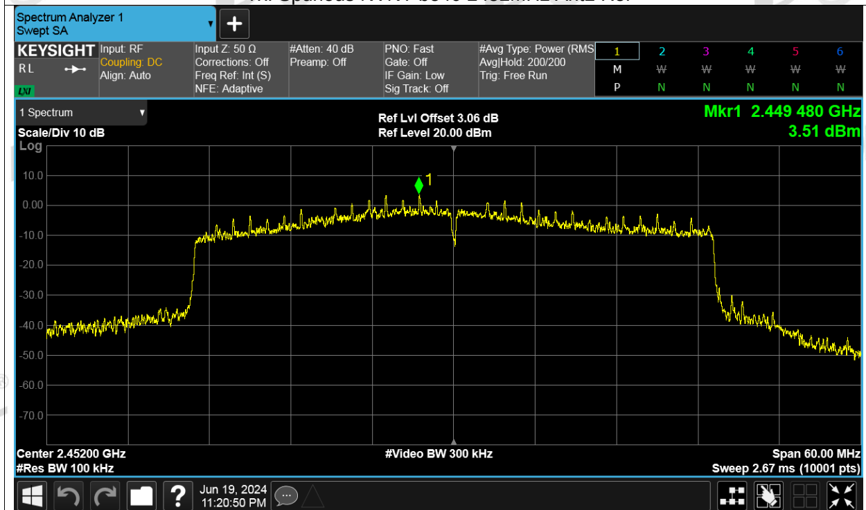
Tx. Spurious NVNT be40 2452MHz Ant2 Emission
