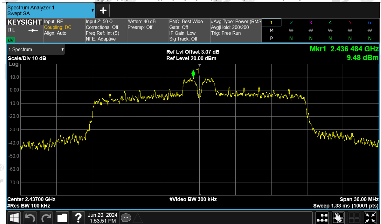
Tx. Spurious NVNT ax20 26RU Index 4 2437MHz Ant1 Emission
