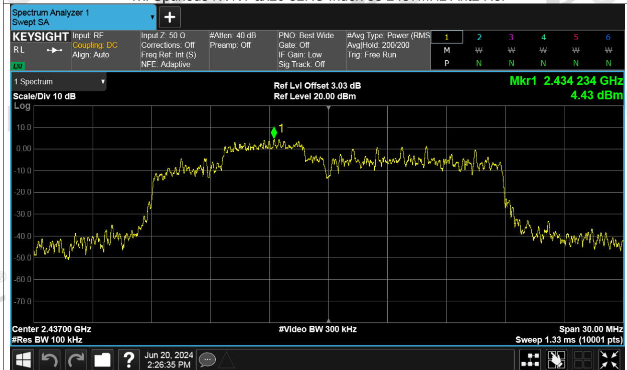
Tx. Spurious NVNT ax20 52RU Index 38 2437MHz Ant2 Emission
