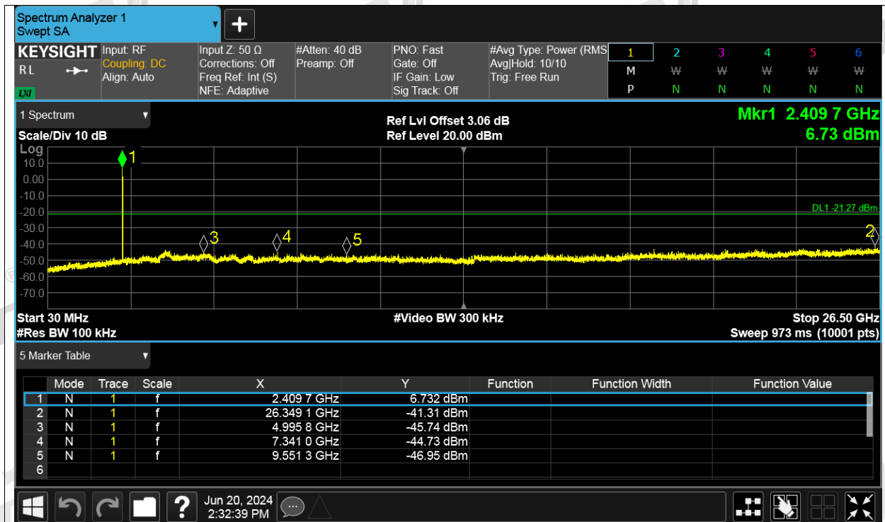
Tx. Spurious NVNT ax20 52RU Index 37 2412MHz Ant2 Ref
