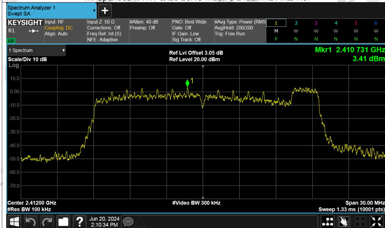
Tx. Spurious NVNT ax20 26RU Index 8 2412MHz Ant2 Emission
