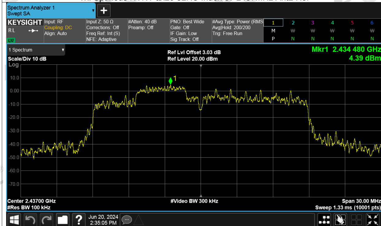
Tx. Spurious NVNT ax20 52RU Index 37 2437MHz Ant2 Emission
