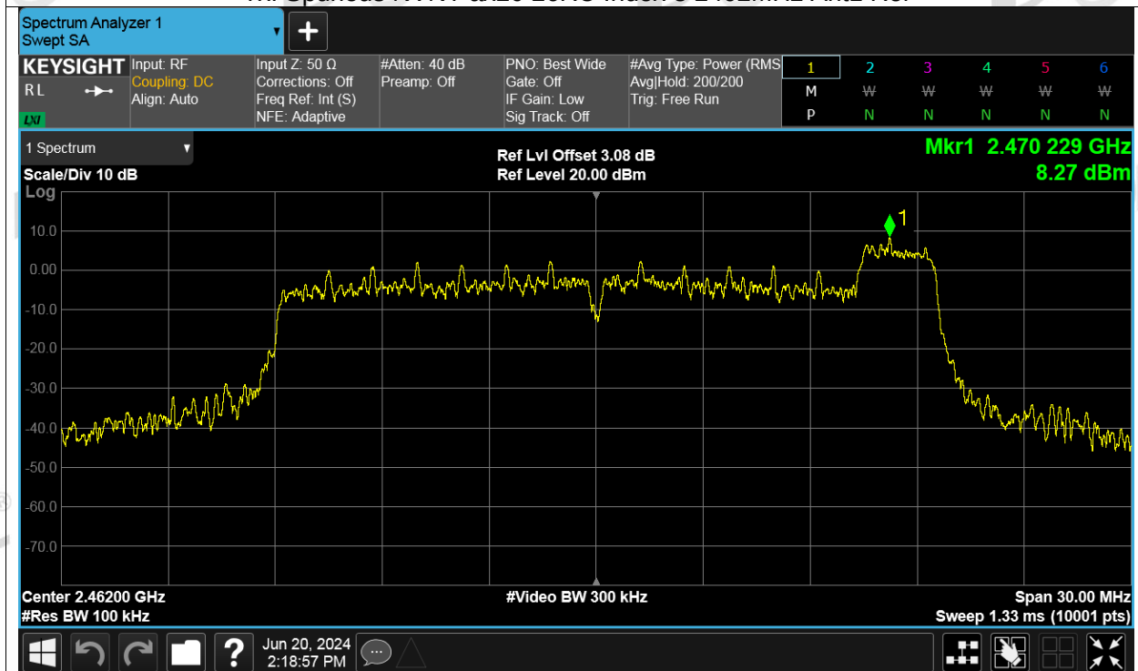
Tx. Spurious NVNT ax20 26RU Index 8 2462MHz Ant1 Emission
