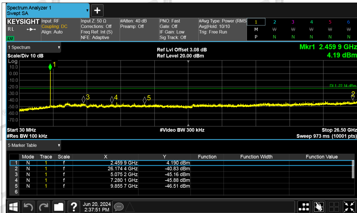
Tx. Spurious NVNT ax20 52RU Index 37 2462MHz Ant2 Ref
