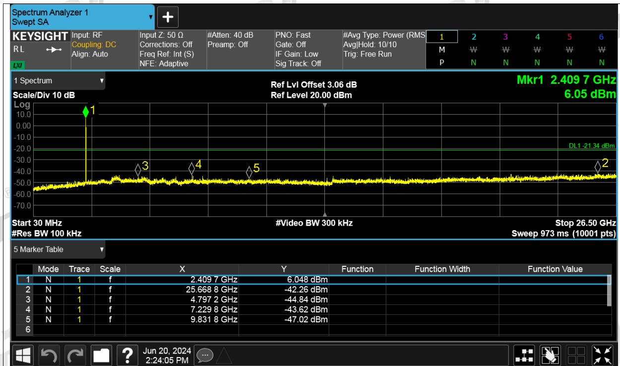
Tx. Spurious NVNT ax20 52RU Index 38 2412MHz Ant2 Ref
