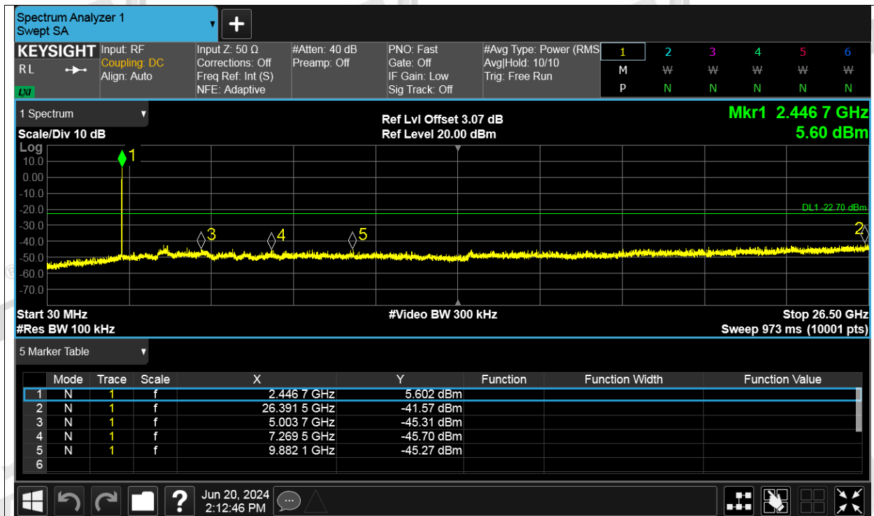
Tx. Spurious NVNT ax20 26RU Index 8 2437MHz Ant2 Ref
