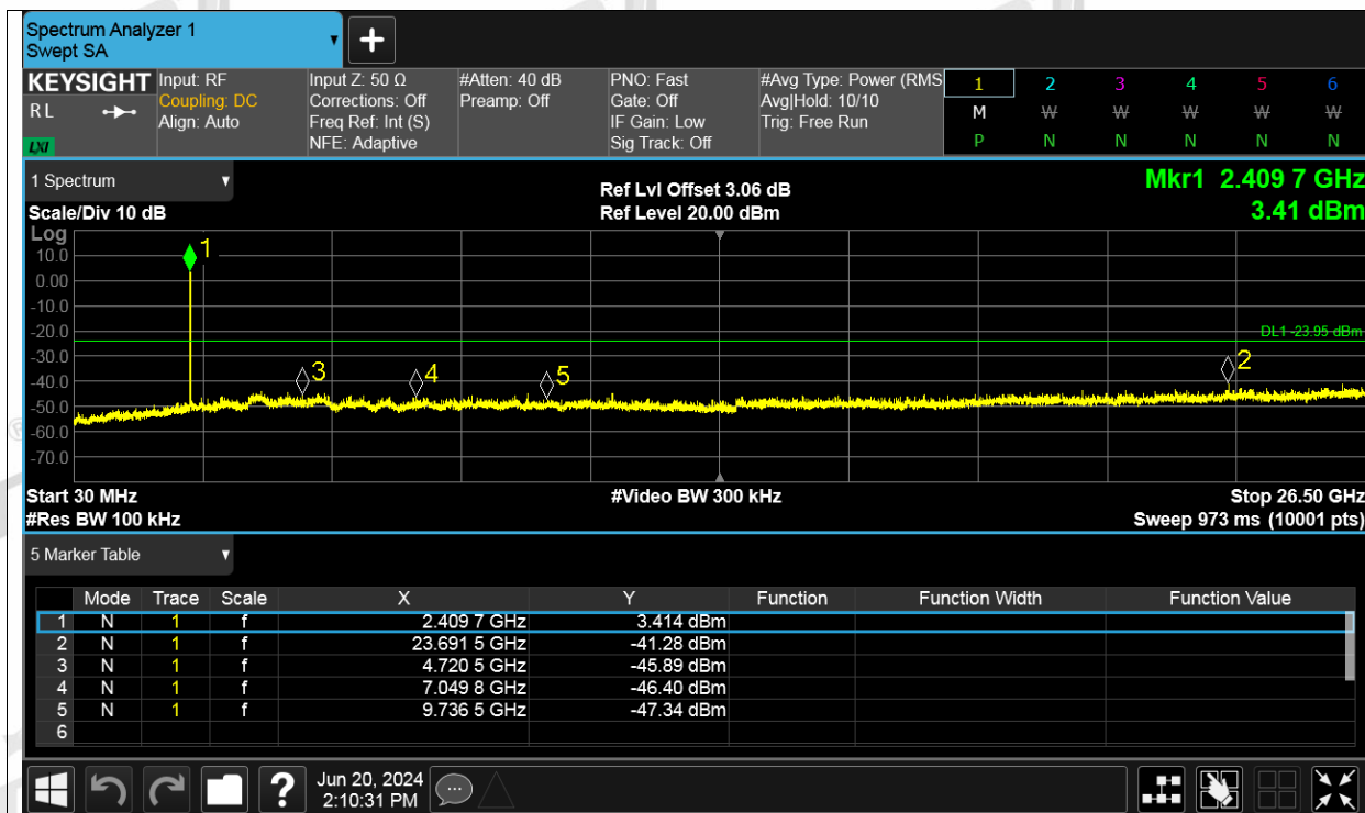
Tx. Spurious NVNT ax20 26RU Index 8 2412MHz Ant2 Ref
