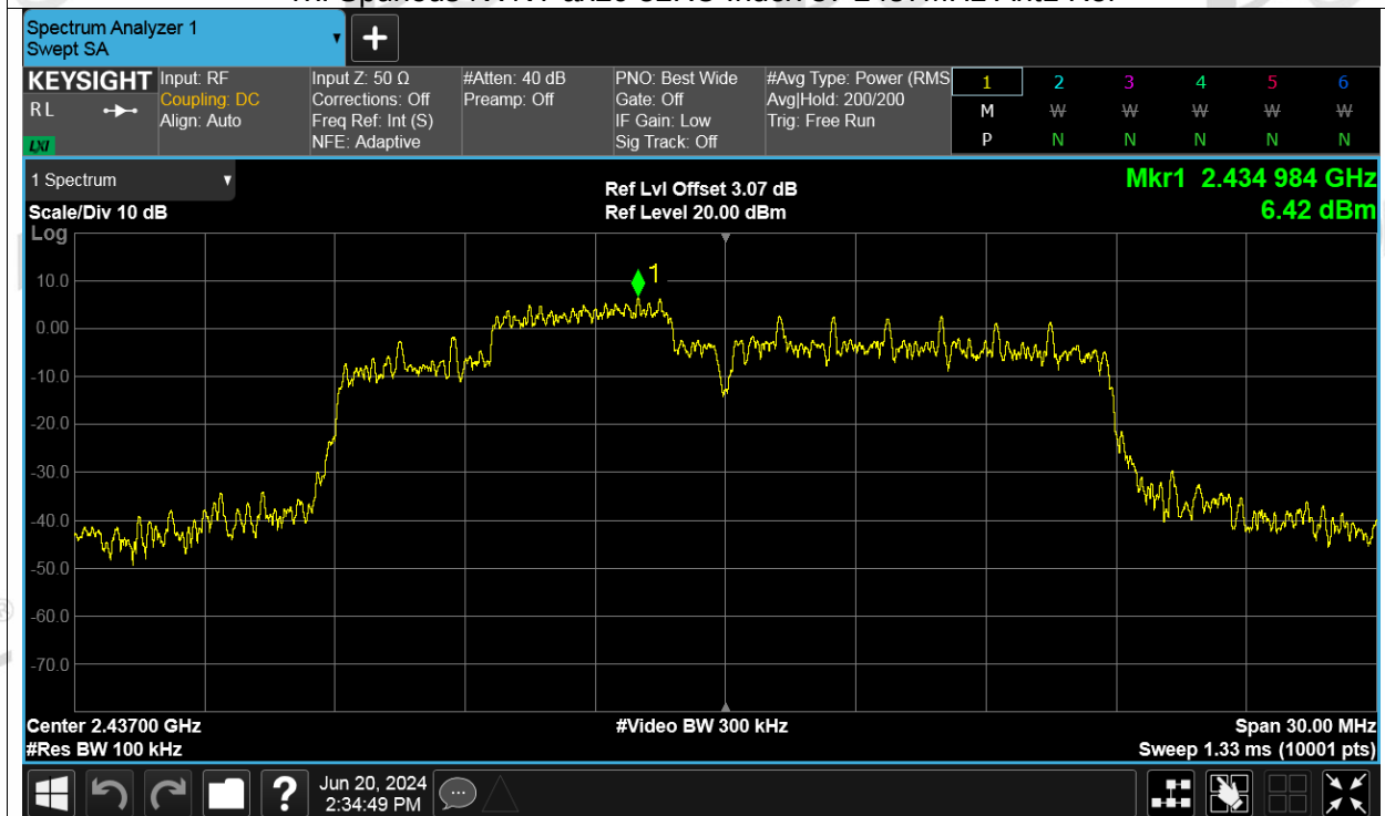
Tx. Spurious NVNT ax20 52RU Index 37 2437MHz Ant1 Emission
