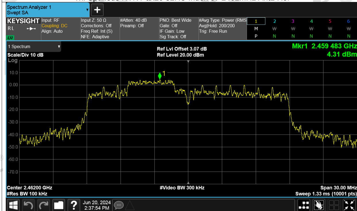
Tx. Spurious NVNT ax20 52RU Index 37 2462MHz Ant2 Emission
