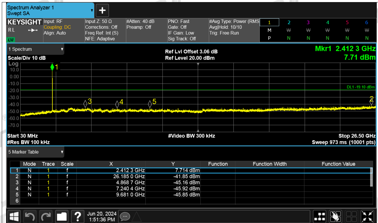
Tx. Spurious NVNT ax20 26RU Index 4 2412MHz Ant2 Ref
