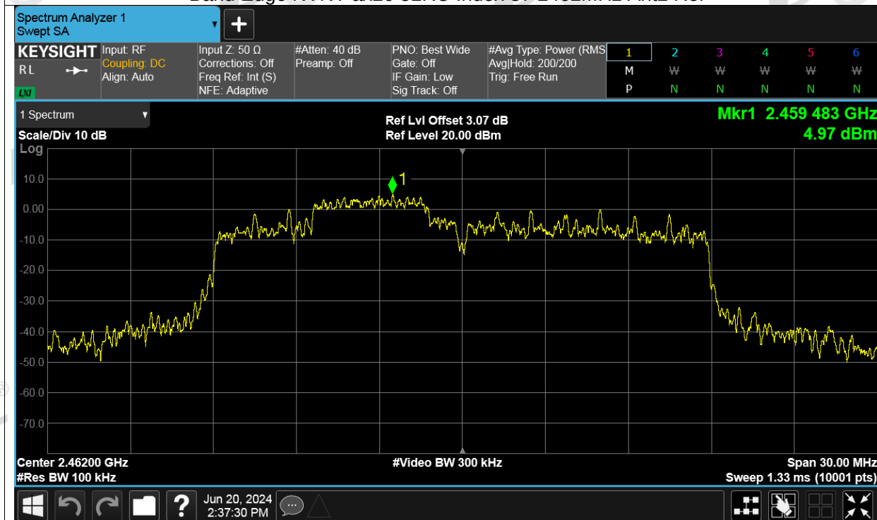
Band Edge NVNT ax20 52RU Index 37 2462MHz Ant2 Emission
