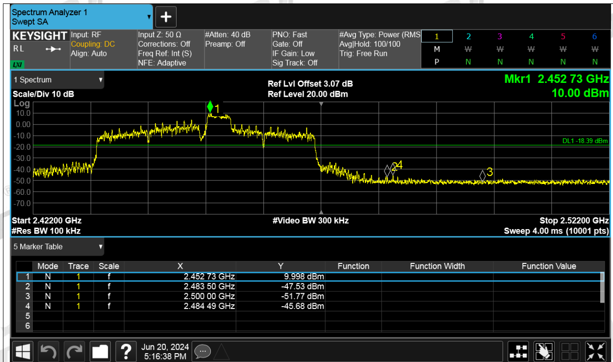
Band Edge NVNT ax40 52RU Index 41 2452MHz Ant2 Ref
