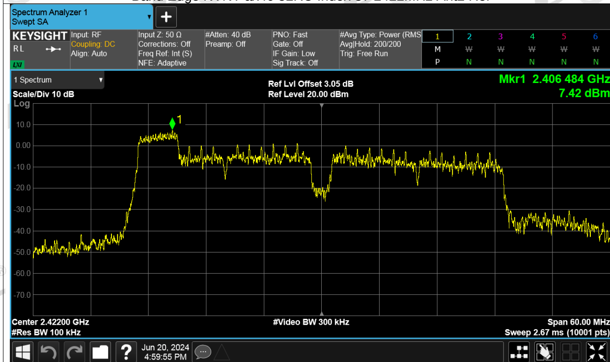
Band Edge NVNT ax40 52RU Index 37 2422MHz Ant2 Emission
