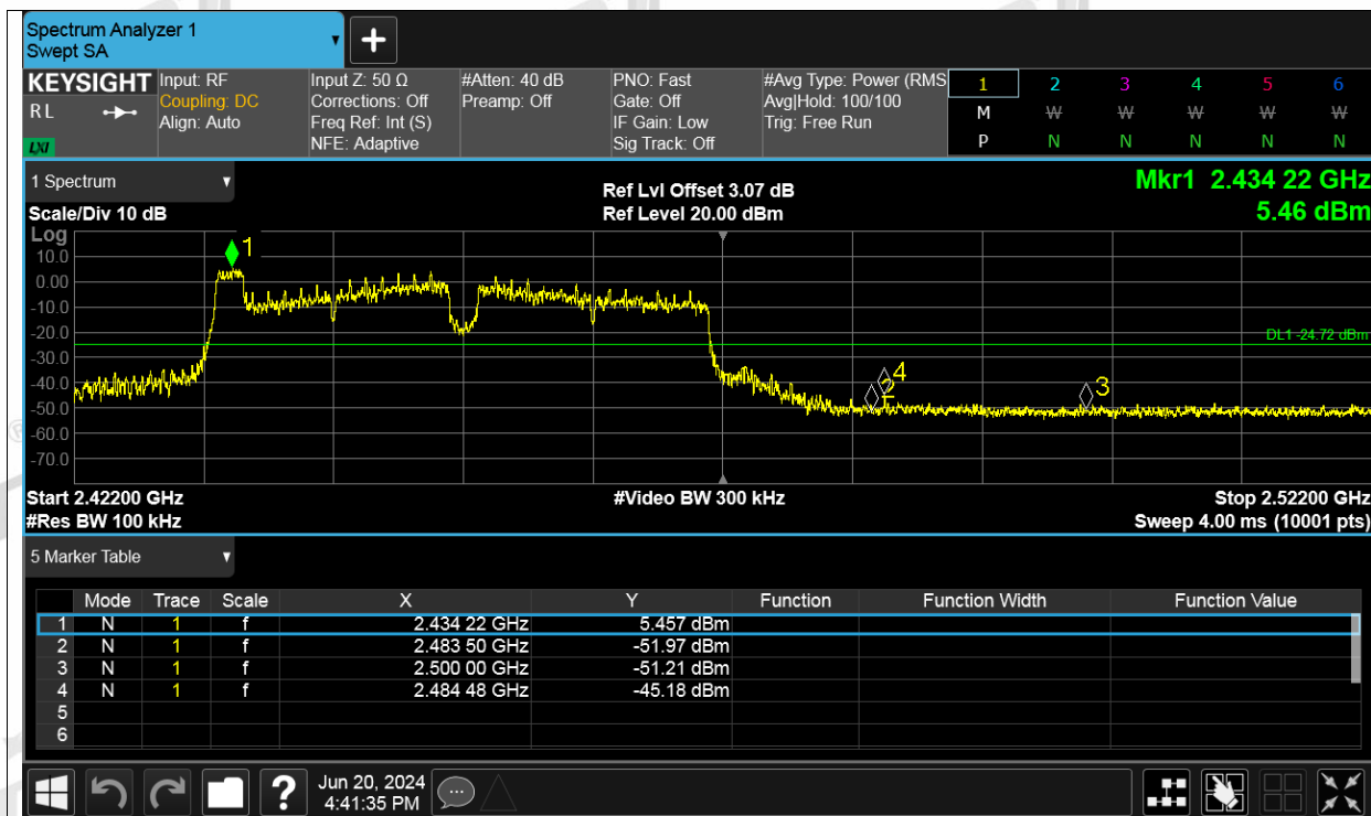
Band Edge NVNT ax40 26RU Index 0 2452MHz Ant2 Ref
