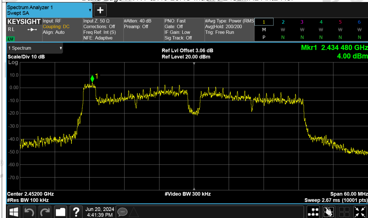
Band Edge NVNT ax40 26RU Index 0 2452MHz Ant2 Emission
