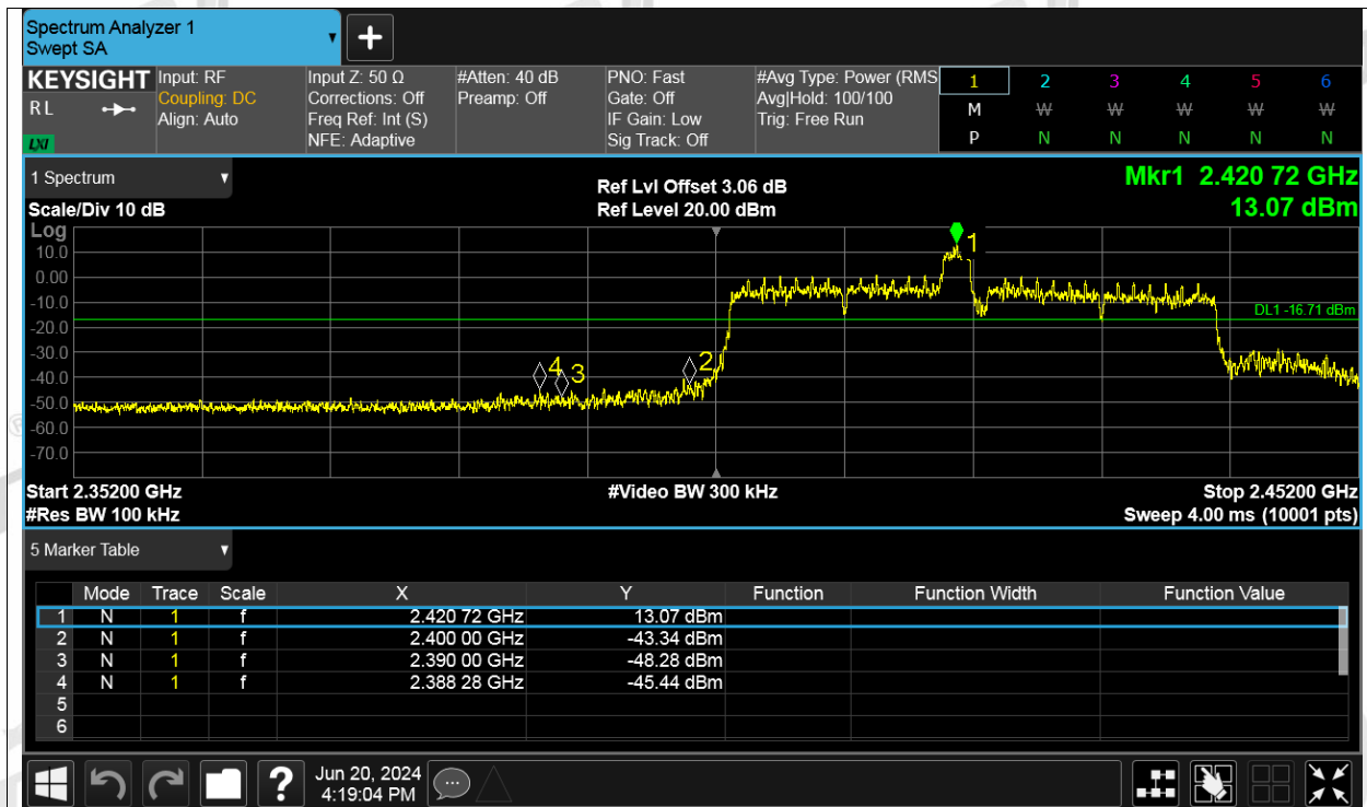
Band Edge NVNT ax40 26RU Index 8 2422MHz Ant2 Ref
