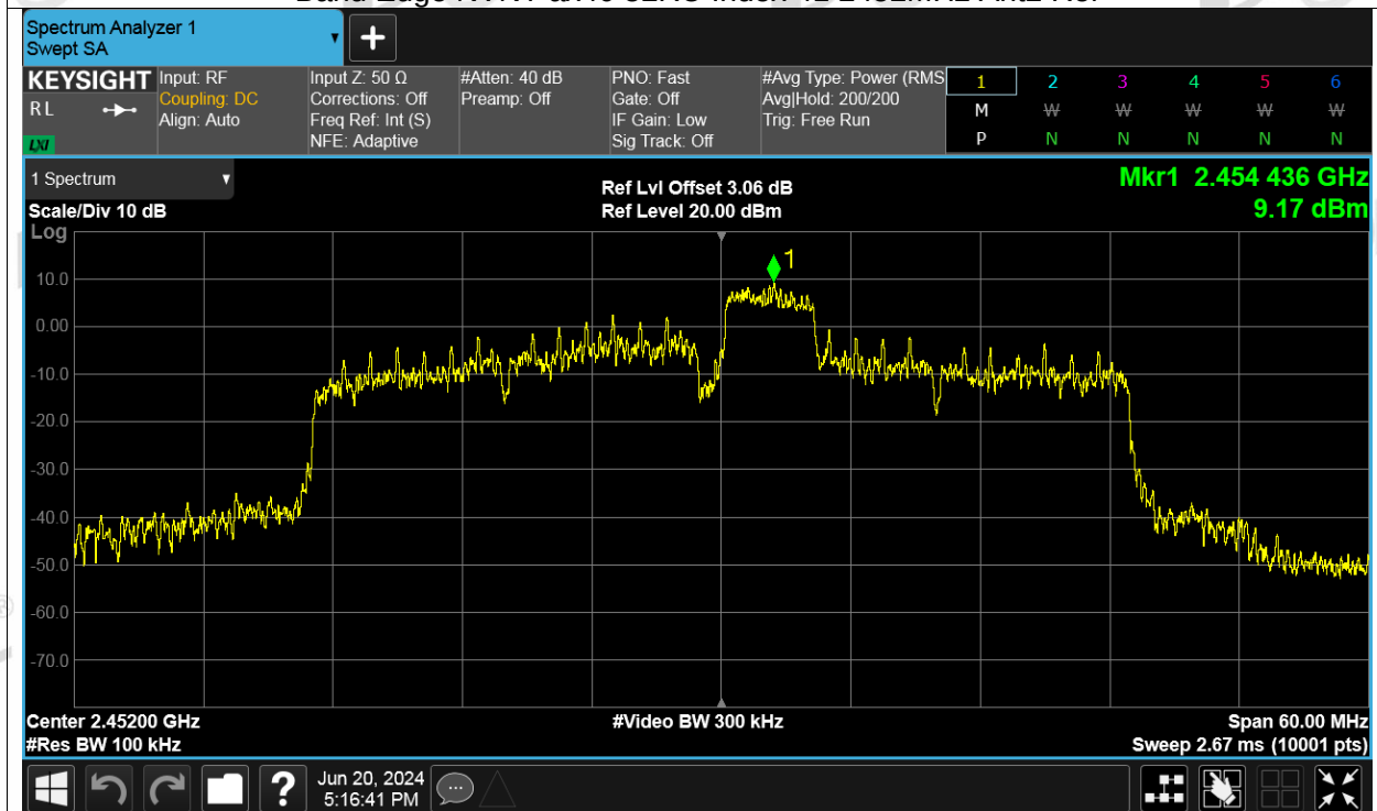
Band Edge NVNT ax40 52RU Index 41 2452MHz Ant2 Emission
