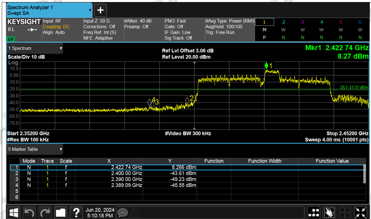
Band Edge NVNT ax40 52RU Index 41 2422MHz Ant2 Ref
