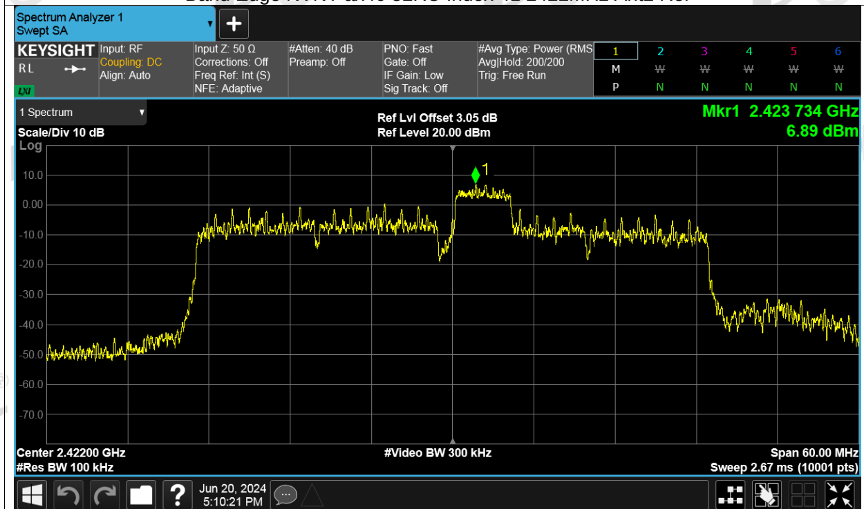
Band Edge NVNT ax40 52RU Index 41 2422MHz Ant2 Emission
