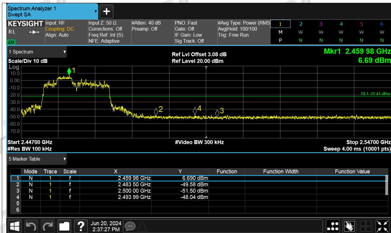
Band Edge NVNT ax20 52RU Index 37 2462MHz Ant2 Ref
