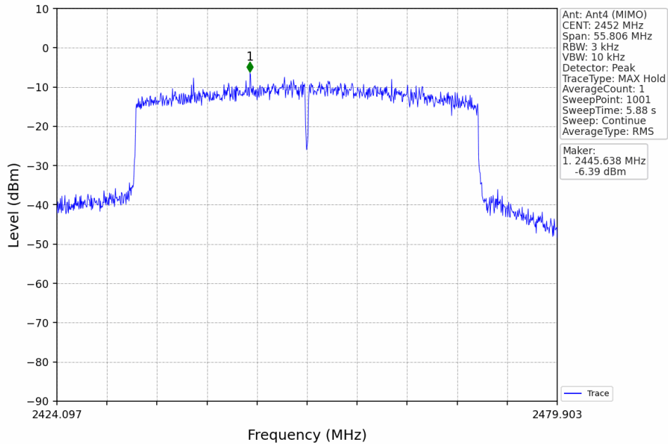
802.11ax(HEW40)_HCH_2452MHz_RU484_Left_MIMO_NTNV
