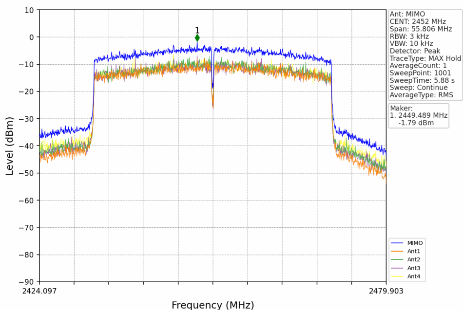
802.11ax(HEW40)_HCH_2452MHz_RU484_Left_MIMO_NTNV
