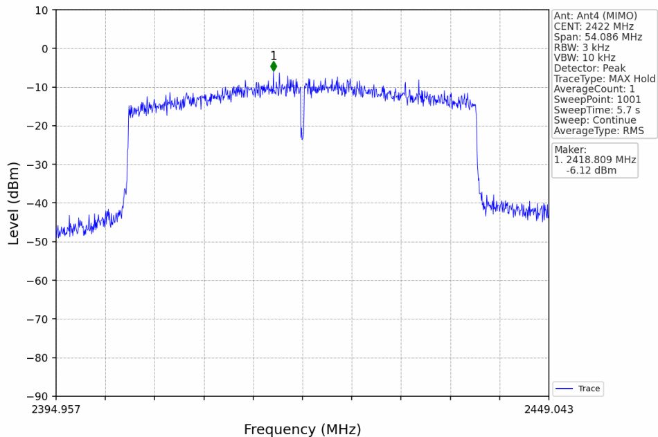
802.11ax(HEW40)_LCH_2422MHz_RU484_Left_MIMO_NTNV
