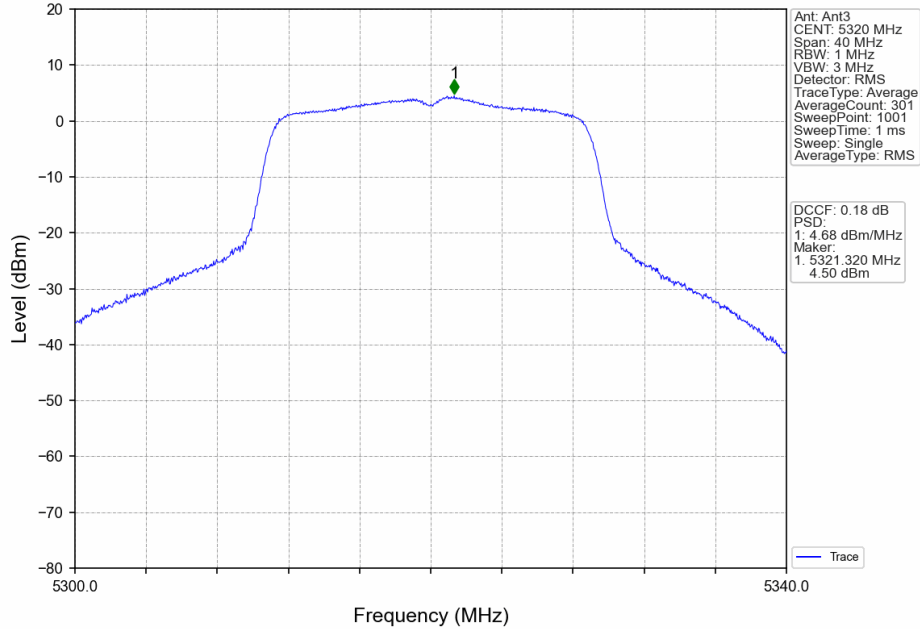
802.11ac(VHT20)_HCH_5320MHz_MIMO_NTNV
