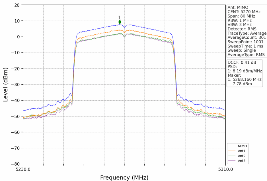
802.11ax(HEW40)_LCH_5270MHz_RU484_Left_MIMO_NTNV
