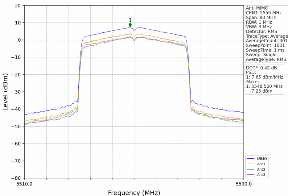
802.11ax(HEW40)_MCH_5550MHz_RU484_Left_MIMO_NTNV
