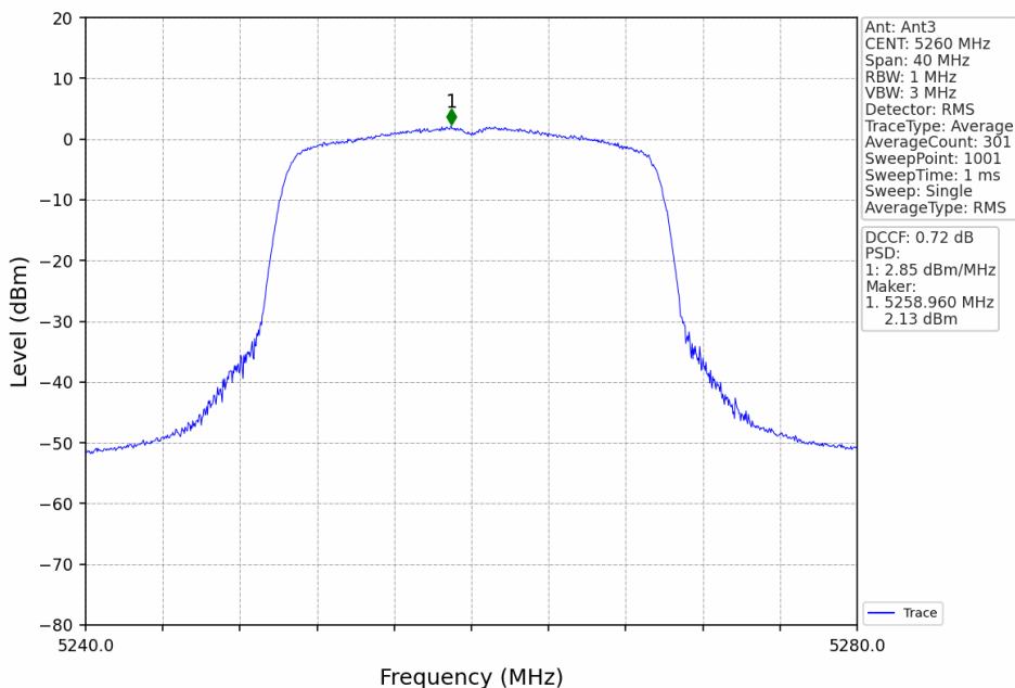
802.11ax(HEW20)_LCH_5260MHz_RU242_Left_MIMO_NTNV
