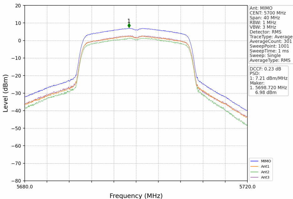
802.11ax(HEW20)_HCH_5700MHz_RU242_Left_MIMO_NTNV
