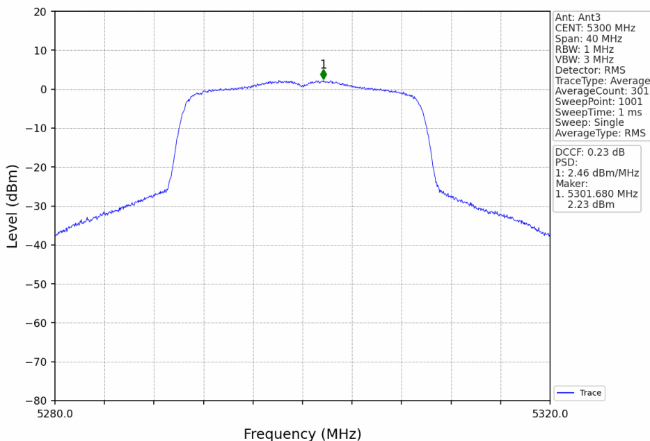
802.11ax(HEW20)_MCH_5300MHz_RU242_Left_MIMO_NTNV
