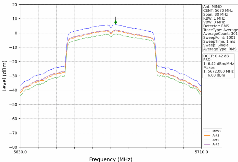
802.11ax(HEW40)_HCH_5670MHz_RU484_Left_MIMO_NTNV
