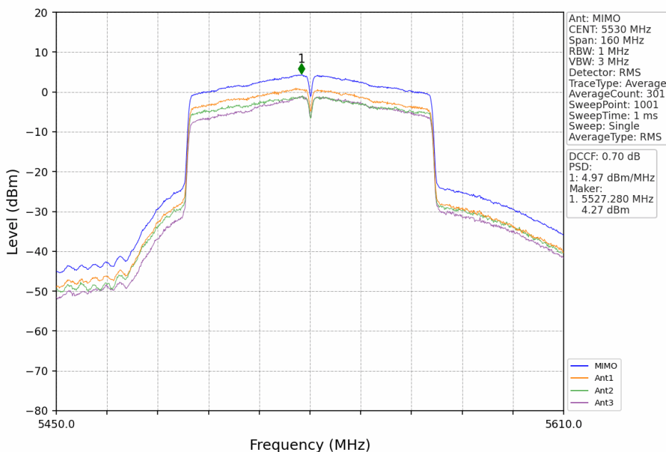
802.11ac(VHT80)_LCH_5530MHz_MIMO_NTNV
