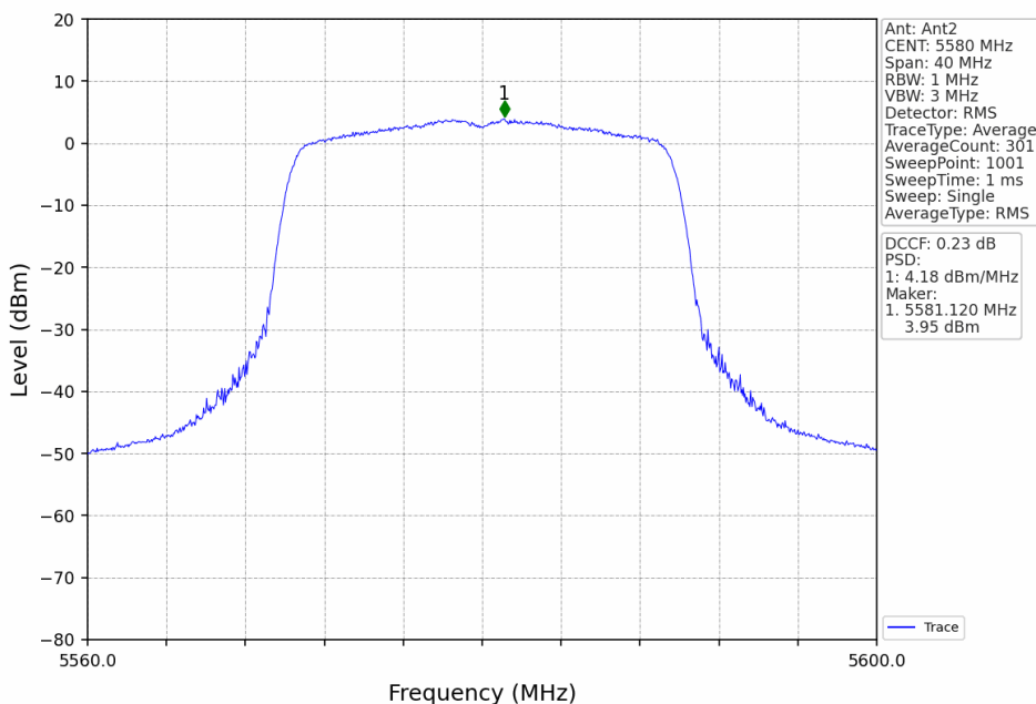
802.11ax(HEW20)_MCH_5580MHz_RU242_Left_Ant2_NTNV
