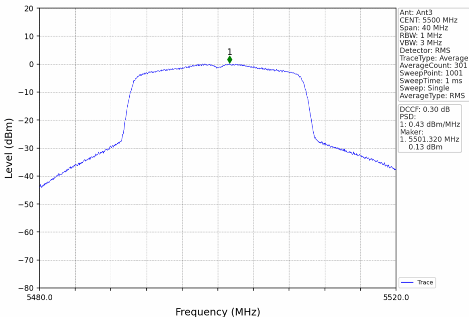
802.11ax(HEW20)_LCH_5500MHz_RU242_Left_MIMO_NTNV
