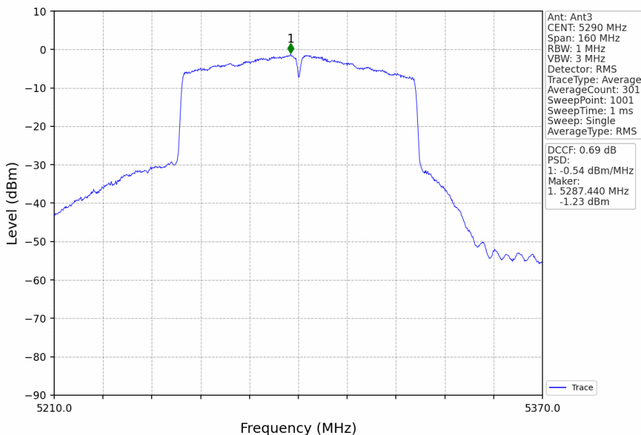
802.11ac(VHT80)_MCH_5290MHz_MIMO_NTNV
