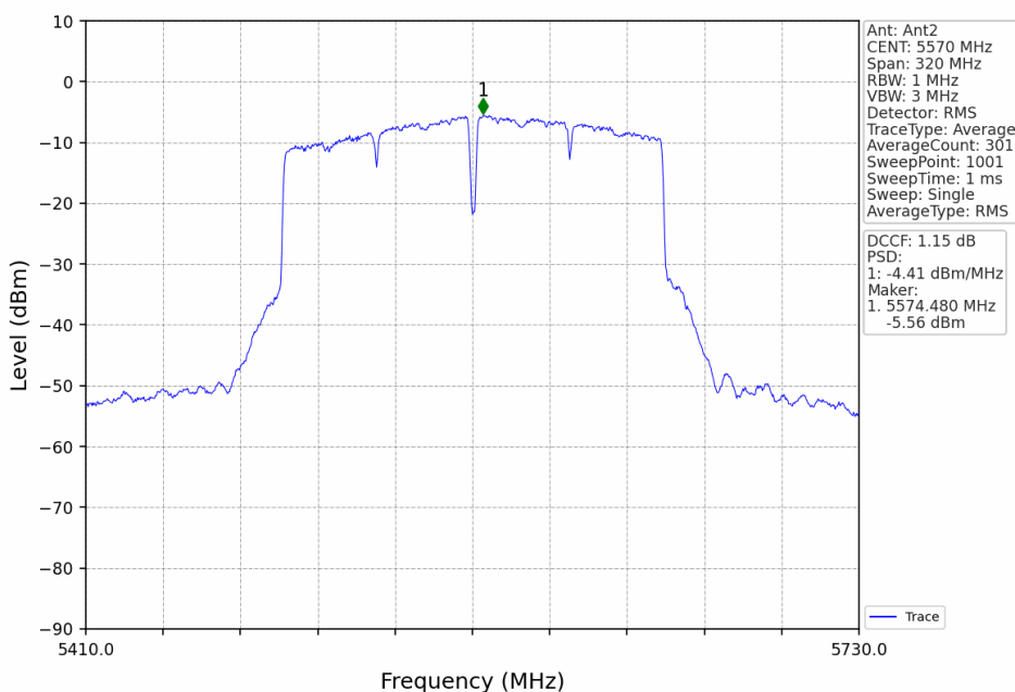
802.11ac(VHT160)_MCH_5570MHz_Ant2_NTNV
