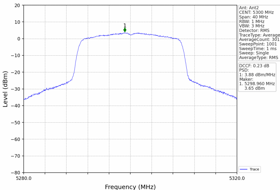
802.11ax(HEW20)_MCH_5300MHz_RU242_Left_Ant2_NTNV
