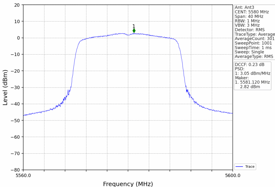
802.11ax(HEW20)_MCH_5580MHz_RU242_Left_MIMO_NTNV
