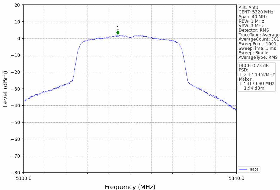
802.11ax(HEW20)_HCH_5320MHz_RU242_Left_MIMO_NTNV
