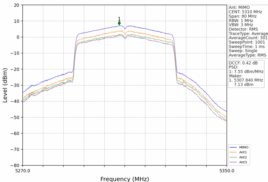
802.11ax(HEW40)_HCH_5310MHz_RU484_Left_MIMO_NTNV
