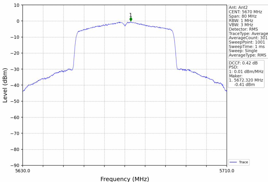
802.11ax(HEW40)_HCH_5670MHz_RU484_Left_Ant2_NTNV
