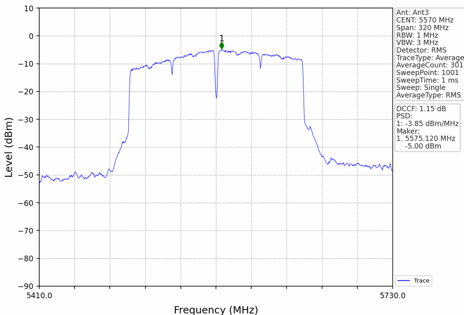
802.11ac(VHT160)_MCH_5570MHz_MIMO_NTNV
