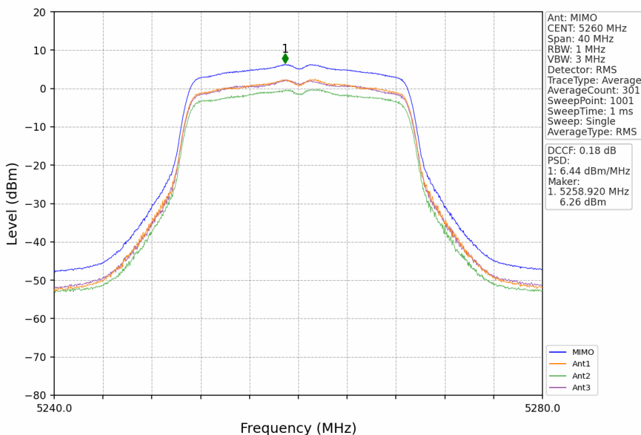
802.11n(HT20)_LCH_5260MHz_MIMO_NTNV
