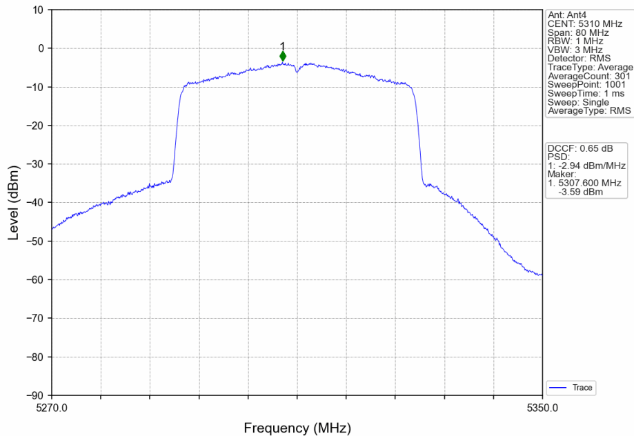
802.11ax(HEW40)_HCH_5310MHz_RU484_Left_MIMO_NTNV
