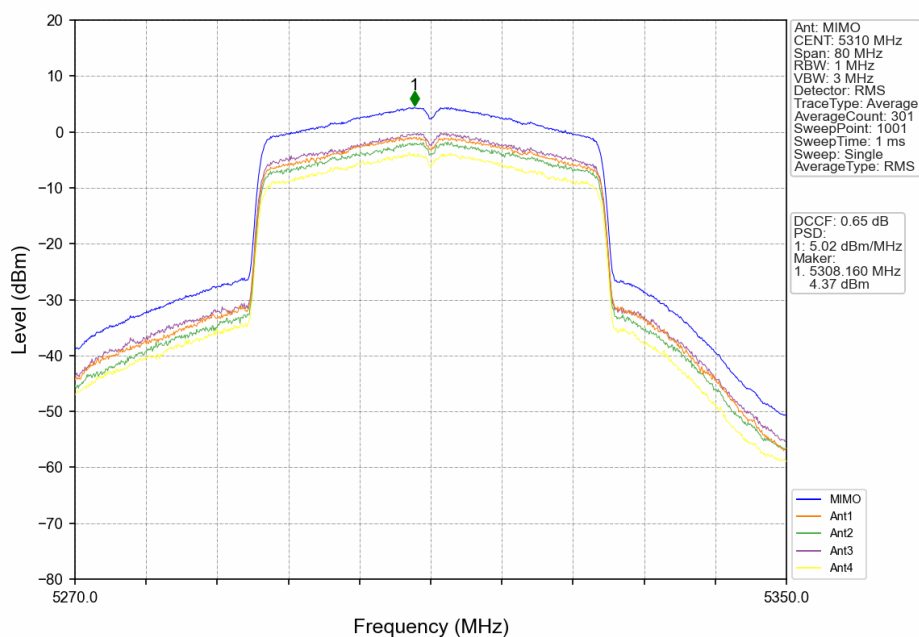
802.11ax(HEW40)_HCH_5310MHz_RU484_Left_MIMO_NTNV
