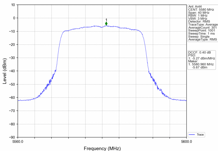
802.11ax(HEW20)_MCH_5580MHz_RU242_Left_Ant4_NTNV
