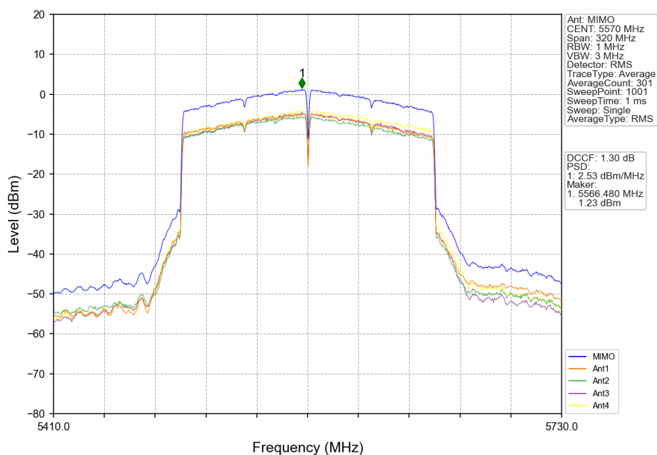
802.11ax(HEW160)_MCH_5570MHz_2xRU996_Left_MIMO_NTNV
