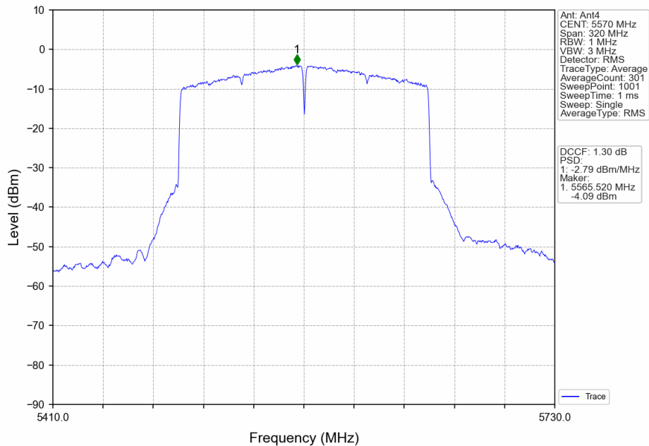
802.11ax(HEW160)_MCH_5570MHz_2xRU996_Left_MIMO_NTNV
