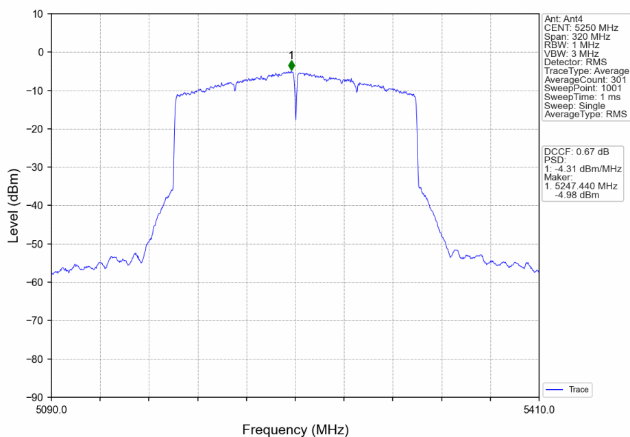
802.11ax(HEW160)_MCH_5250MHz_2xRU996_Left_Ant4_NTNV
