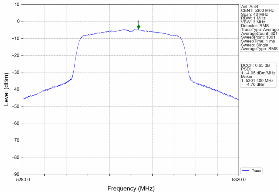
802.11ax(HEW20)_MCH_5300MHz_RU242_Left_MIMO_NTNV
