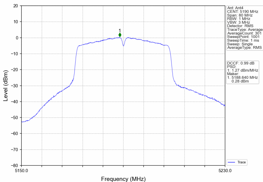
802.11ac(VHT40)_LCH_5190MHz_Ant4_NTNV
