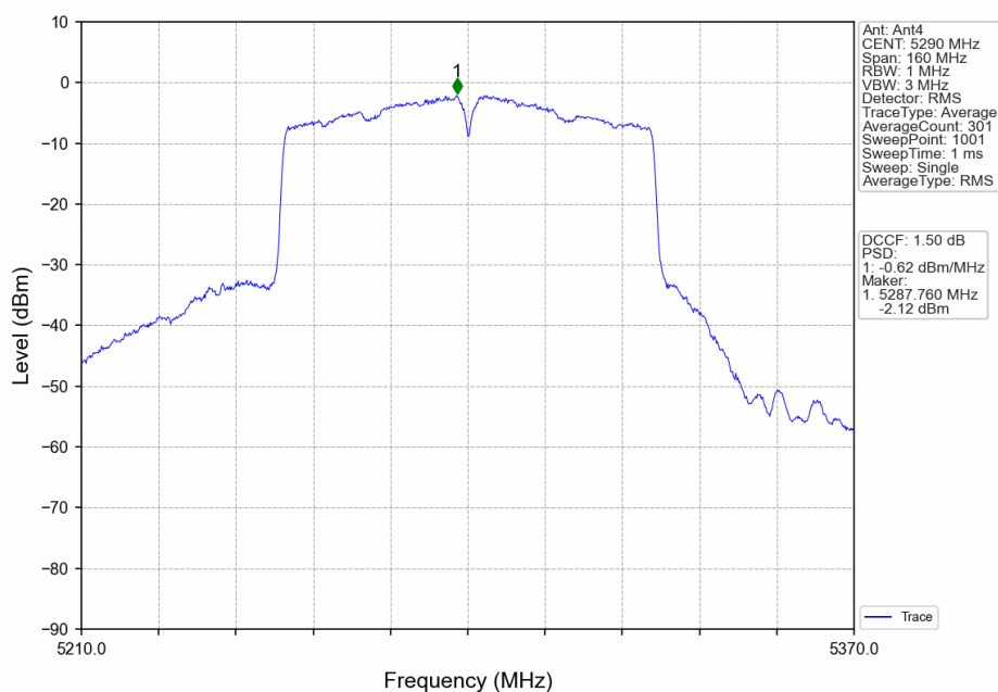
802.11ac(VHT80)_MCH_5290MHz_Ant4_NTNV
