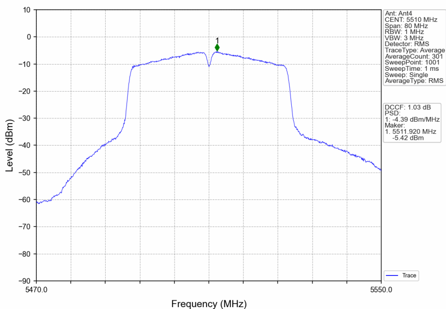
802.11ac(VHT40)_LCH_5510MHz_Ant4_NTNV
