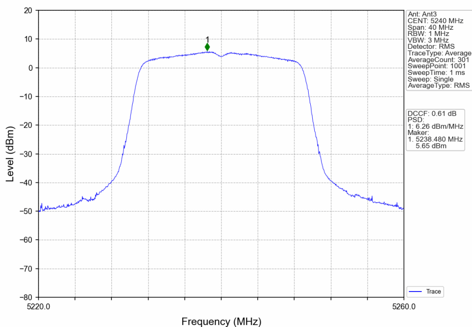
802.11ac(VHT20)_HCH_5240MHz_Ant3_NTNV
