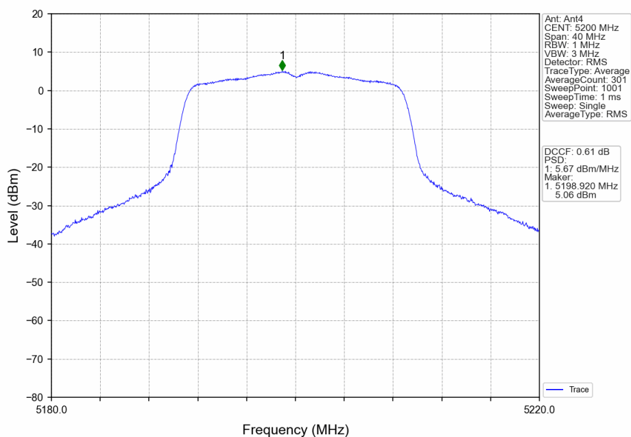
802.11ac(VHT20)_MCH_5200MHz_Ant4_NTNV
