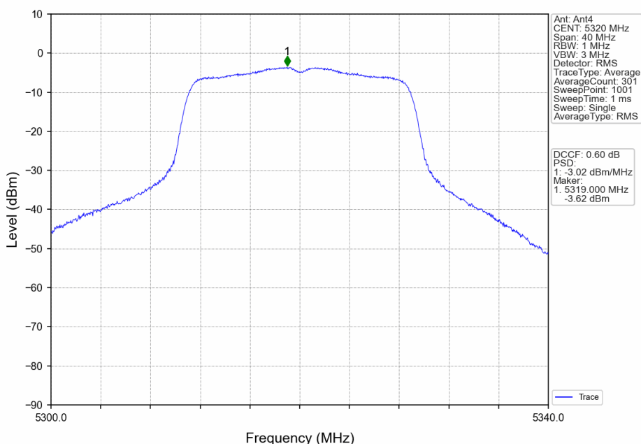
802.11ac(VHT20)_HCH_5320MHz_Ant4_NTNV
