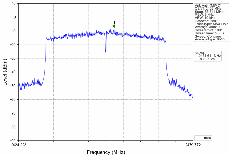
802.11ax(HEW40)_HCH_2452MHz_RU484_Left_MIMO_NTNV
