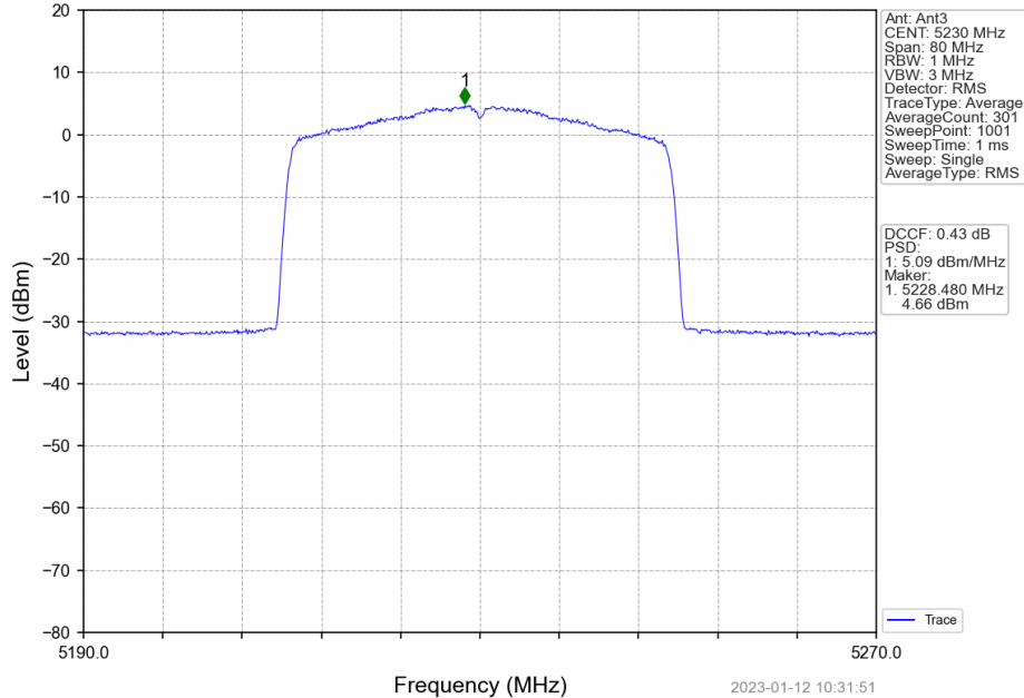
802.11ax(HEW40)_HCH_5230MHz_RU484_Left_MIMO_NTNV
