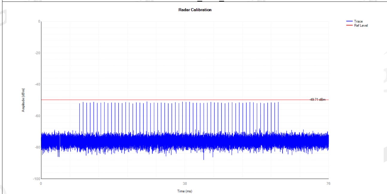
5530MHz DFS_FCC_T2000
