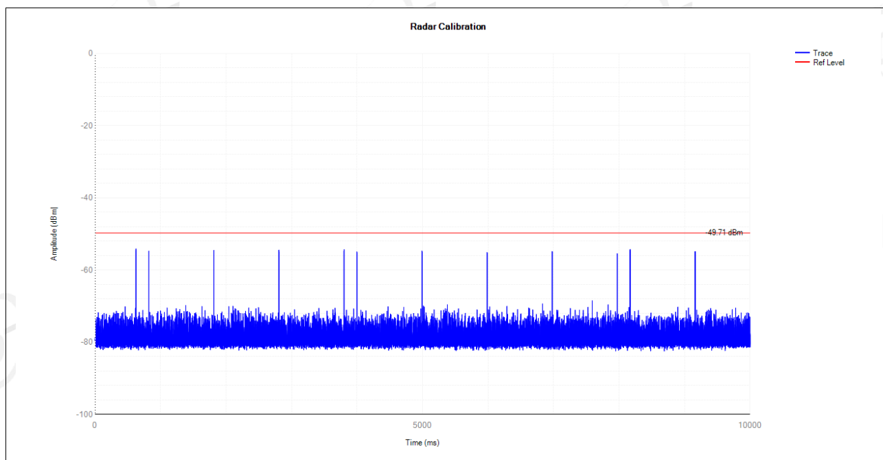
5310MHz DFS_FCC_T6000
