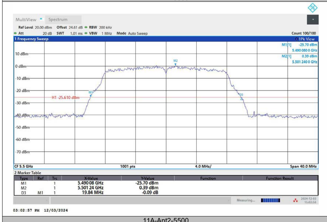
11A-Ant2-5500
