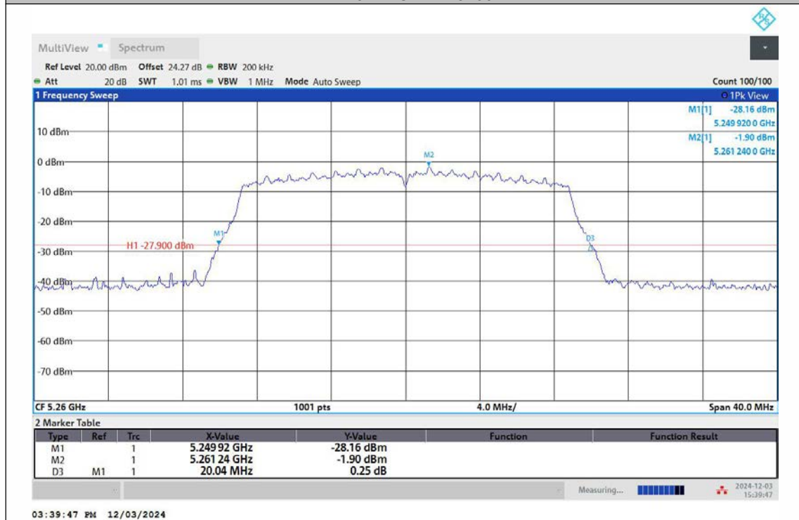
11N20MIMO-Ant2-5260
