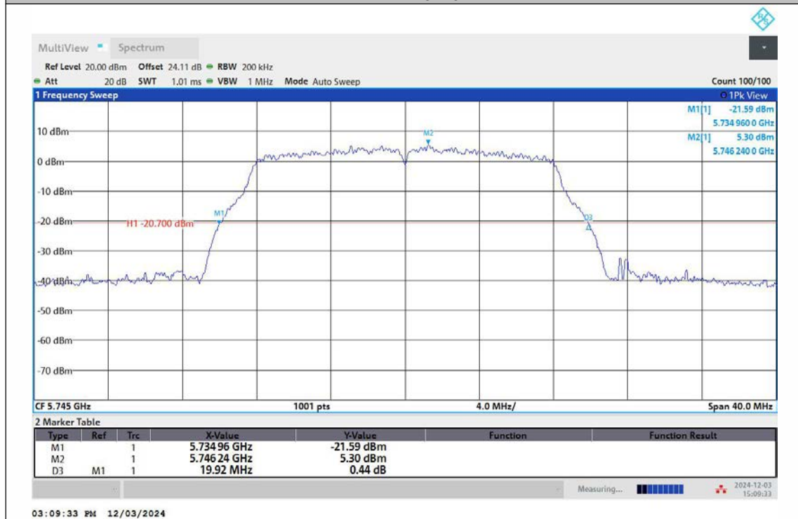
11A-Ant2-5745
