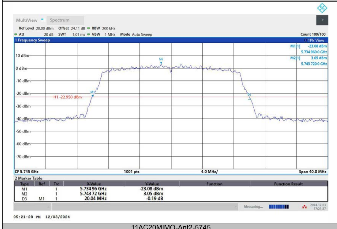
11AC20MIMO-Ant2-5745
