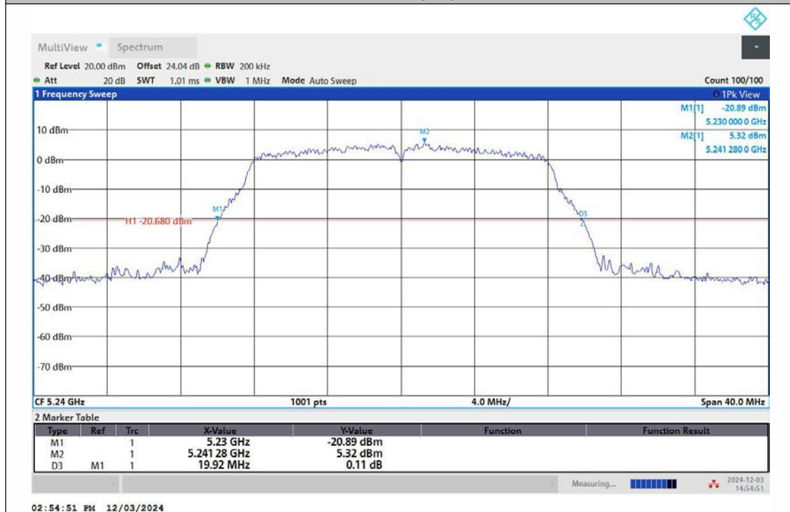
11A-Ant2-5240
