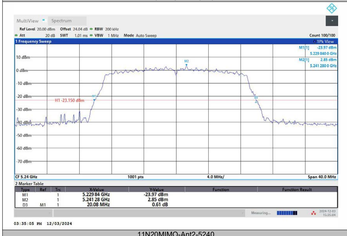
11N20MIMO-Ant2-5240
