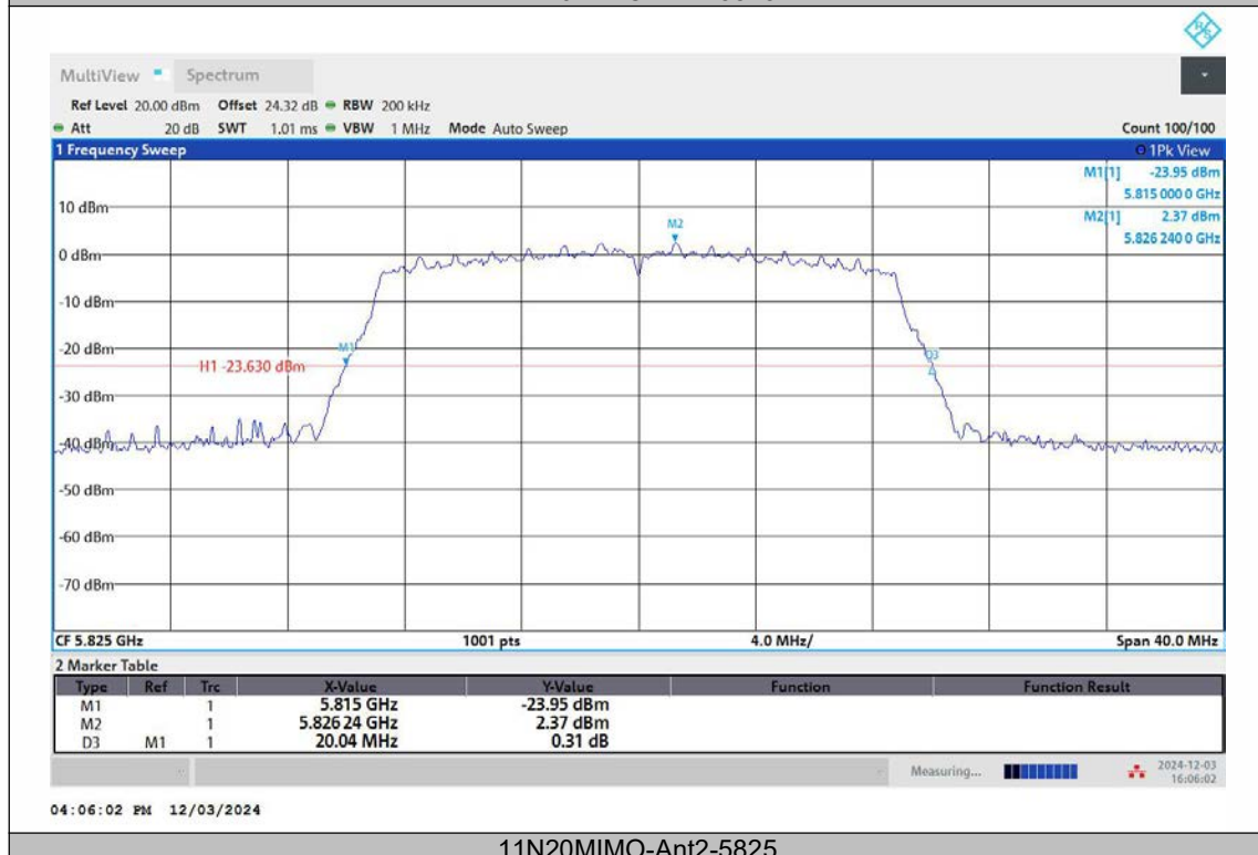
11N20MIMO-Ant2-5825
