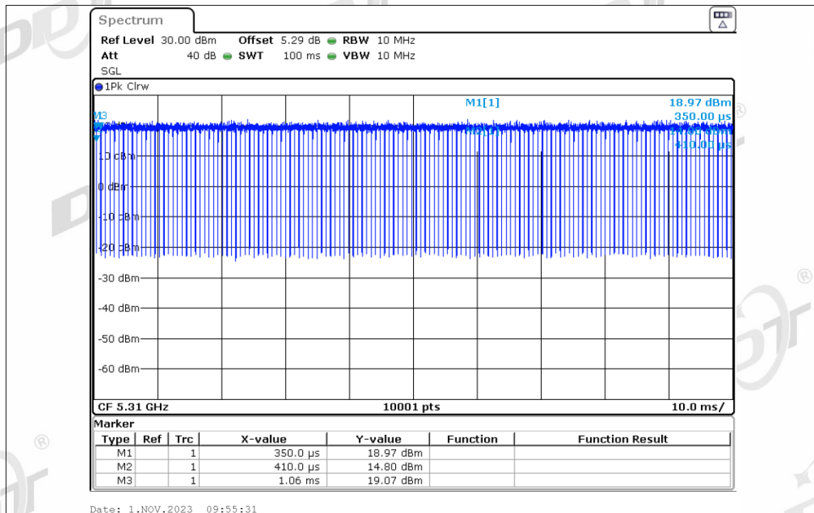
Duty Cycle NVNT n40 5510MHz Ant2
