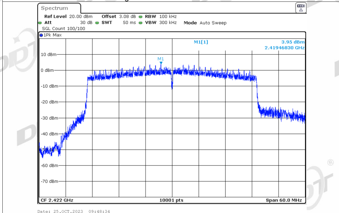
Band Edge NVNT ax40 2422MHz Ant2 Emission
