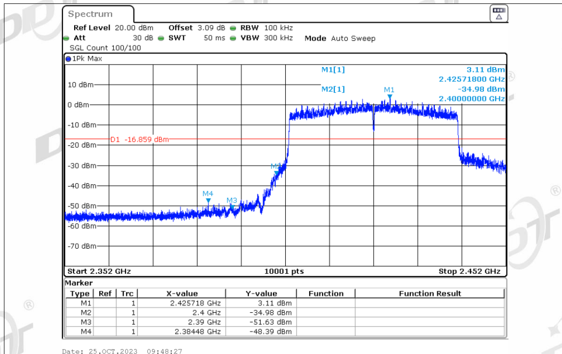
Band Edge NVNT ax40 2422MHz Ant2 Ref
