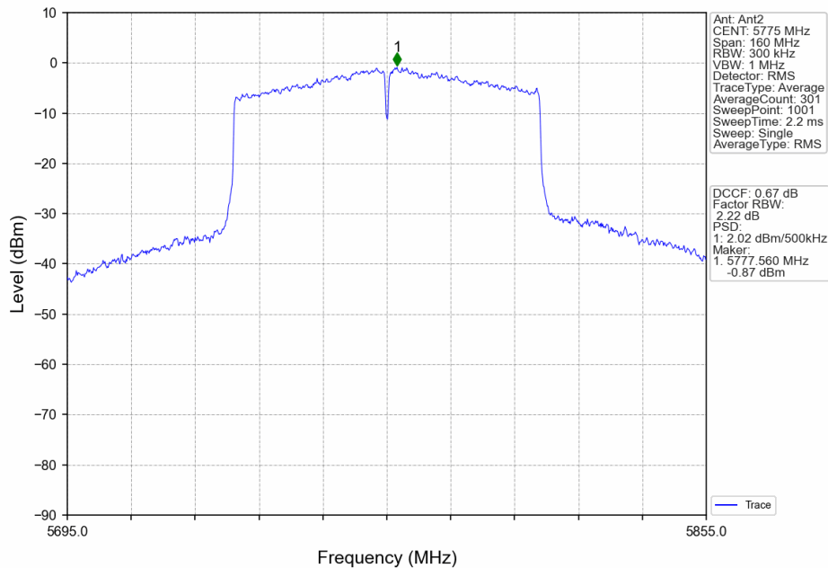
802.11ac(VHT80)_MCH_5775MHz_MIMO_NTNV
