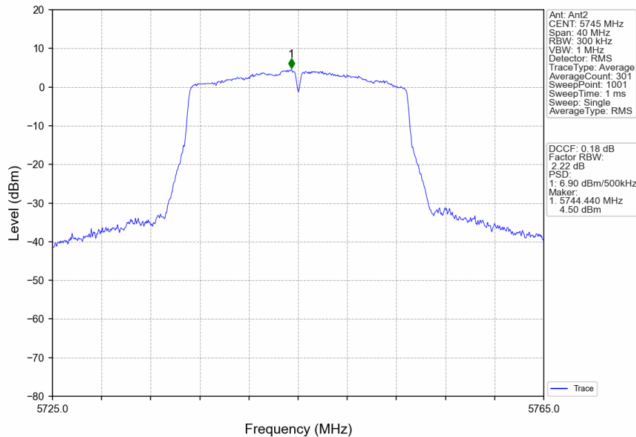
802.11n(HT20)_LCH_5745MHz_MIMO_NTNV
