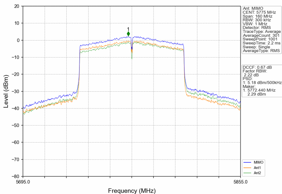
802.11ac(VHT80)_MCH_5775MHz_MIMO_NTNV
