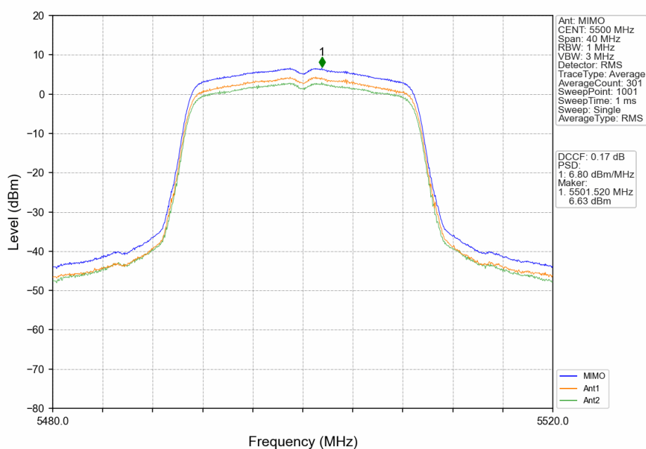
802.11ac(VHT20)_LCH_5500MHz_MIMO_NTNV
