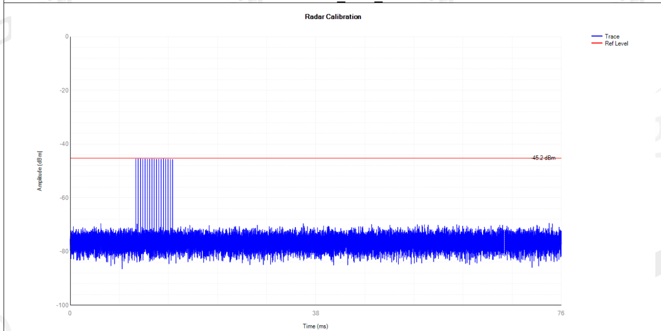
5260MHz DFS_FCC_T4000
