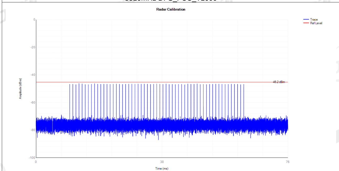
5510MHz DFS_FCC_T2000
