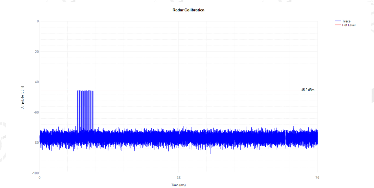
5260MHz DFS_FCC_T3000
