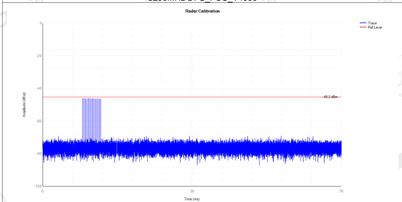
5290MHz DFS_FCC_T5000
