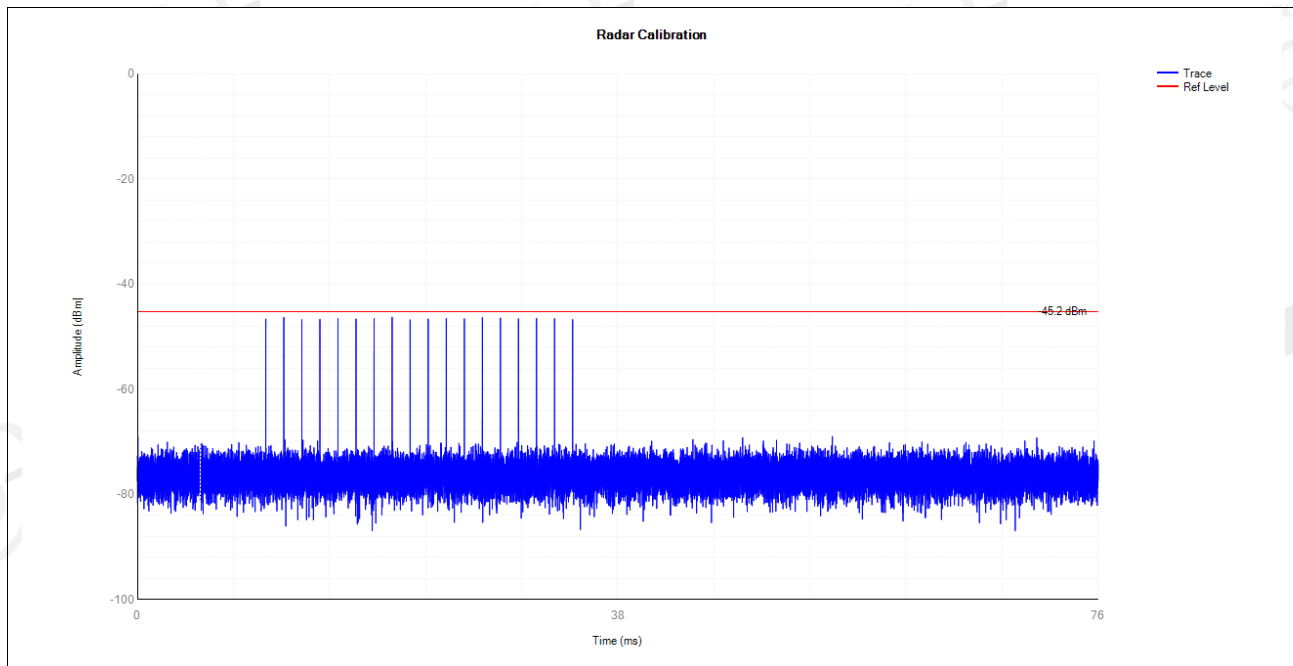
5510MHz DFS_FCC_T1000
