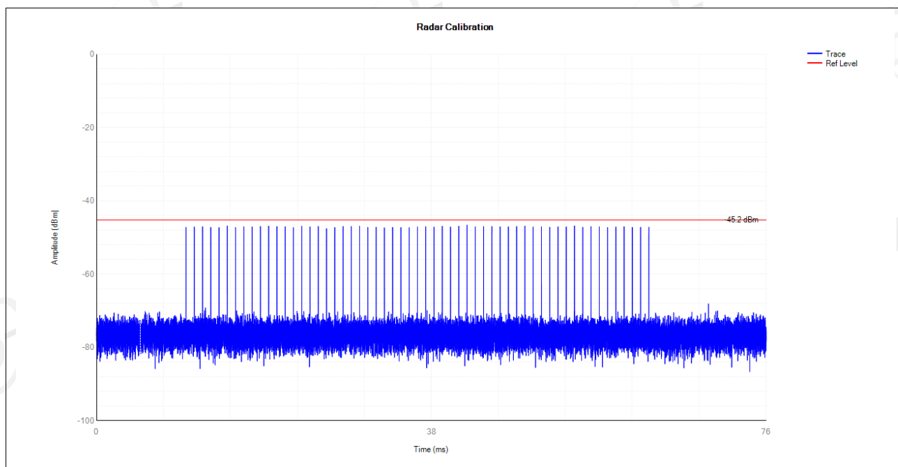
5290MHz DFS_FCC_T2000
