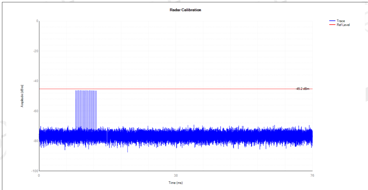
5290MHz DFS_FCC_T4000
