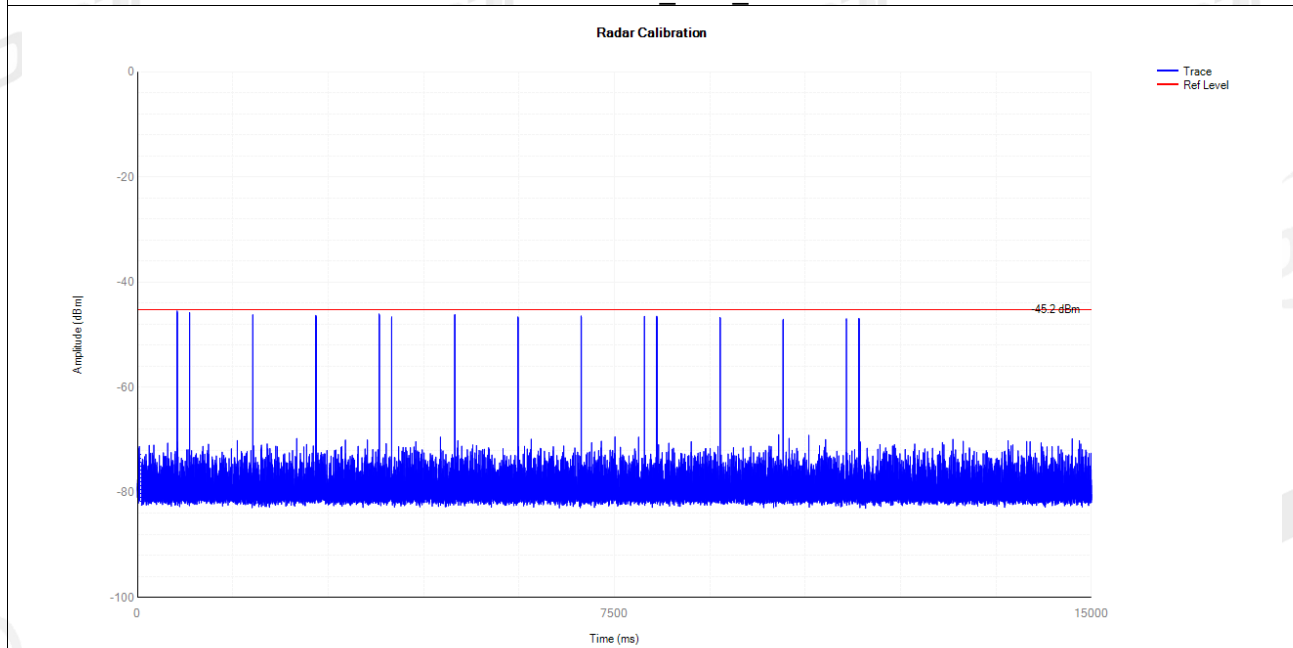
5510MHz DFS_FCC_T6000
