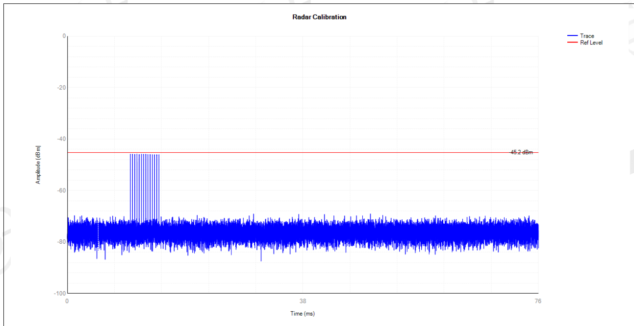
5510MHz DFS_FCC_T5000
