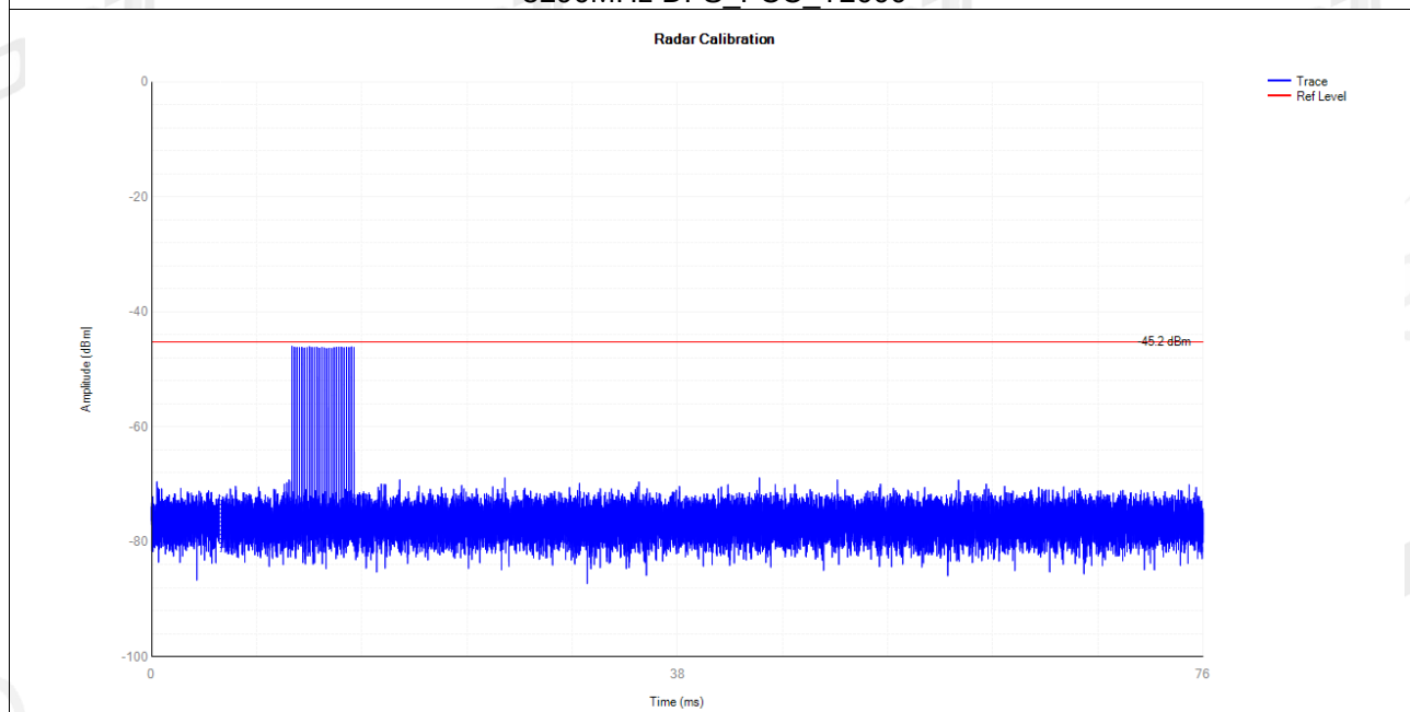
5290MHz DFS_FCC_T3000
