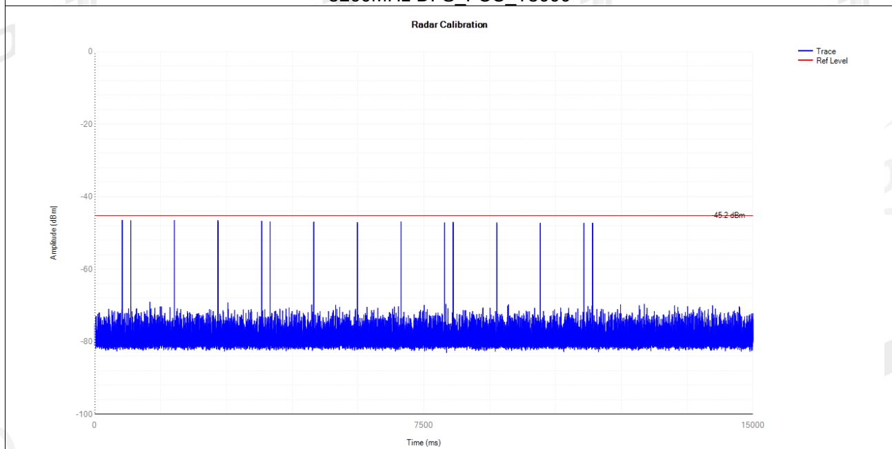
5260MHz DFS_FCC_T6000
