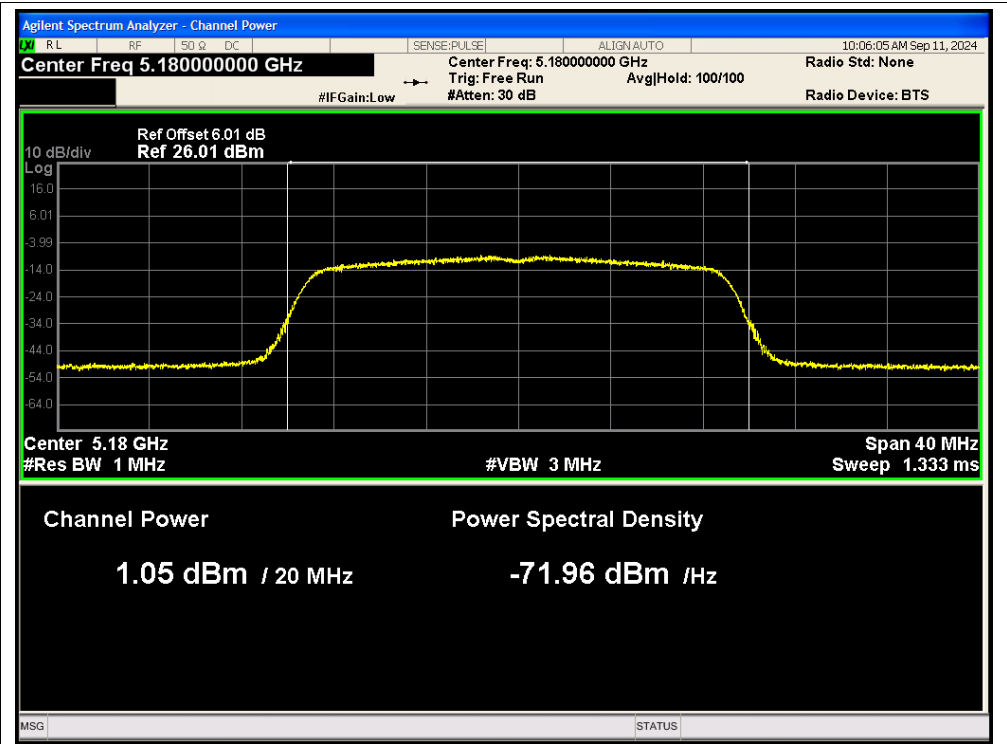
Power NVNT n20 5180MHz Ant2
