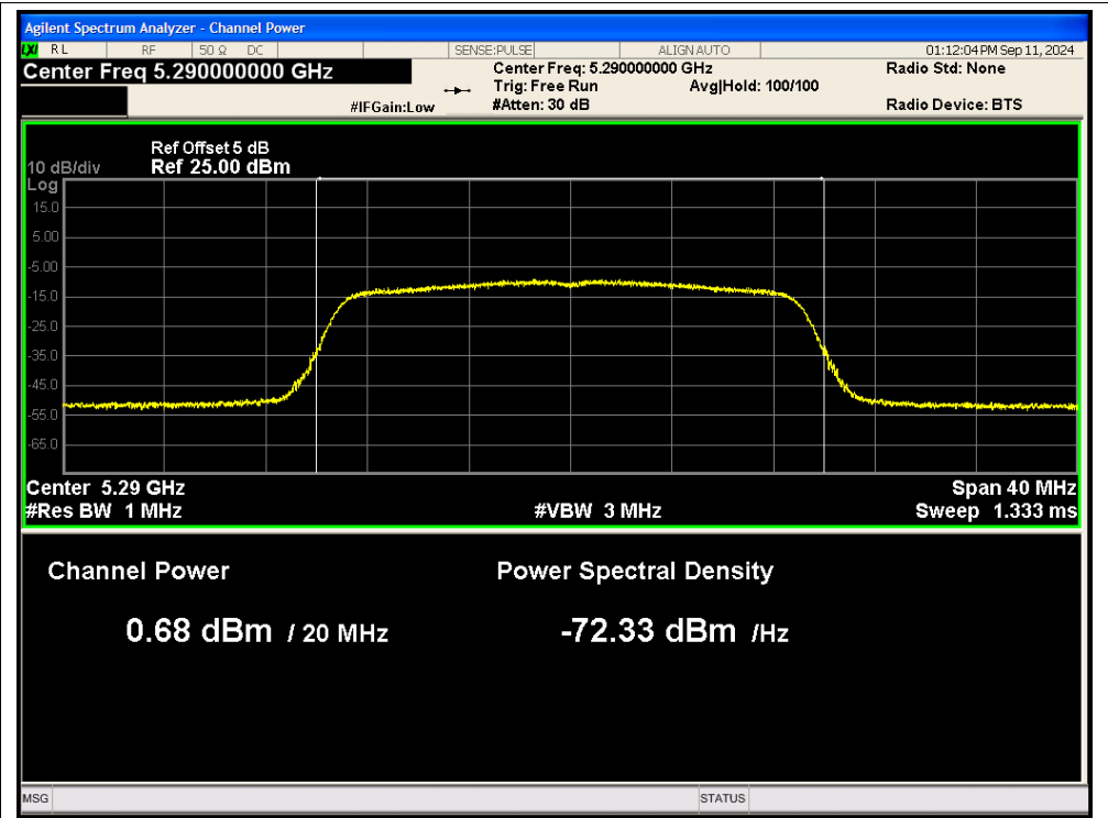
Power NVNT n20 5290MHz Ant2
