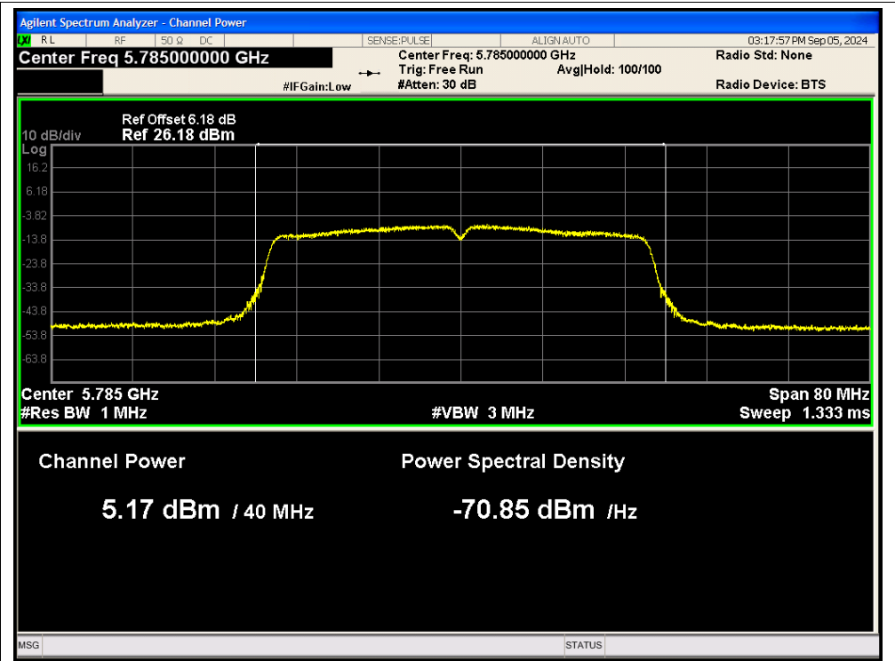
Power NVNT ac40 5785MHz Ant2
