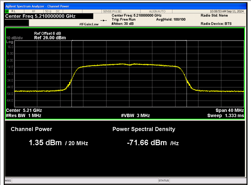
Power NVNT n20 5210MHz Ant2
