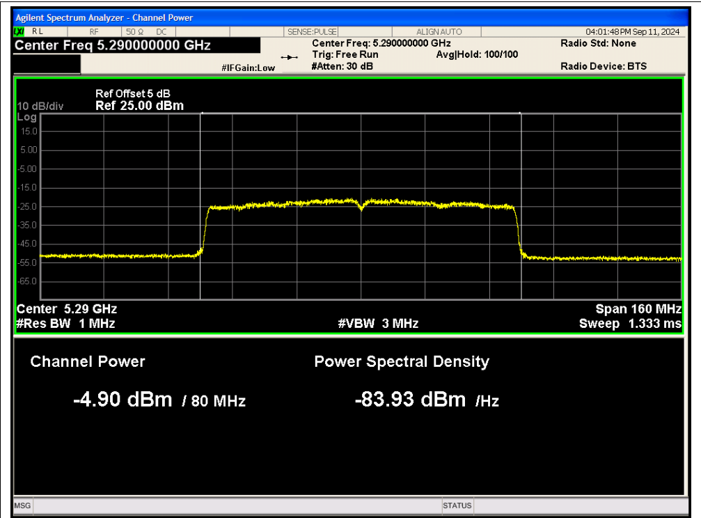
Power NVNT ac80 5290MHz Ant2
