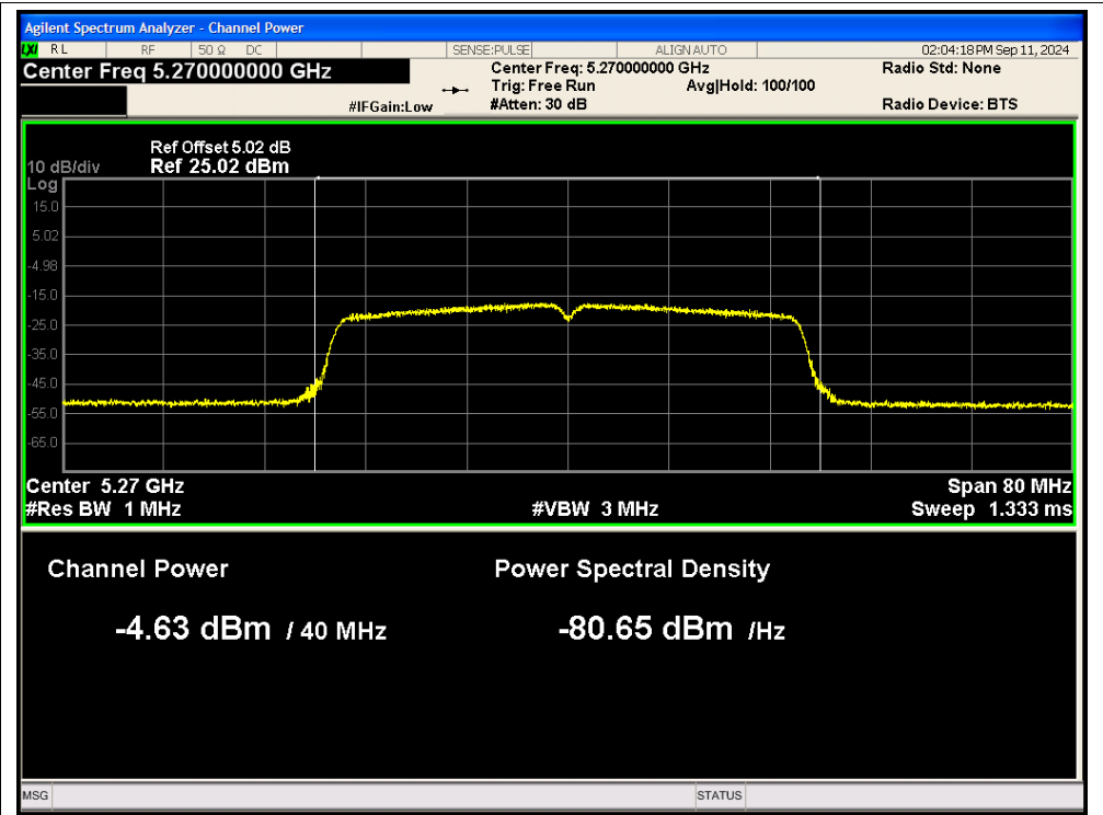
Power NVNT n40 5270MHz Ant2
