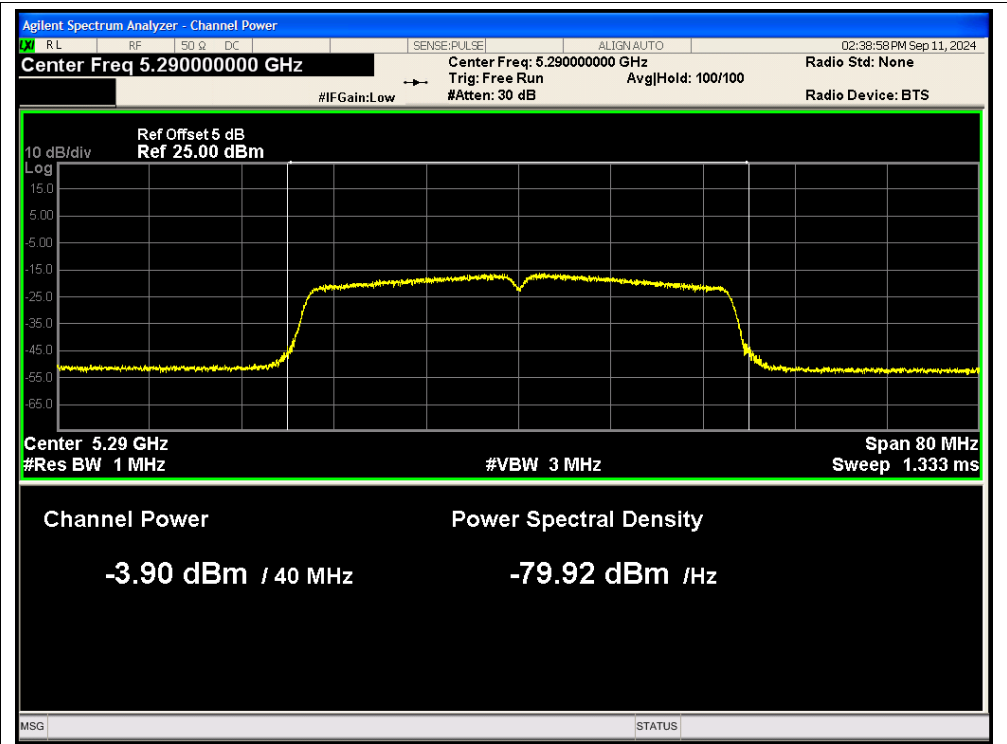
Power NVNT n40 5290MHz Ant2
