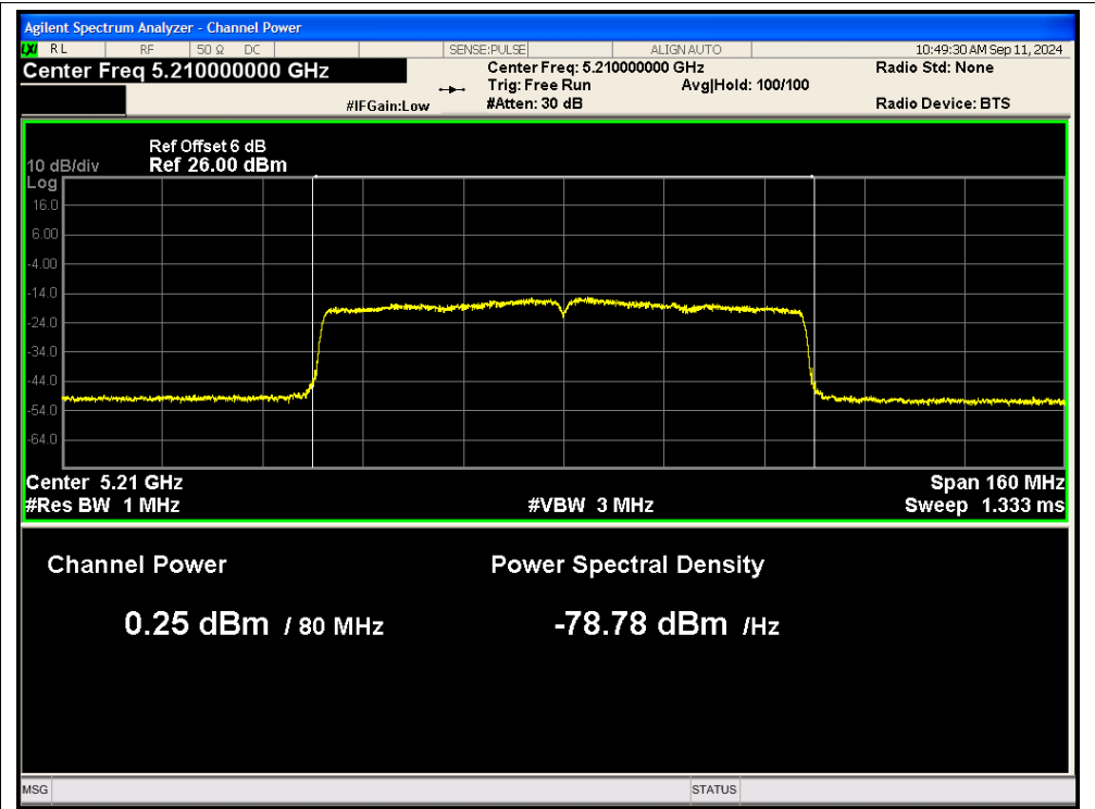
Power NVNT ac80 5210MHz Ant2
