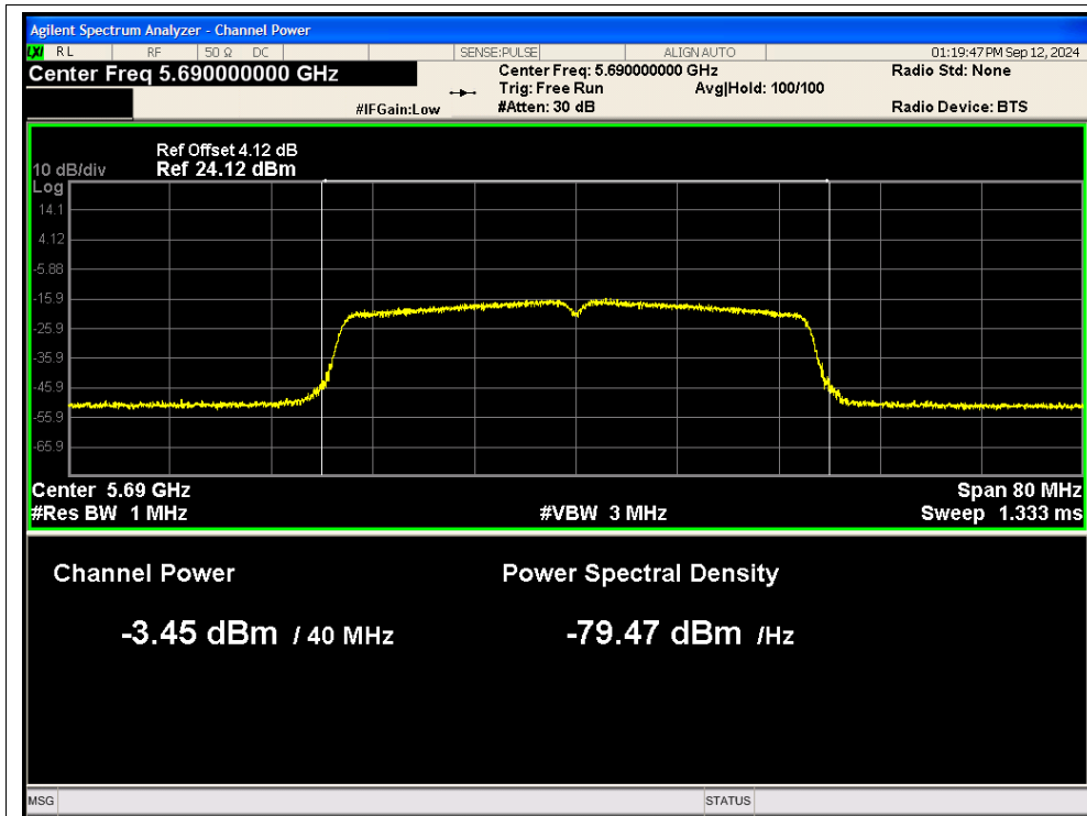
Power NVNT n40 5690MHz Ant2
