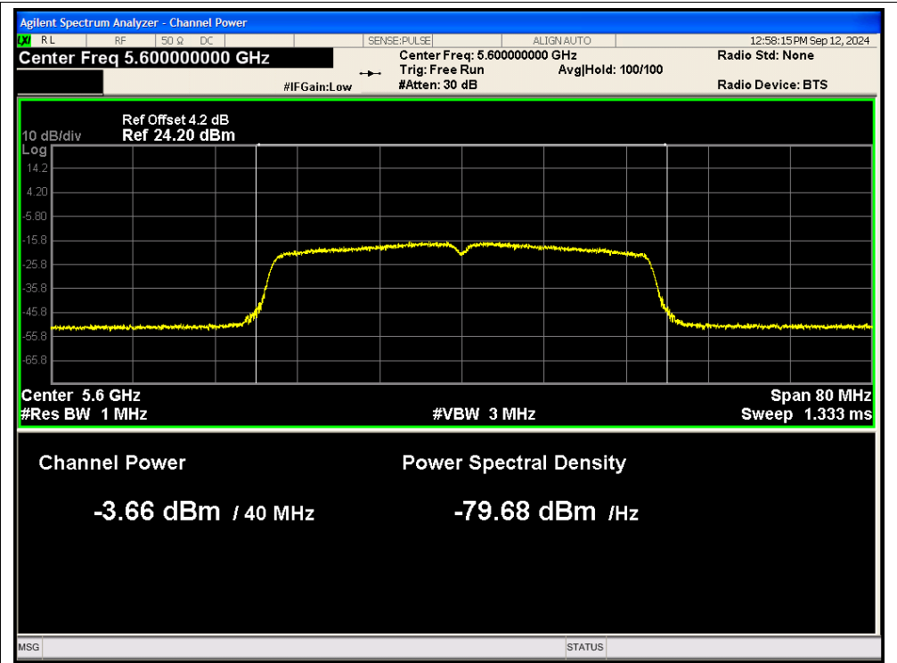
Power NVNT n40 5600MHz Ant2
