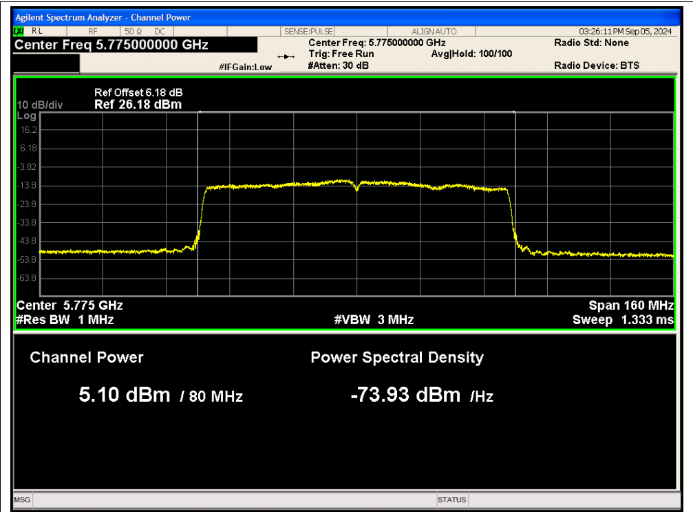
Power NVNT ac80 5775MHz Ant2
