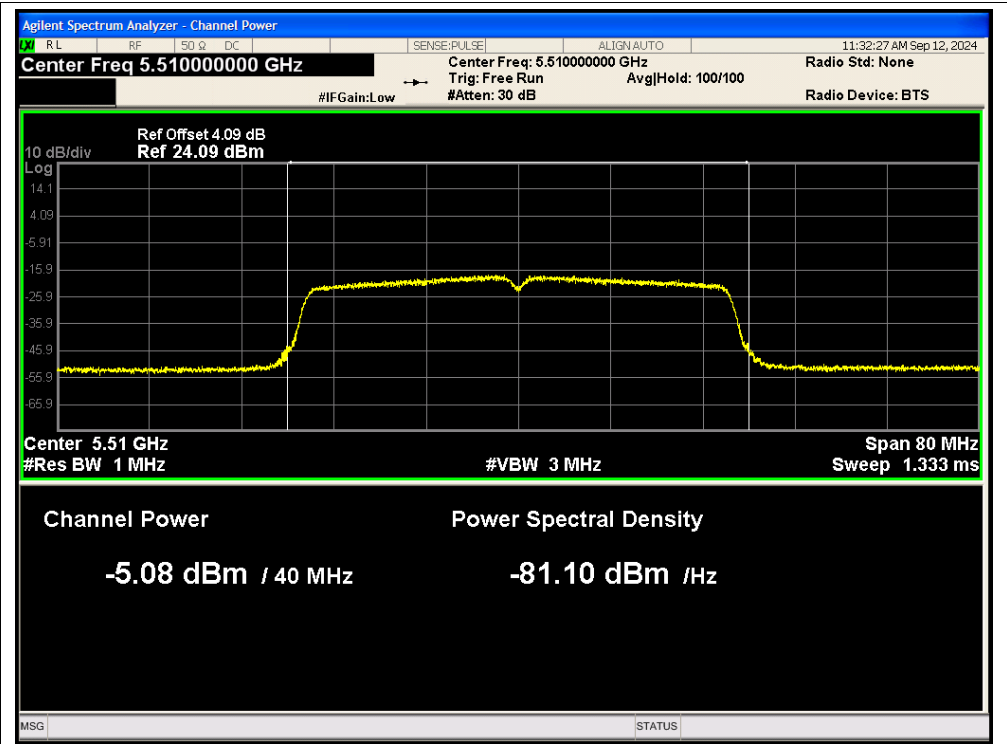
Power NVNT n40 5510MHz Ant2
