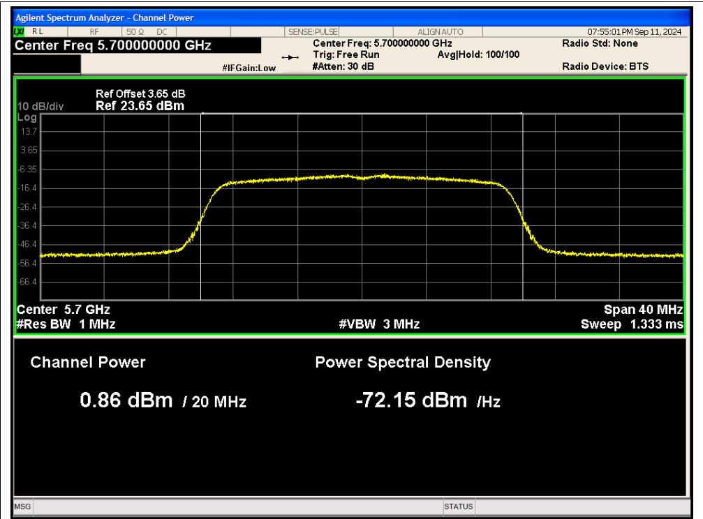
Power NVNT n20 5700MHz Ant2
