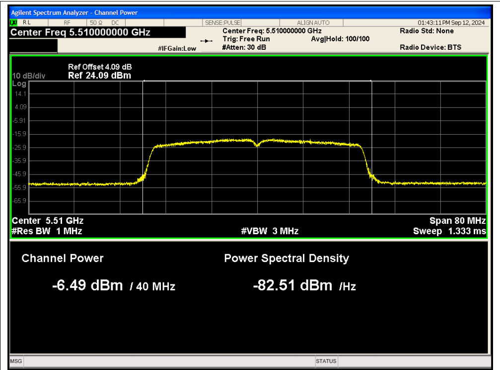
Power NVNT ac40 5510MHz Ant2
