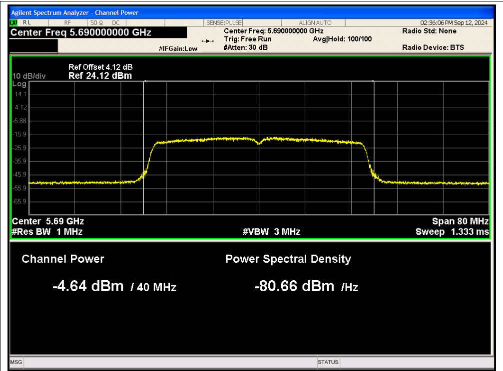
Power NVNT ac40 5690MHz Ant2
