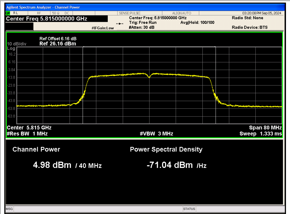
Power NVNT ac40 5815MHz Ant2
