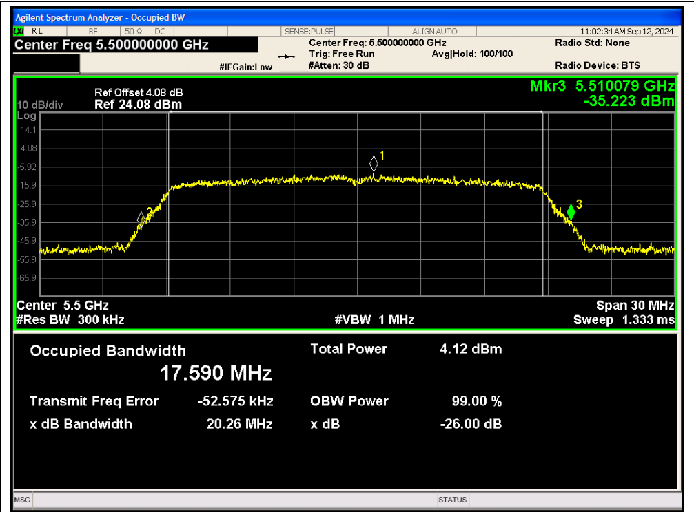
-26dB Bandwidth NVNT ac20 5500MHz Ant2
