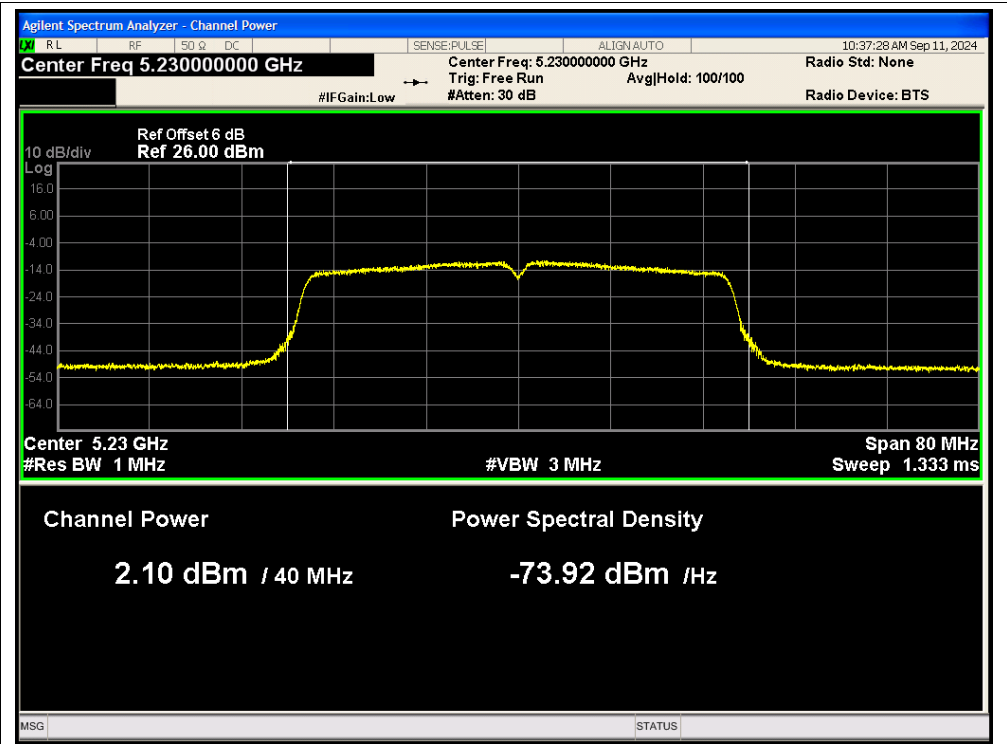
Power NVNT n40 5230MHz Ant2
