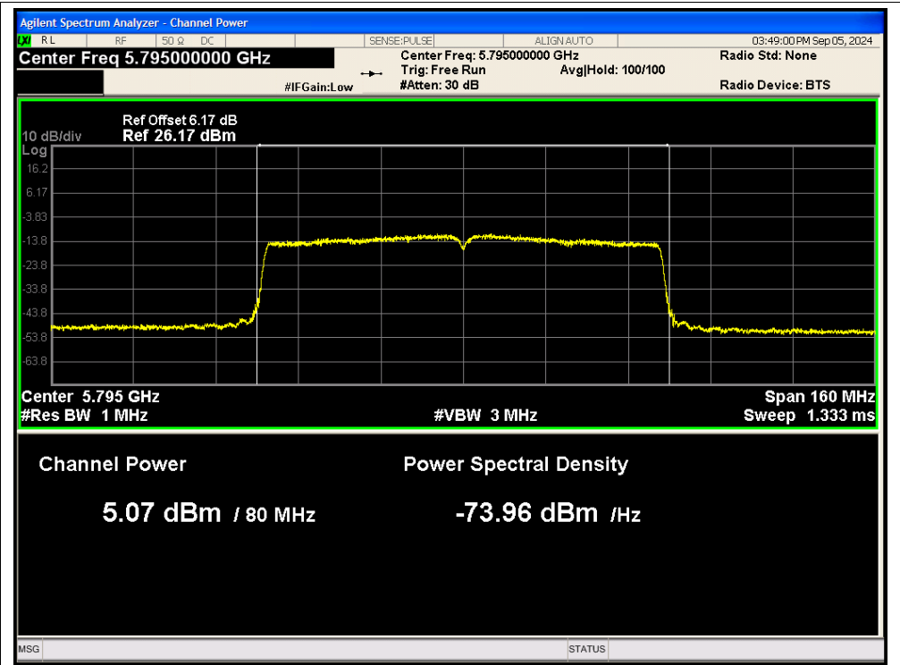
Power NVNT ac80 5795MHz Ant2
