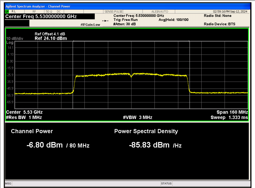
Power NVNT ac80 5530MHz Ant2
