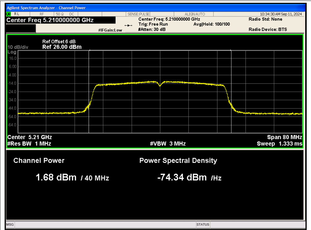
Power NVNT n40 5210MHz Ant2
