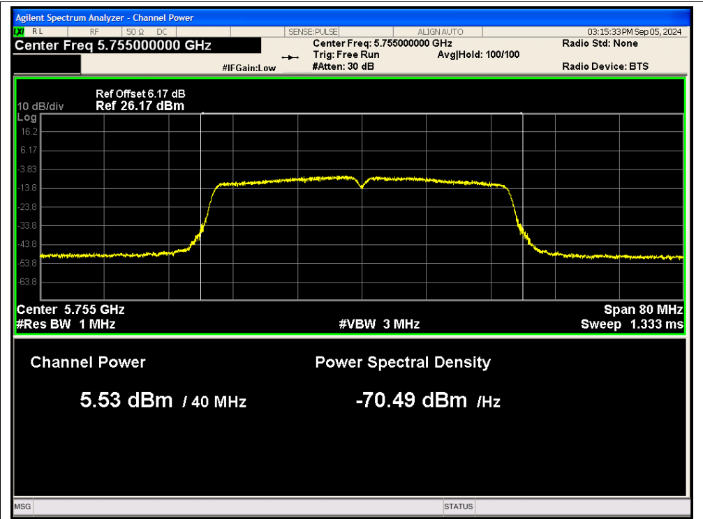
Power NVNT ac40 5755MHz Ant2
