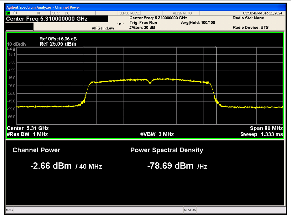
Power NVNT ac40 5310MHz Ant2
