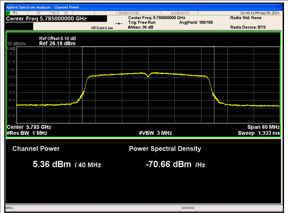
Power NVNT n40 5785MHz Ant2
