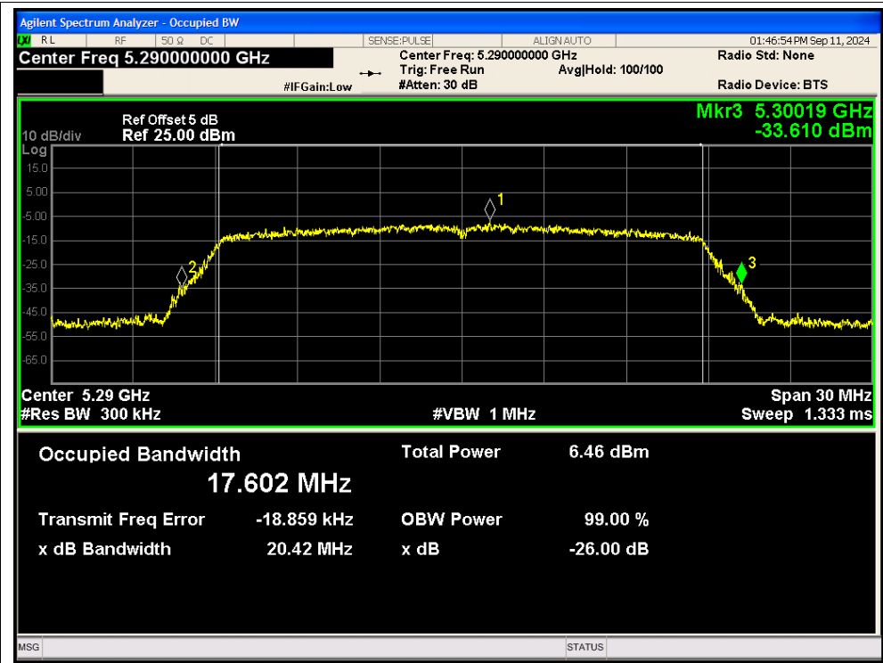
-26dB Bandwidth NVNT ac20 5290MHz Ant2
