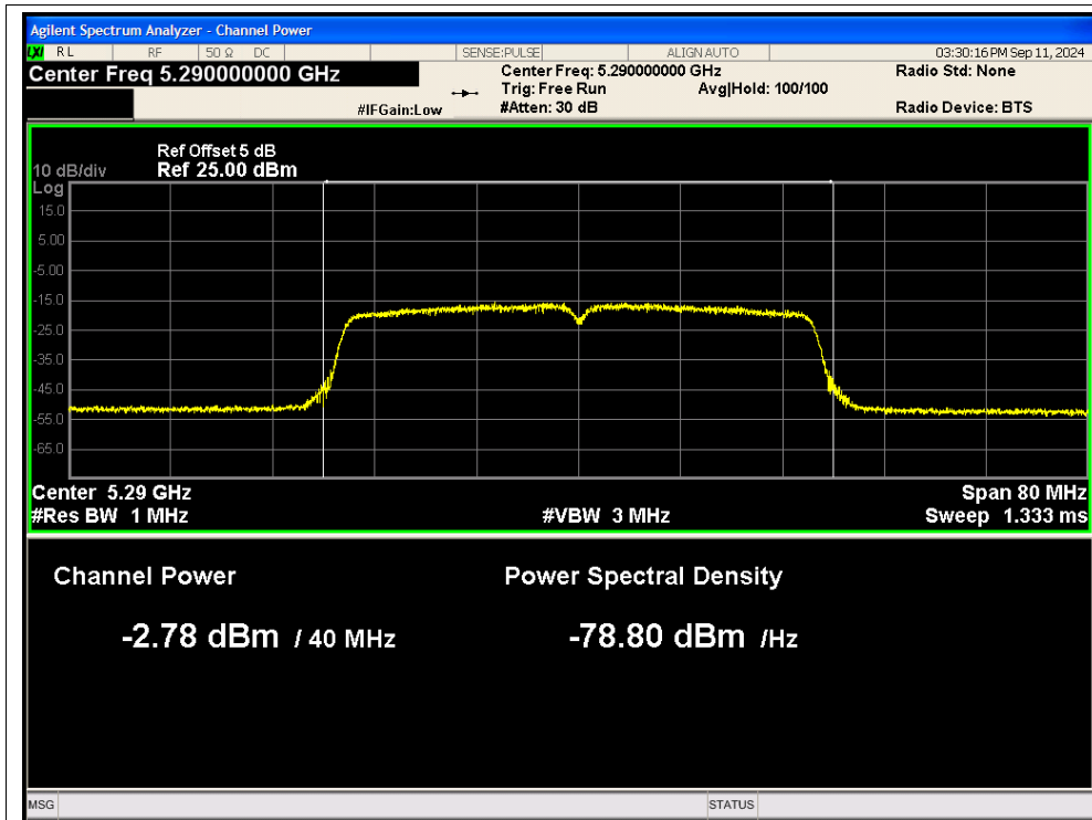
Power NVNT ac40 5290MHz Ant2
