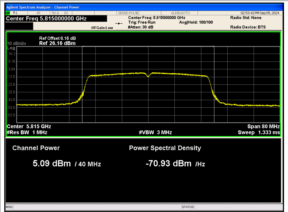
Power NVNT n40 5815MHz Ant2
