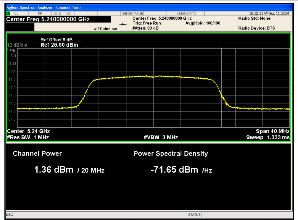
Power NVNT n20 5240MHz Ant2
