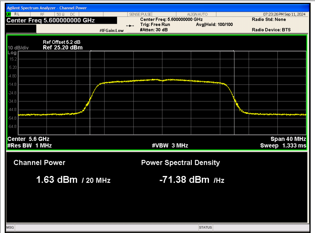
Power NVNT n20 5600MHz Ant2
