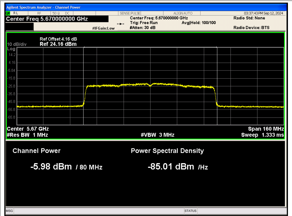
Power NVNT ac80 5670MHz Ant2
