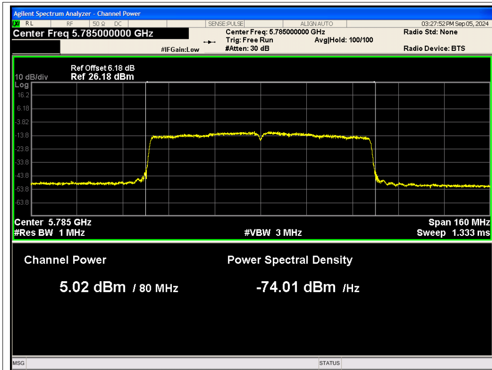
Power NVNT ac80 5785MHz Ant2
