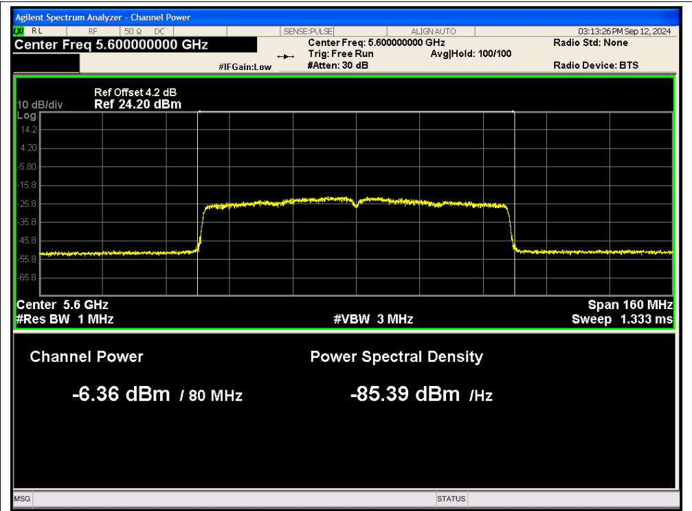
Power NVNT ac80 5600MHz Ant2
