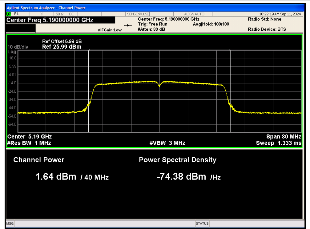
Power NVNT n40 5190MHz Ant2
