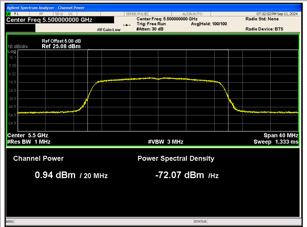
Power NVNT n20 5500MHz Ant2
