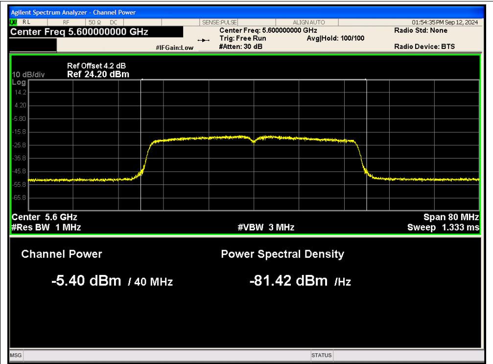
Power NVNT ac40 5600MHz Ant2
