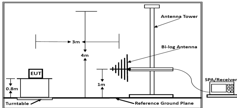
Below 1GHz
