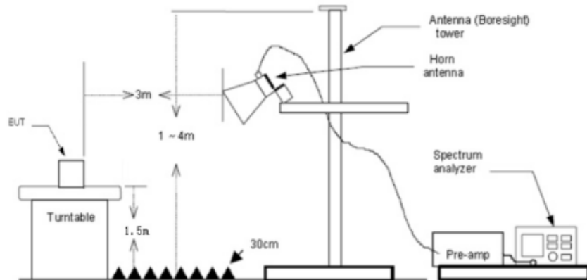
Above 1GHz
