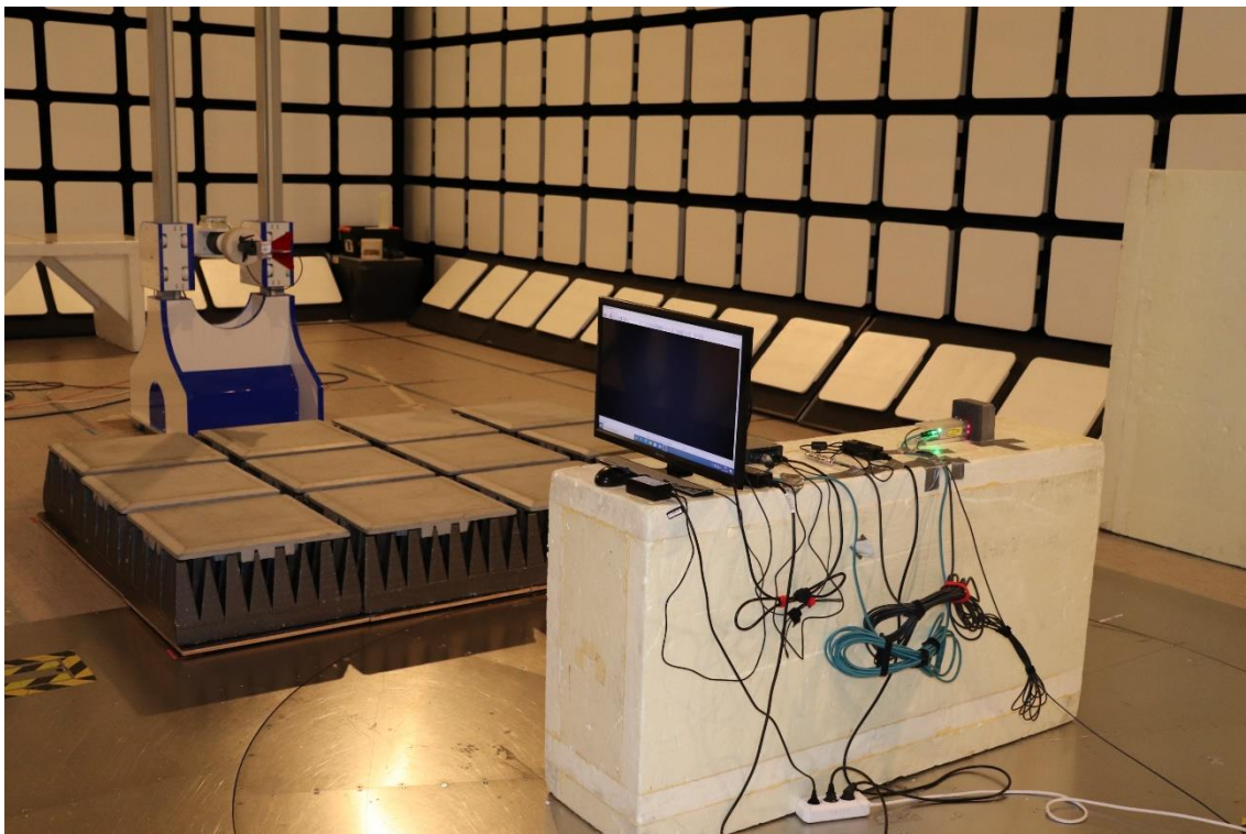
Photograph 5: Radiated emissions (1-5 GHz) test setup
