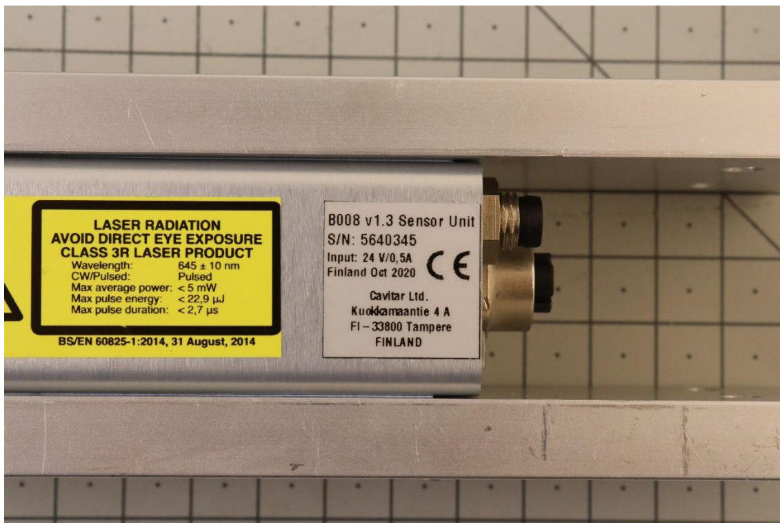
Photograph 3: Type label of the EUT
