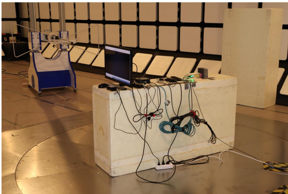
Photograph 4: Radiated emissions (30-1000 MHz) test setup
