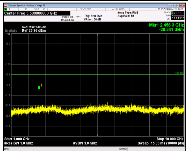
Band26-1.4MHz-16QAM-26783-1RB#0-Range2:1000 ~10000MHz
