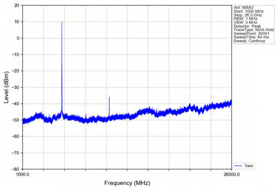
802.11ac(VHT20)_MCH_5785MHz_MIMO_NTNV
