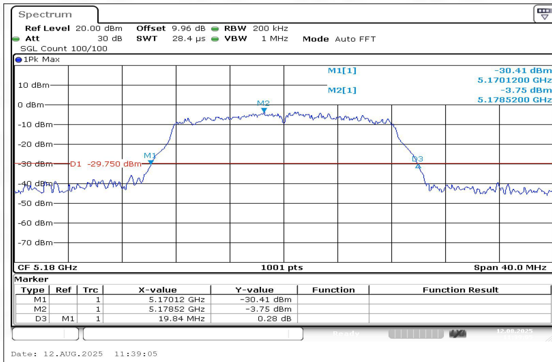
11A-Ant1-5180
