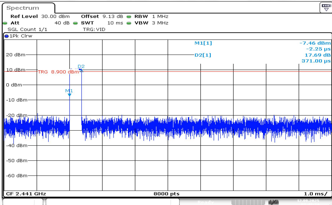
DH1-Ant1-Hop-PASS
