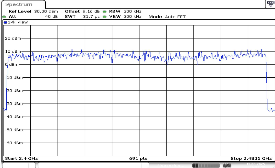
DH5-Ant1-Hop-PASS
