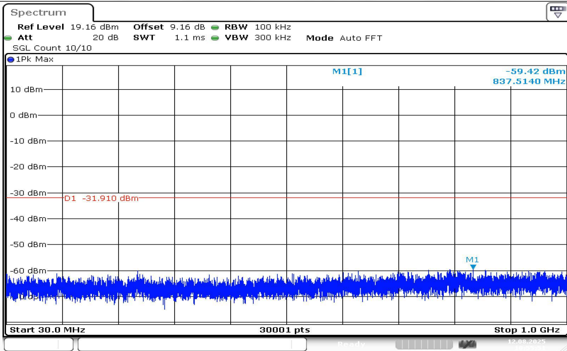
11B-Ant1-2412-30~1000-PASS
