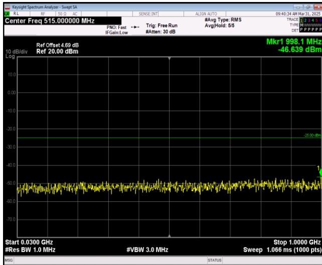
Band7-20MHz-16QAM-20850-1RB#0-Range1:30~10 00MHz
