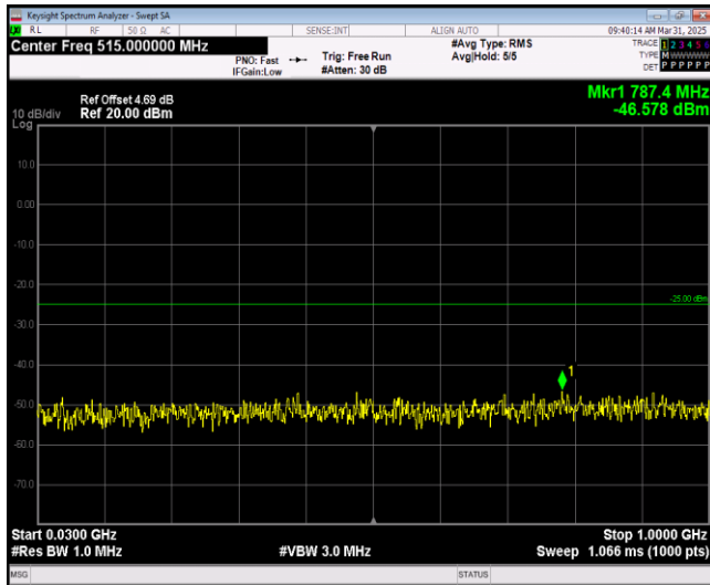
Band7-20MHz-64QAM-21350-1RB#0-Range1:30~1000MHz
