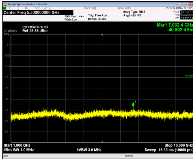
Band5-10MHz-64QAM-20450-1RB#0-Range2:1000~10000MHz
