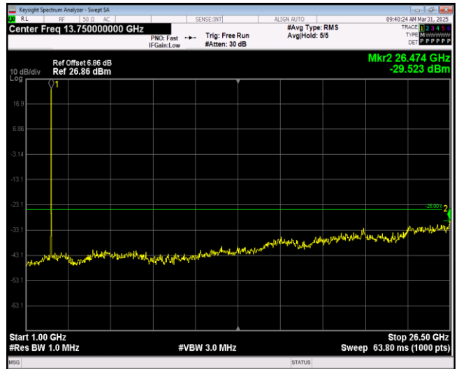
Band7-20MHz-64QAM-21350-1RB#0-Range2:1000~26500MHz
