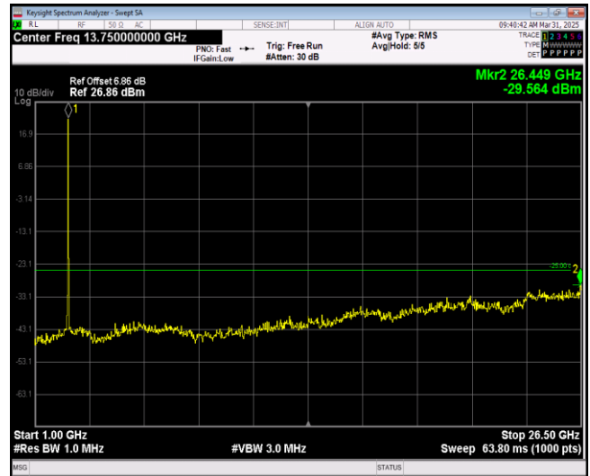
Band7-20MHz-16QAM-20850-1RB#0-Range2:1000~ 26500MHz
