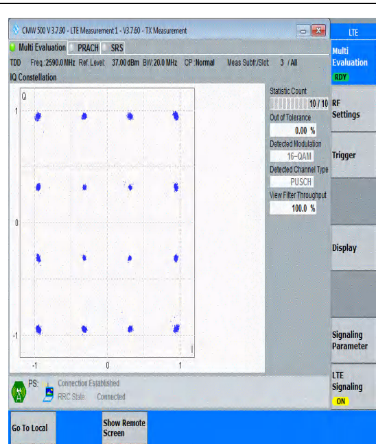
Band41(2535-2655)-20MHz-16QAM-40590-100RB #0-PASS
