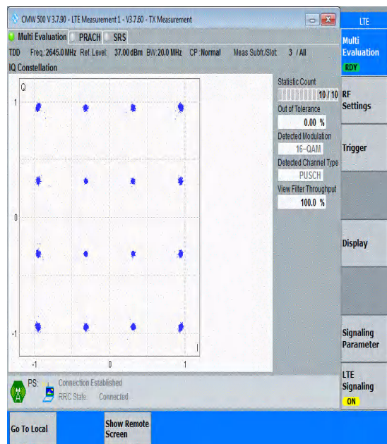
Band41(2535-2655)-20MHz-16QAM-41140-100RB #0-PASS
